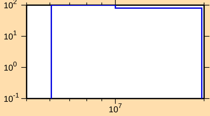
\Delta\sigma/\sigma vs. E for ^{191}\text{Tl}(n,2n)
