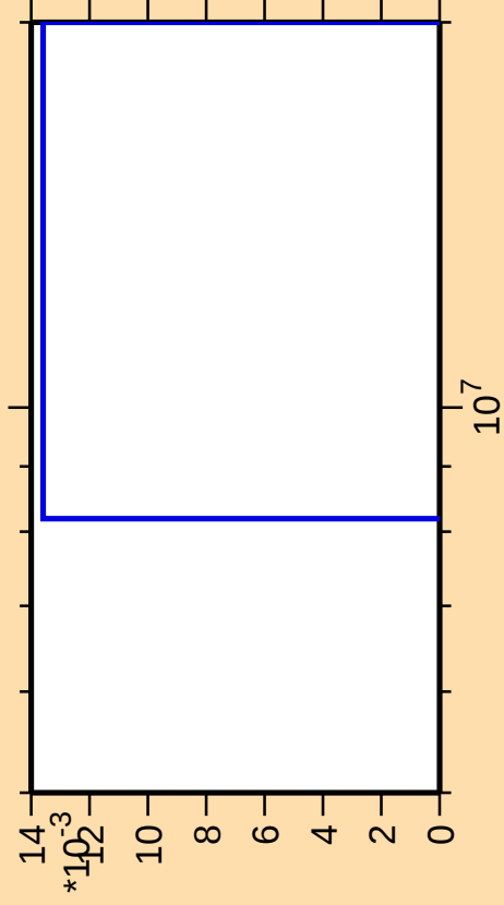
\Delta\sigma/\sigma vs. E for ^{191}\text{Tl}(\text{mt } 34)
