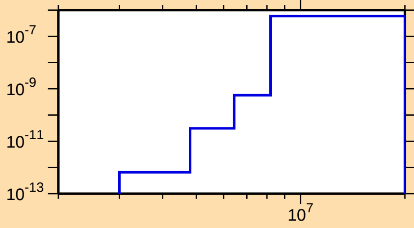
\sigma vs. E for ^{191}\text{Tl}(n,p\alpha)
