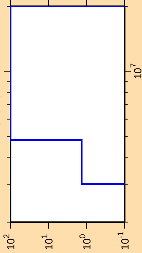
\Delta\sigma/\sigma vs. E for ^{191}\text{Tl}(n,p\alpha)
