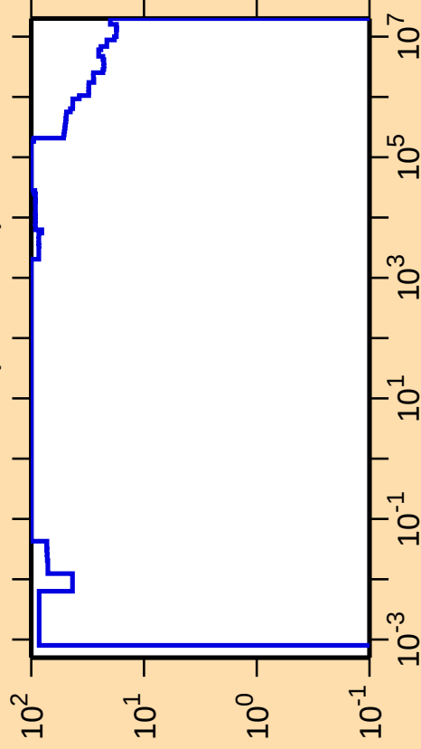
\Delta\sigma/\sigma vs. E for ^{192}\text{Tl}(n,\text{nonel.})
