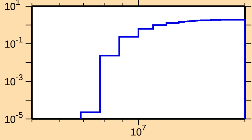
\sigma vs. E for ^{192}\text{Tl}(n,2n)
