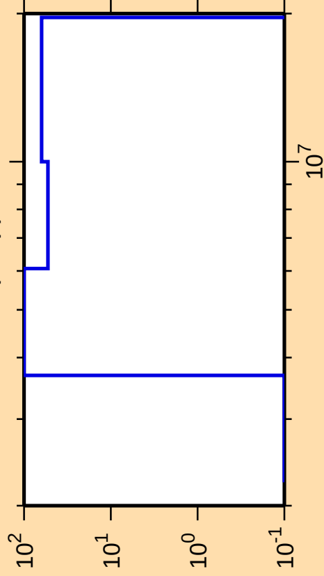
\Delta\sigma/\sigma vs. E for ^{192}\text{Tl}(n,np)
