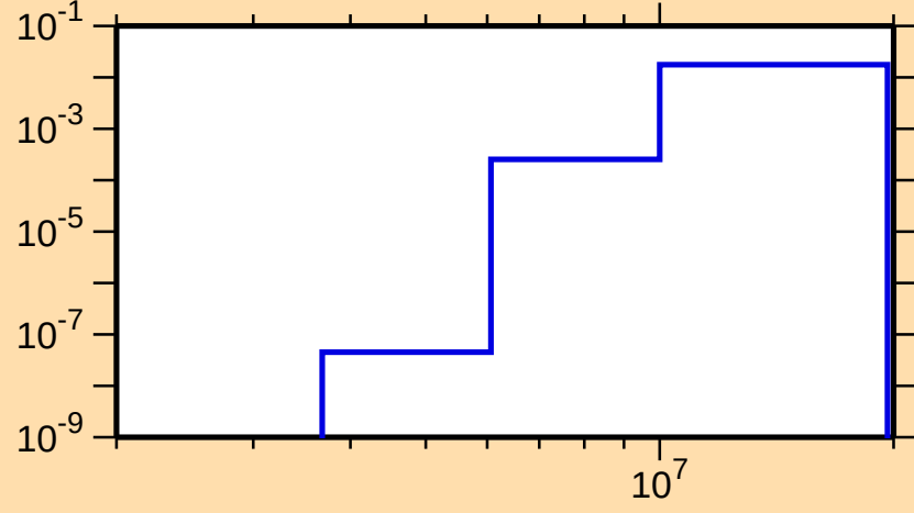
\sigma vs. E for ^{192}\text{Tl}(n,np)
