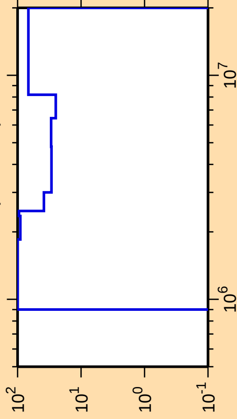
\Delta\sigma/\sigma vs. E for ^{192}\text{Tl}(n,n\text{cont.})
