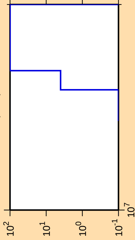
\Delta\sigma/\sigma vs. E for ^{192}\text{Tl}(n,\text{nt})
