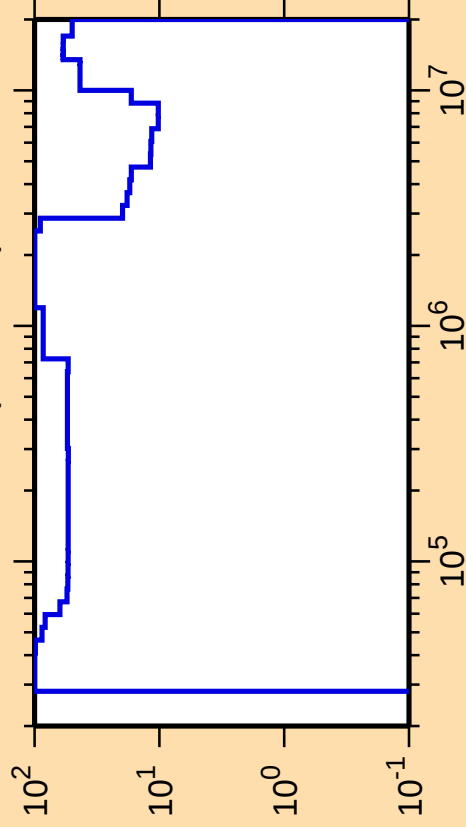
\Delta\sigma/\sigma vs. E for ^{192}\text{Tl}(n,\text{ncont.})
