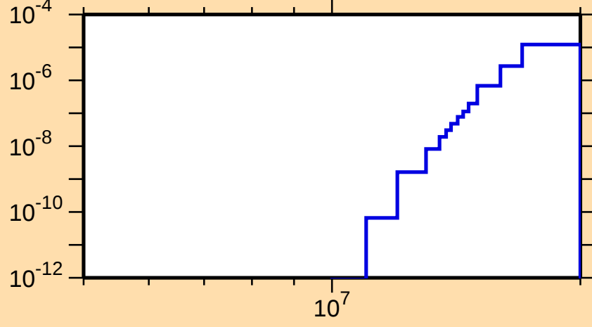
\sigma vs. E for ^{192}\text{Tl}(n,2n\alpha)
