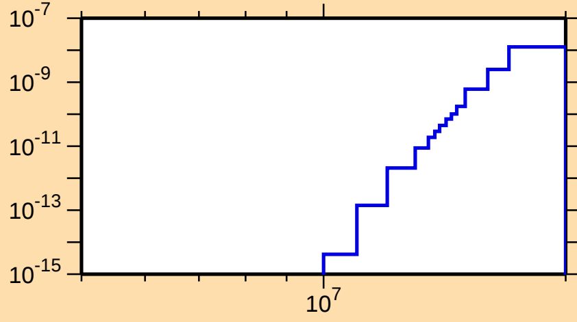
\sigma vs. E for ^{192}\text{Tl}(\text{mt } 45)
