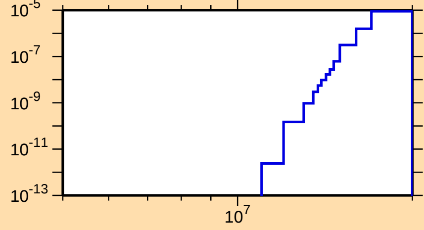
\sigma vs. E for ^{192}\text{Tl}(n,\text{nd})
