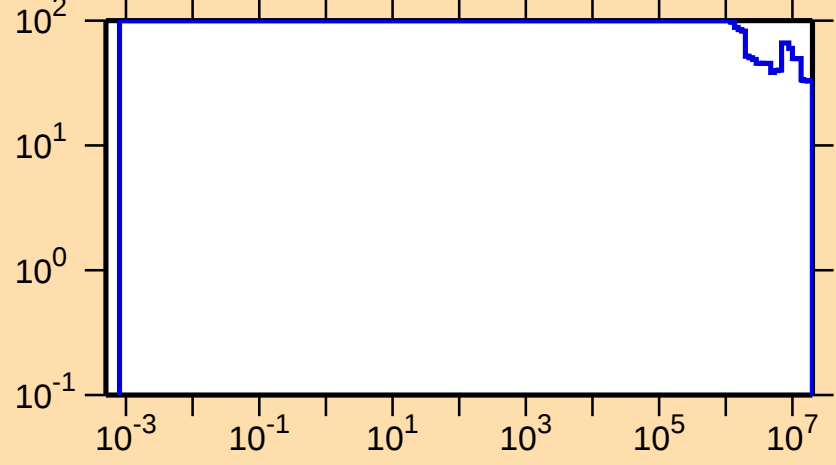
\Delta\sigma/\sigma vs. E for ^{192}\text{Tl}(n,p)
