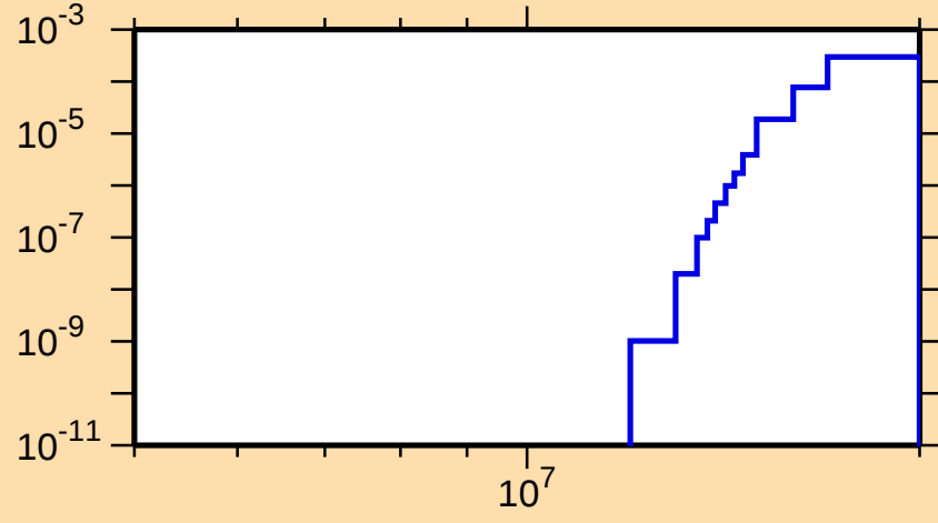
\sigma vs. E for ^{192}\text{Tl}(n,2np)
