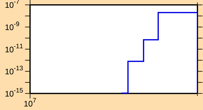
\sigma vs. E for ^{192}\text{Tl}(n,\text{nt})
