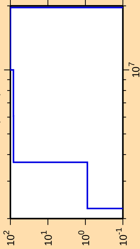
\Delta\sigma/\sigma vs. E for ^{192}\text{Tl}(n,n\alpha)
