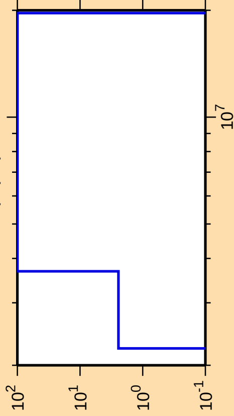
\Delta\sigma/\sigma vs. E for ^{192}\text{Tl}(n,p\alpha)
