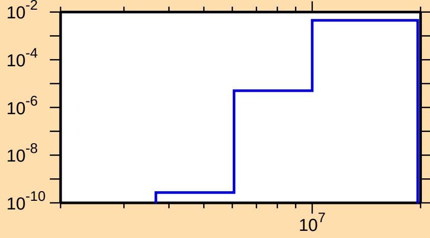
\sigma vs. E for ^{192}\text{Tl}(n,d)
