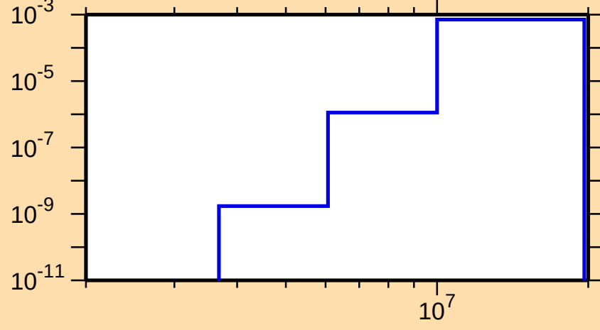
\sigma vs. E for ^{192}\text{Tl}(n,n\alpha)
