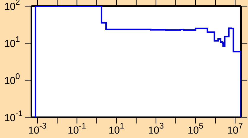
\Delta\sigma/\sigma vs. E for ^{192}\text{Tl}(n,\text{el.})
