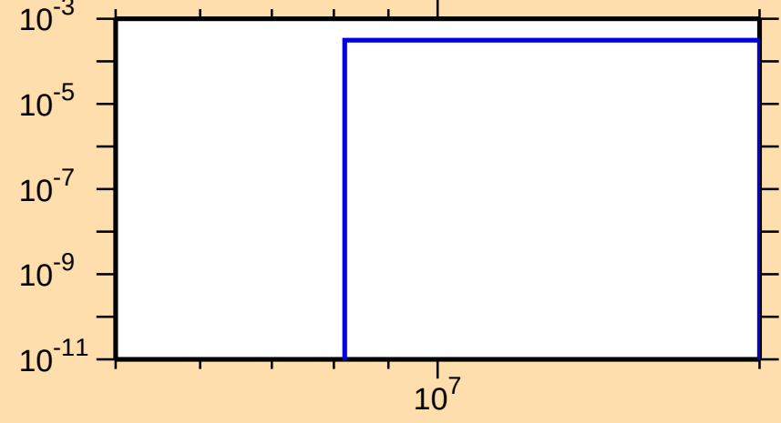
\sigma vs. E for ^{192}\text{Tl}(n,t)
