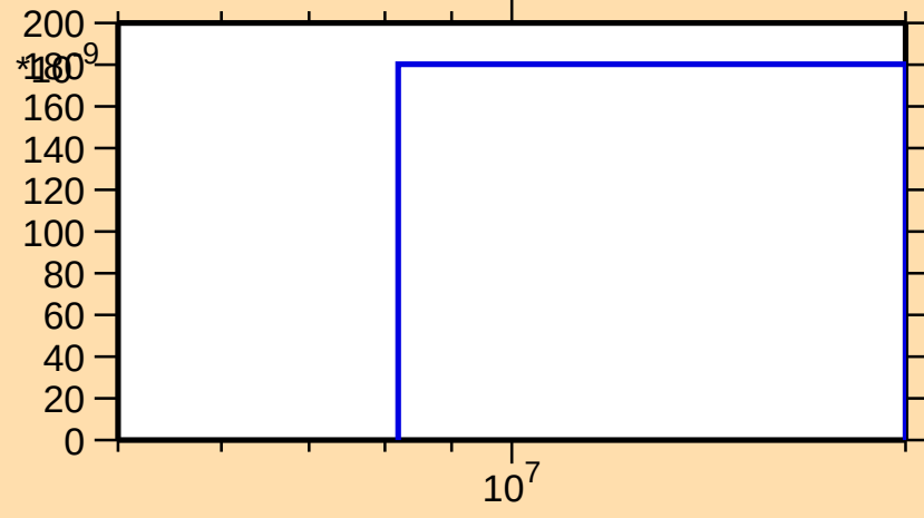
\sigma vs. E for ^{192}\text{Tl}(n,\text{nd})
