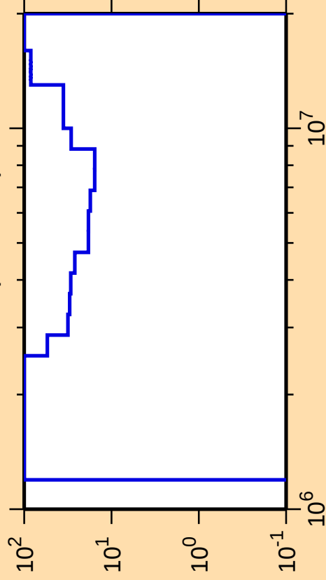
\Delta\sigma/\sigma vs. E for ^{193}\text{Tl}(n,n_{\text{cont}})
