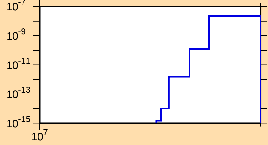
\sigma vs. E for ^{193}\text{Tl}(n,\text{nt})
