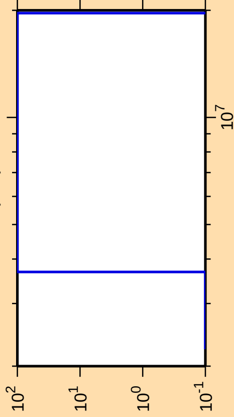
\Delta\sigma/\sigma vs. E for ^{193}\text{Tl}(n,d)
