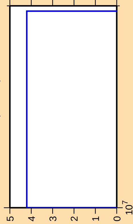
\Delta\sigma/\sigma vs. E for ^{193}\text{Tl}(\text{mt117})
