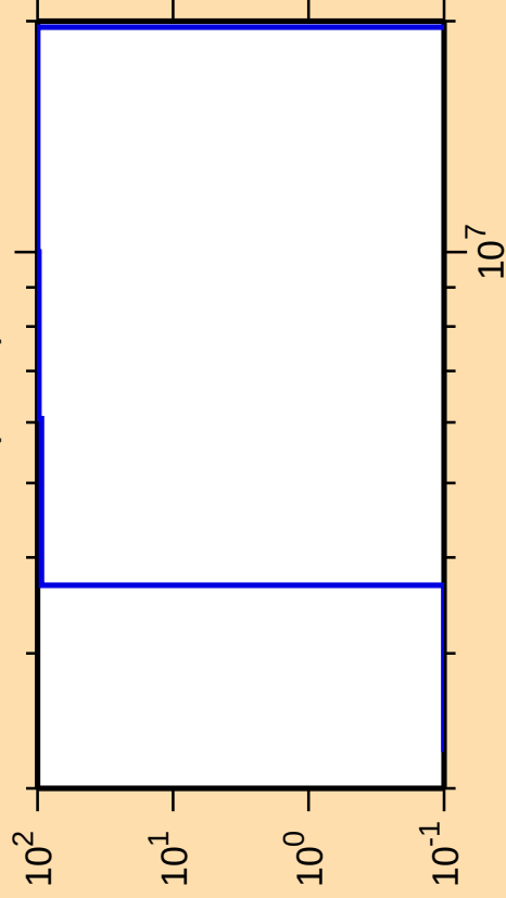
\Delta\sigma/\sigma vs. E for ^{193}\text{Tl}(n,n\alpha)
