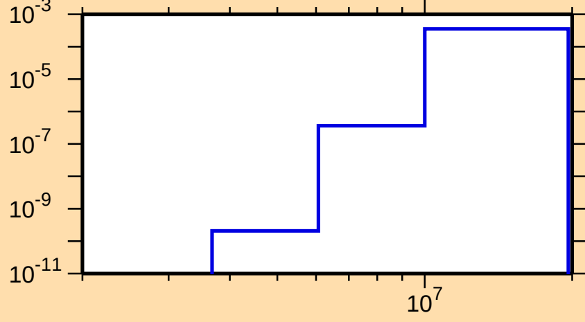
\sigma vs. E for ^{193}\text{Tl}(n,n\alpha)
