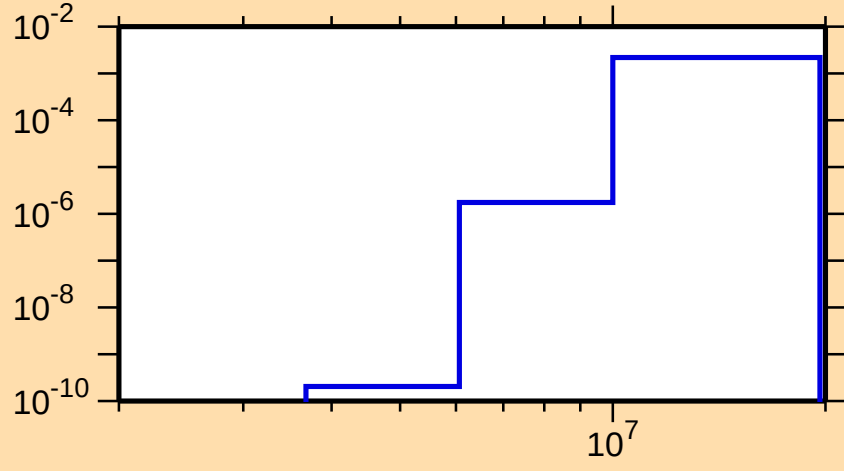
\sigma vs. E for ^{193}\text{Tl}(n,d)
