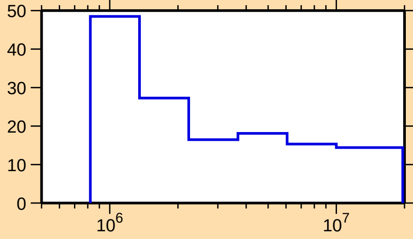
\Delta\sigma/\sigma vs. E for ^{193}\text{Tl}(n,n\text{nonel.})
