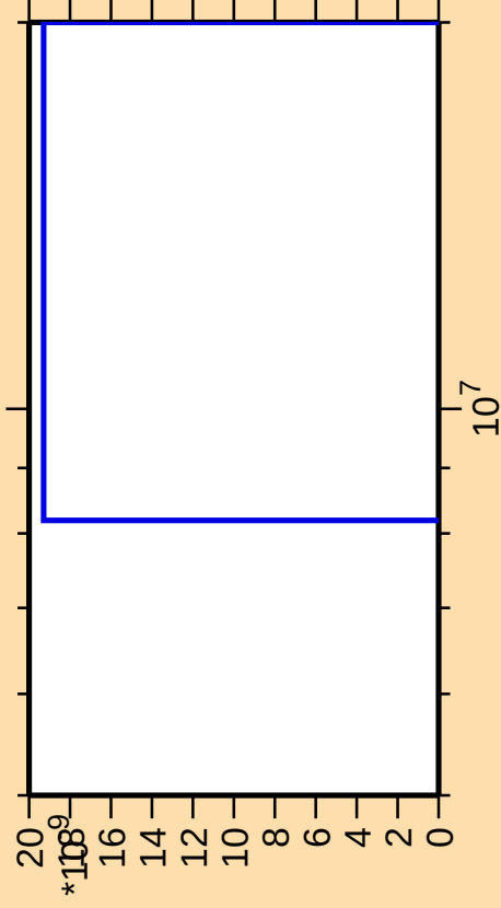
\Delta\sigma/\sigma vs. E for ^{193}\text{Tl}(\text{mt } 42)
