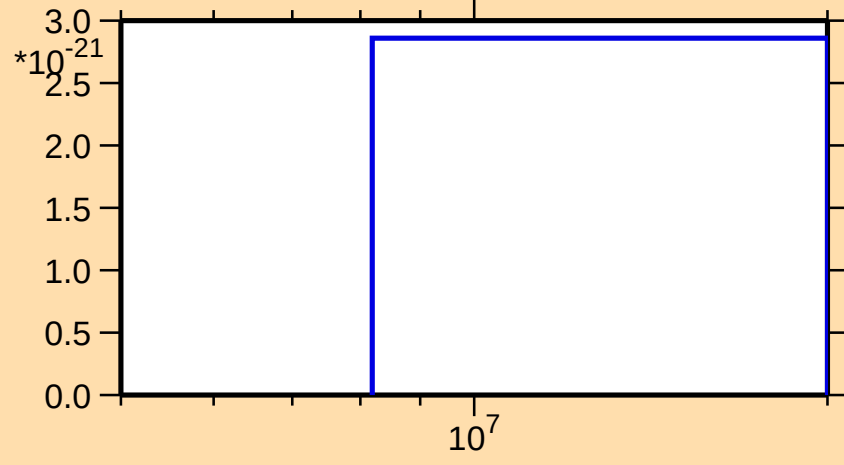
\sigma vs. E for ^{193}\text{Tl}(\text{mt } 42)
