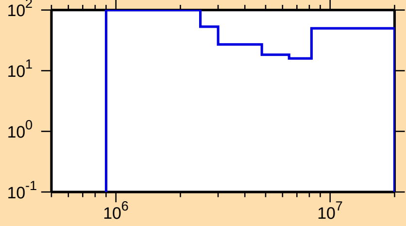
\Delta\sigma/\sigma vs. E for ^{193}\text{Tl}(n,ncont.)
