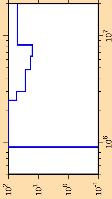
\Delta\sigma/\sigma vs. E for ^{193}\text{Tl}(n,\text{ncont.})
