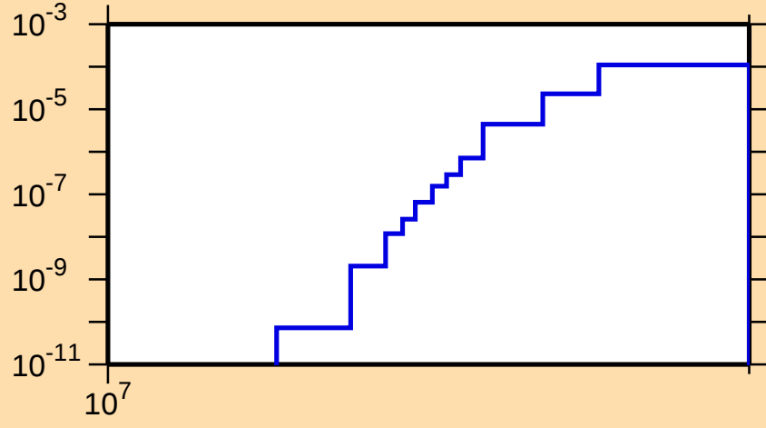
\sigma vs. E for ^{194}\text{Tl}(n,2np)
