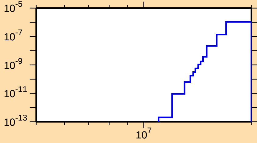
\sigma vs. E for ^{194}\text{Tl}(n,2n\alpha)
