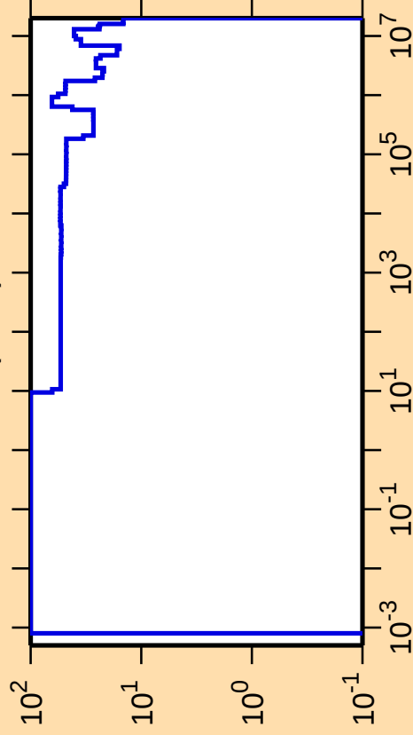
\Delta\sigma/\sigma vs. E for ^{194}\text{Tl}(n,\text{el.})
