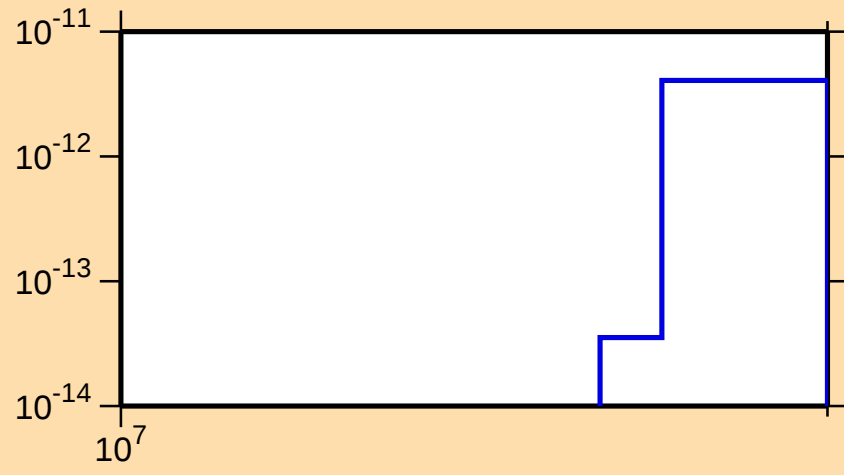
\sigma vs. E for ^{194}\text{Tl}(\text{mt 34})
