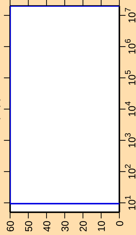
\Delta\sigma/\sigma vs. E for ^{194}\text{Tl}(n,p)
