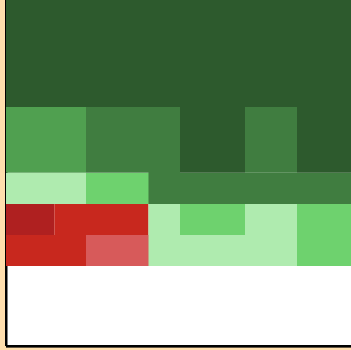
\Delta\sigma/\sigma vs. E for ^{194}\text{Tl}(n,\text{nonel.})
