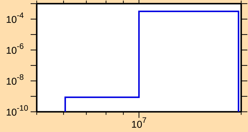
\sigma vs. E for ^{194}\text{Tl}(n,t)
