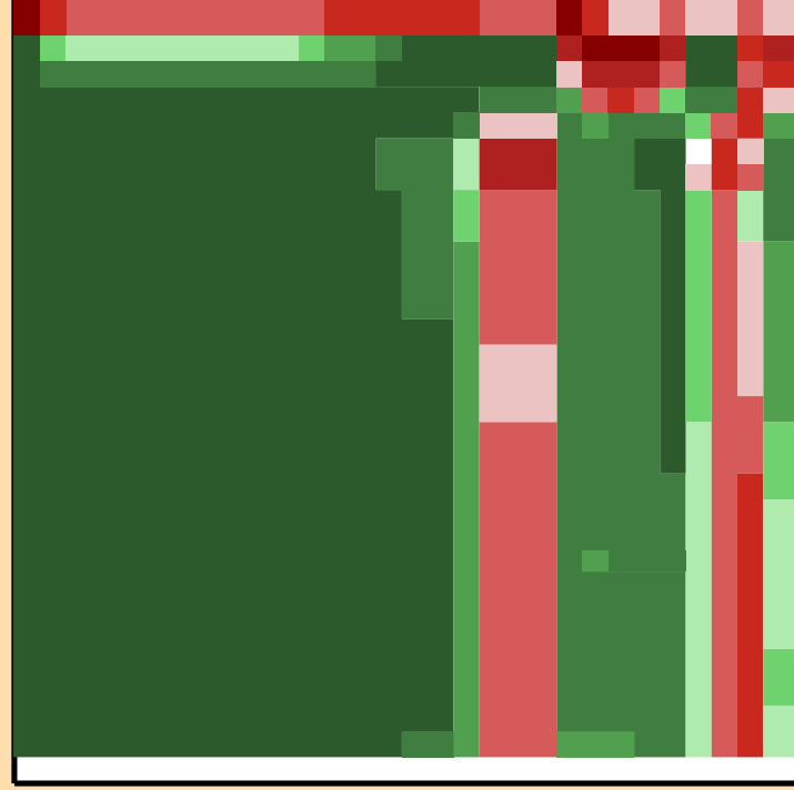
\Delta\sigma/\sigma vs. E for ^{194}\text{Tl}(n,\text{tot.})
