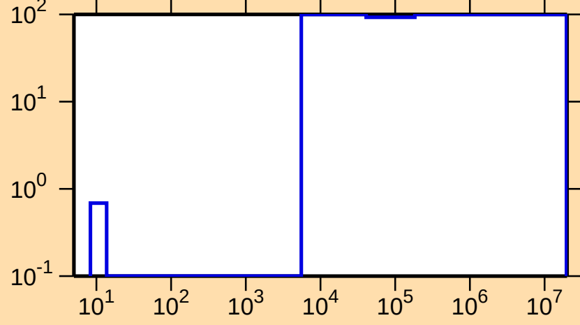
\Delta\sigma/\sigma vs. E for ^{194}\text{Tl}(n,n_1)
