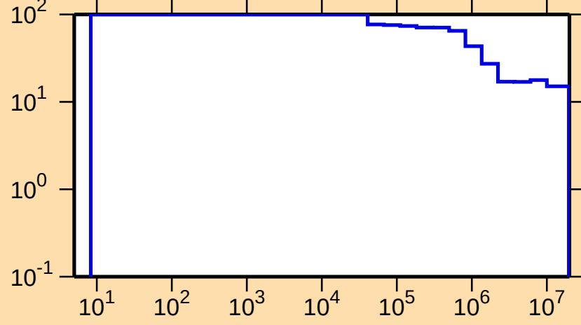
\Delta\sigma/\sigma vs. E for ^{194}\text{Tl}(n,\text{nonel.})
