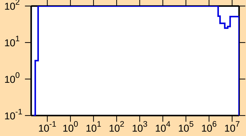
\Delta\sigma/\sigma vs. E for ^{194}\text{Tl}(n,n\text{cont.})
