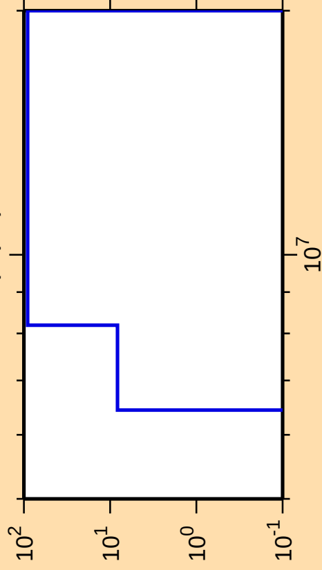
\Delta\sigma/\sigma vs. E for ^{194}\text{Tl}(n,p\alpha)
