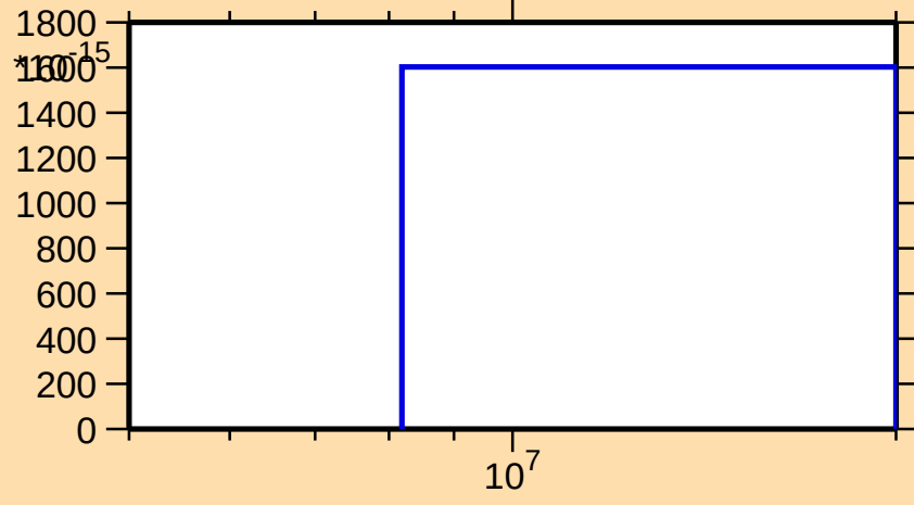
\sigma vs. E for ^{194}\text{Tl}(\text{mt 45})
