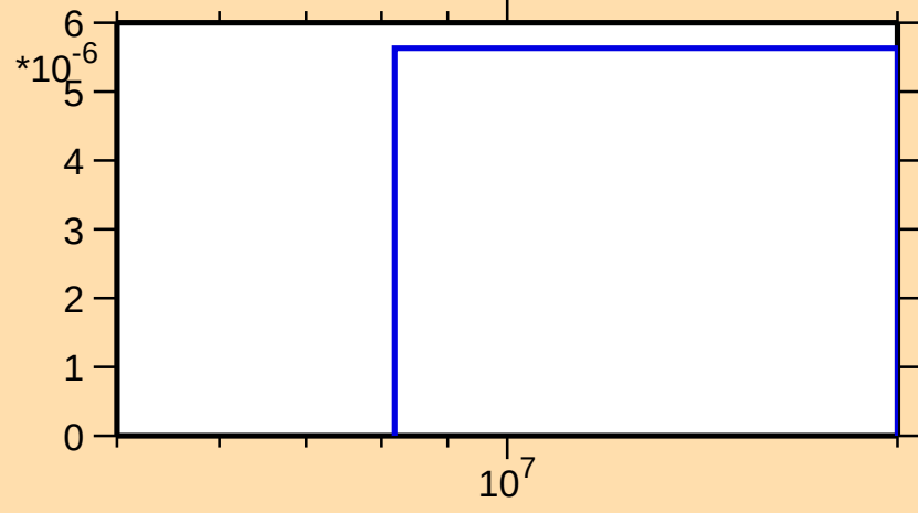
\sigma vs. E for ^{194}\text{Tl}(n,3n)
