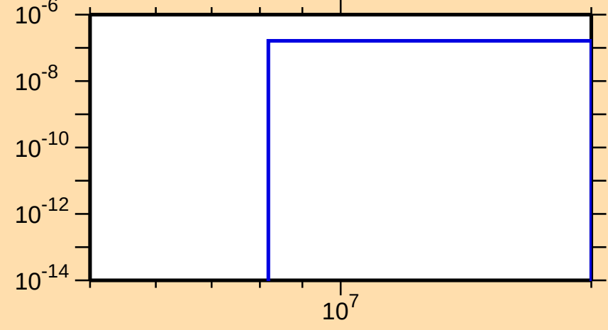
\sigma vs. E for ^{194}\text{Tl}(n,\text{nd})
