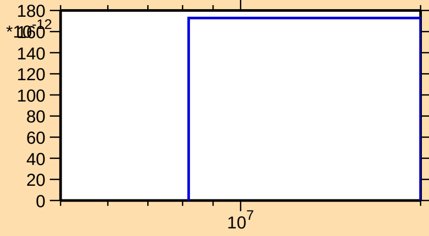
\sigma vs. E for ^{194}\text{Tl}(n,\text{nt})
