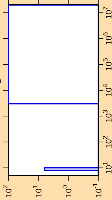
\Delta\sigma/\sigma vs. E for ^{194}\text{Tl}(n,n_1)
