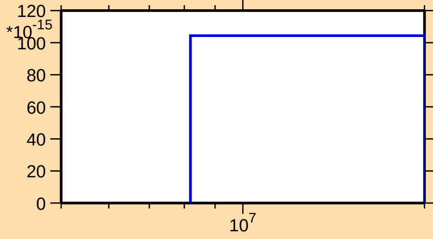
\sigma vs. E for ^{194}\text{Tl}(n,\text{pd})
