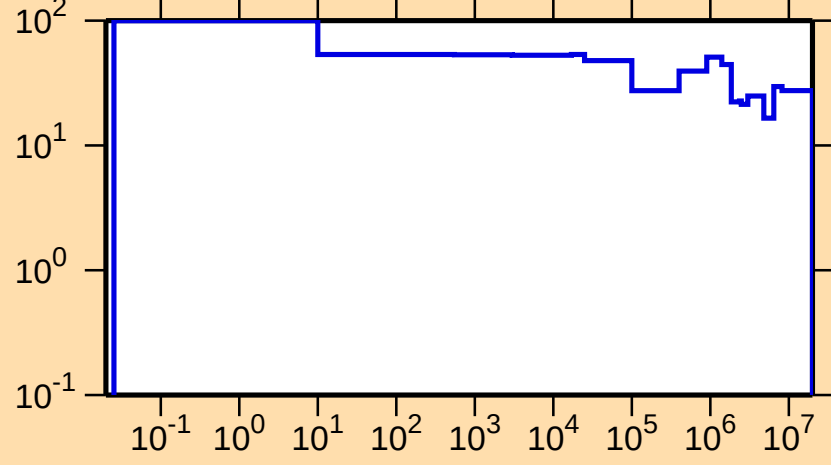
\Delta\sigma/\sigma vs. E for ^{194}\text{Tl}(n,\text{el.})
