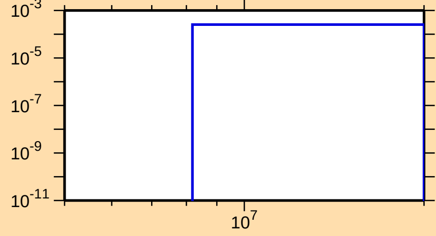
\sigma vs. E for ^{194}\text{Tl}(n,t)
