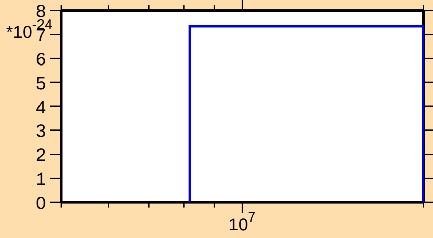
\sigma vs. E for ^{194}\text{Tl}(\text{mt } 42)
