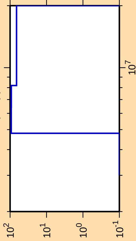
\Delta\sigma/\sigma vs. E for ^{194}\text{Tl}(n,np)
