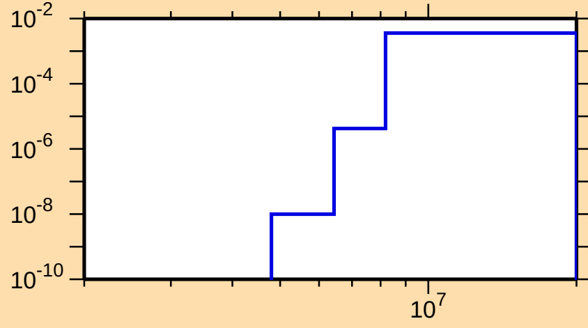
\sigma vs. E for ^{194}\text{Tl}(n,np)
