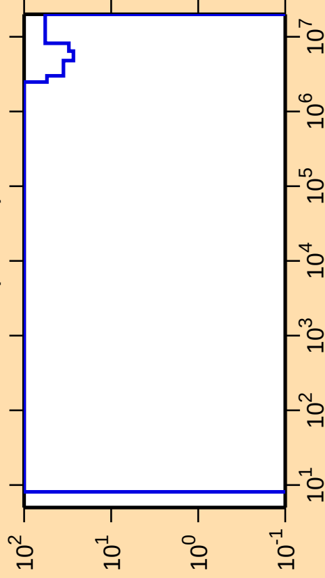
\Delta\sigma/\sigma vs. E for ^{194}\text{Tl}(n,\text{inel.})
