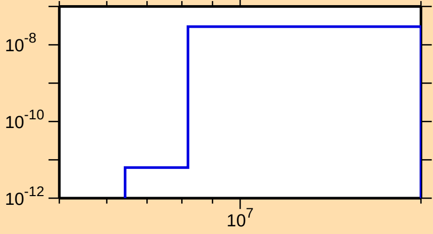
\sigma vs. E for ^{194}\text{Tl}(n,p\alpha)
