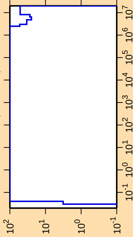
\Delta\sigma/\sigma vs. E for ^{194}\text{Tl}(n,\text{ncont.})
