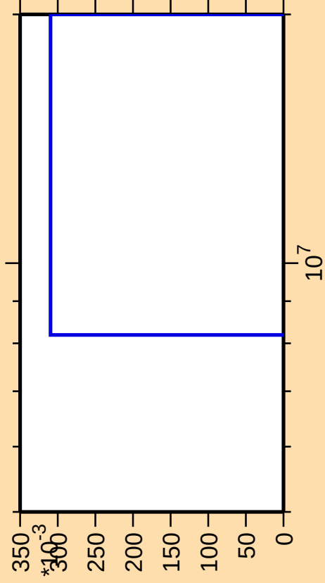
\Delta\sigma/\sigma vs. E for ^{194}\text{Tl}(\text{mt } 34)
