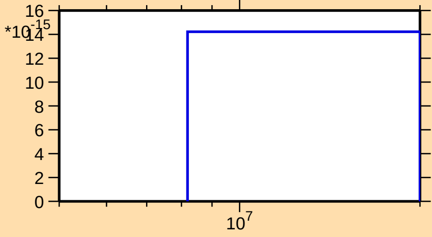
\sigma vs. E for ^{194}\text{Tl}(n,\text{pt})
