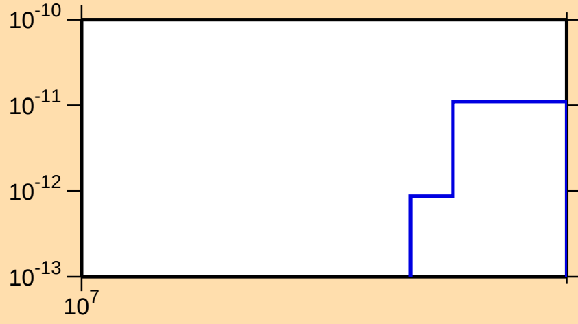
\sigma vs. E for ^{195}\text{Tl}(\text{mt } 45)
