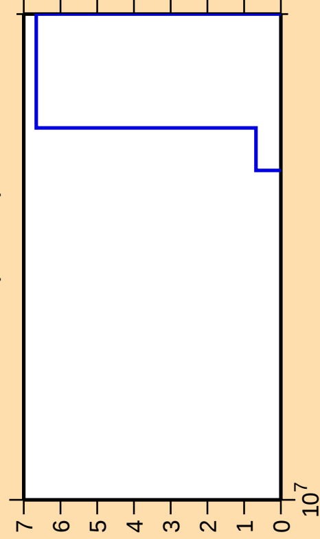
\Delta\sigma/\sigma vs. E for ^{195}\text{Tl}(\text{mt117})
