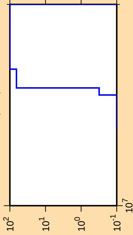
\Delta\sigma/\sigma vs. E for ^{195}\text{Tl}(n,\text{nt})
