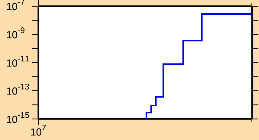
\sigma vs. E for ^{195}\text{Tl}(n,\text{nt})
