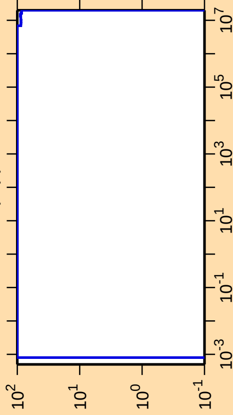
\Delta\sigma/\sigma vs. E for ^{195}\text{Tl}(n,p)
