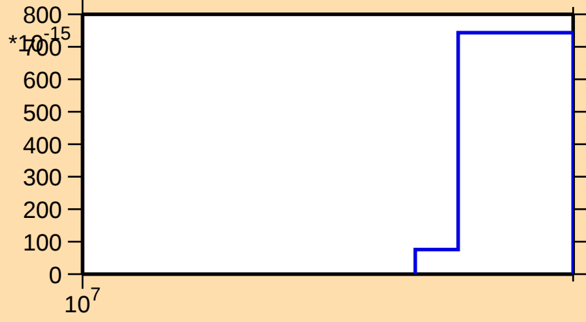
\sigma vs. E for ^{195}\text{Tl}(\text{mt117})
