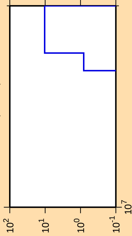
\Delta\sigma/\sigma vs. E for ^{195}\text{Tl}(\text{mt } 45)
