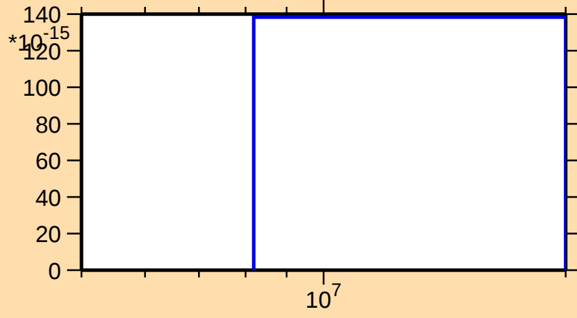
\sigma vs. E for ^{195}\text{Tl}(\text{mt } 45)
