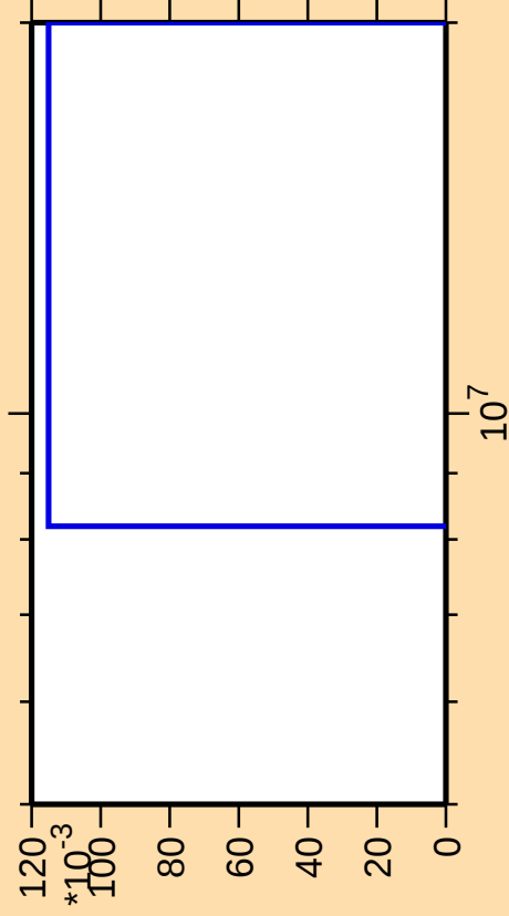
\Delta\sigma/\sigma vs. E for ^{195}\text{Tl}(\text{mt } 45)
