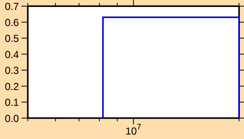
\sigma vs. E for ^{195}\text{Tl}(n,2n)
