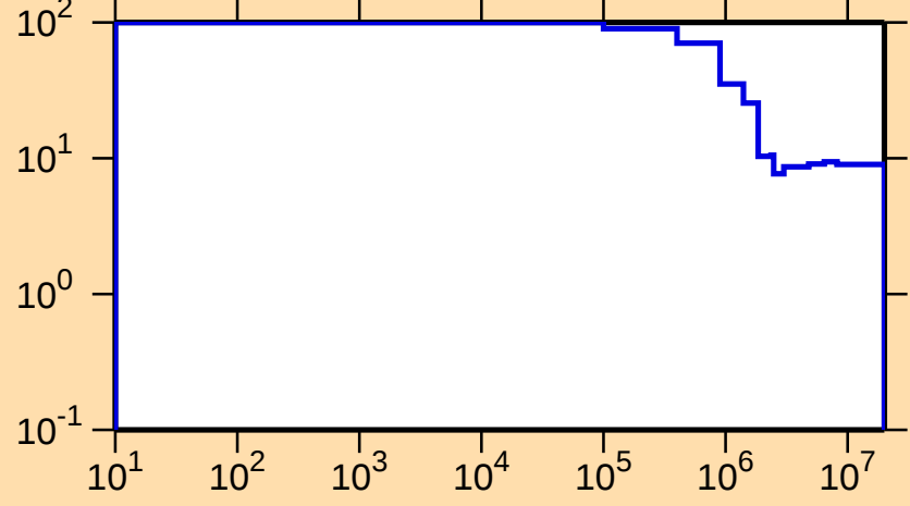
\Delta\sigma/\sigma vs. E for ^{195}\text{Tl}(n,\text{nonel.})
