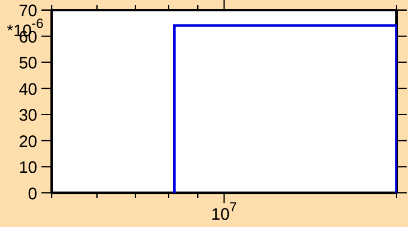
\sigma vs. E for ^{195}\text{Tl}(n,t)
