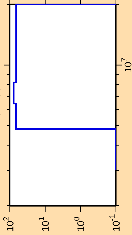
\Delta\sigma/\sigma vs. E for ^{195}\text{Tl}(n,np)
