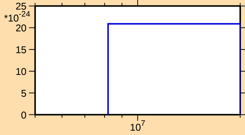
\sigma vs. E for ^{195}\text{Tl}(\text{mt } 42)
