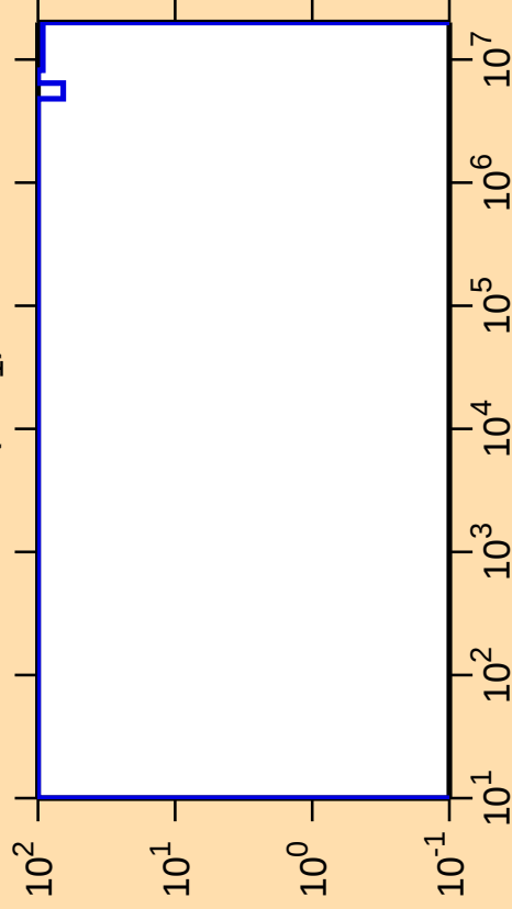
\Delta\sigma/\sigma vs. E for ^{195}\text{Tl}(n,n_1)
