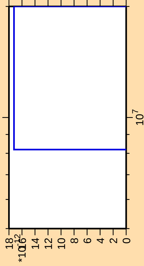
\Delta\sigma/\sigma vs. E for ^{195}\text{Tl}(\text{mt } 42)
