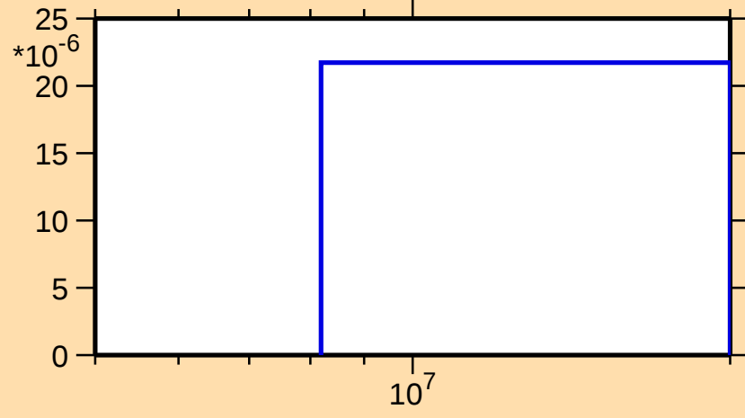
\sigma vs. E for ^{195}\text{Tl}(n,3n)
