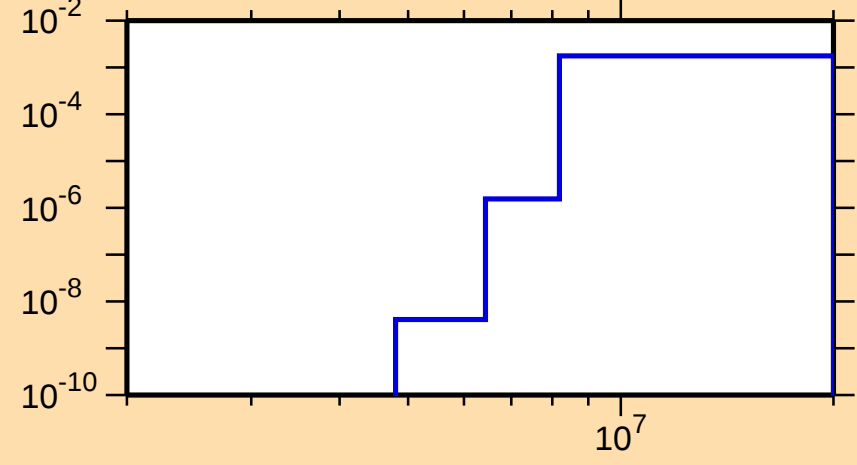
\sigma vs. E for ^{195}\text{Tl}(n,np)
