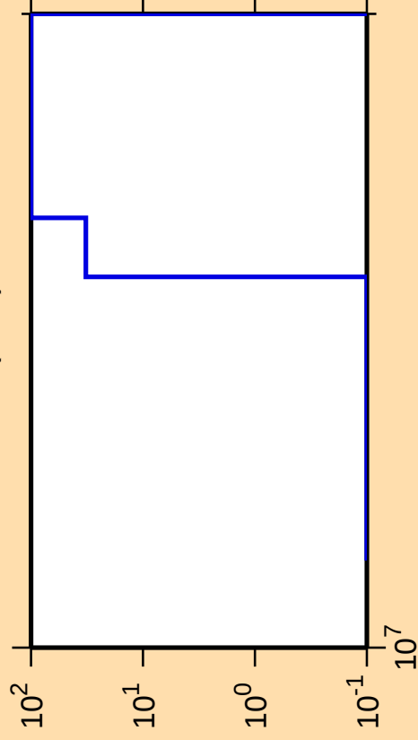
\Delta\sigma/\sigma vs. E for ^{196}\text{Tl}(n,\text{nt})
