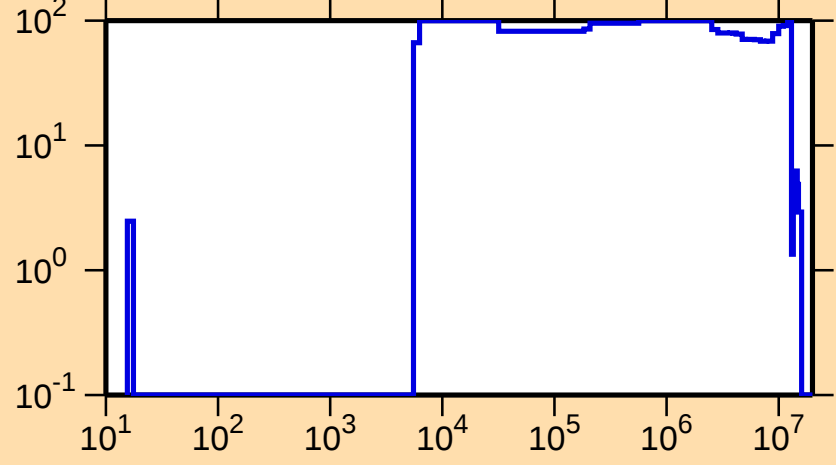
\Delta\sigma/\sigma vs. E for ^{196}\text{Tl}(n,n_1)
