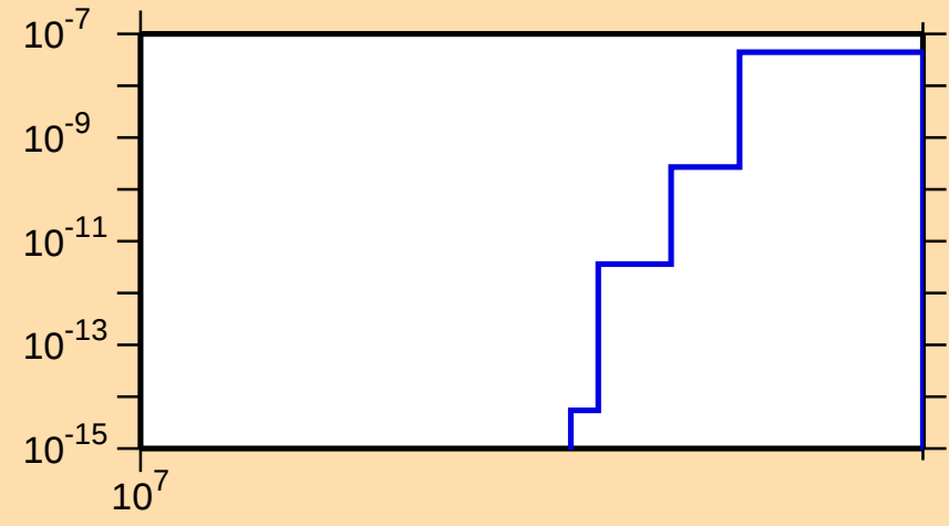
\sigma vs. E for ^{196}\text{Tl}(n,\text{nt})
