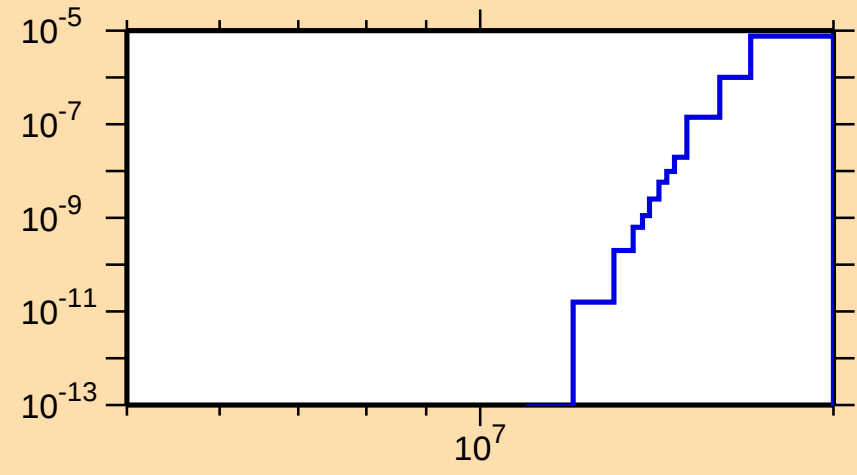
\sigma vs. E for ^{196}\text{Tl}(n,\text{nd})
