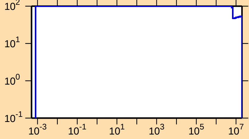
\Delta\sigma/\sigma vs. E for ^{196}\text{Tl}(n,p)
