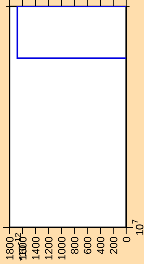
\Delta\sigma/\sigma vs. E for ^{196}\text{Tl}(\text{mt } 42)
