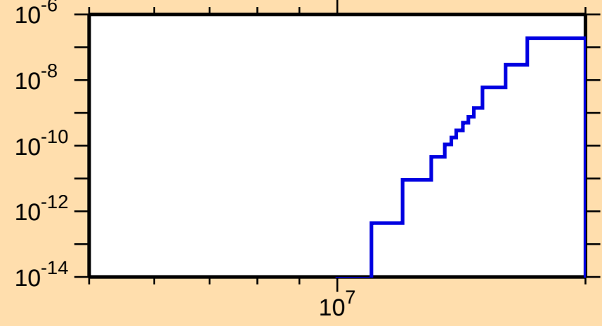
\sigma vs. E for ^{196}\text{Tl}(n,\text{He3})
