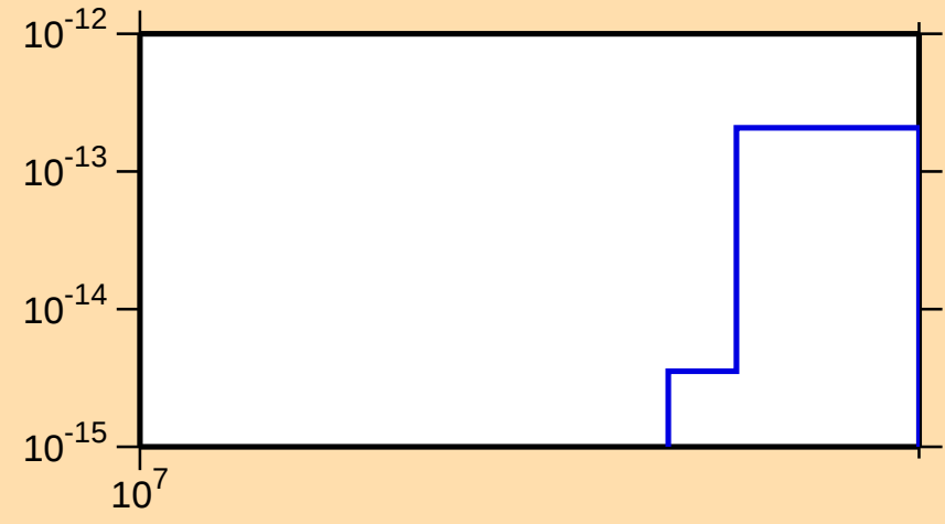
\sigma vs. E for ^{196}\text{Tl}(n,\text{pd})
