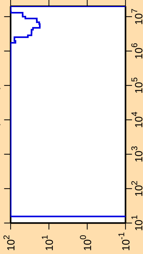
\Delta\sigma/\sigma vs. E for ^{196}\text{Tl}(n,\text{inel.})
