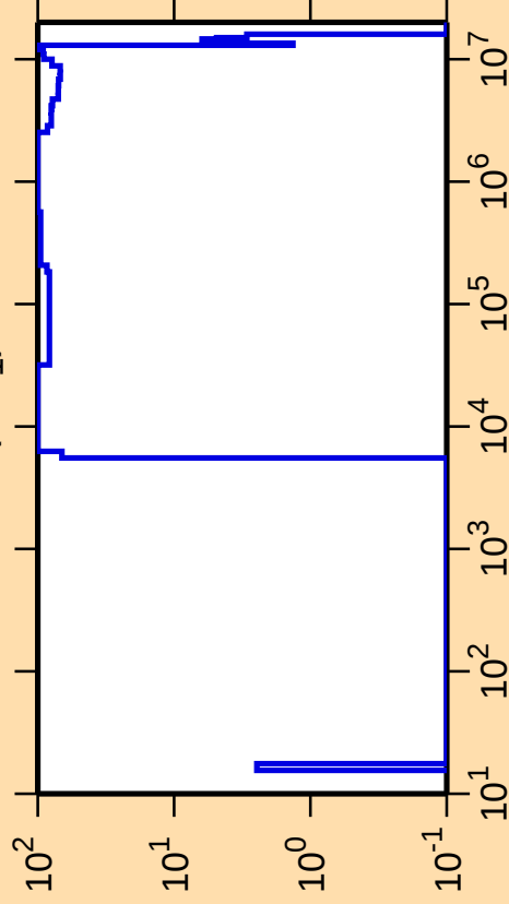
\Delta\sigma/\sigma vs. E for ^{196}\text{Tl}(n,n_1)
