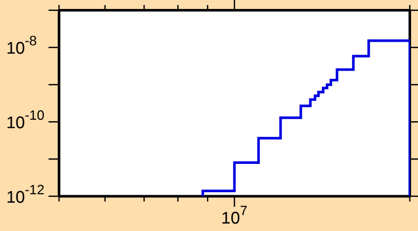
\sigma vs. E for ^{196}\text{Tl}(n,p\alpha)
