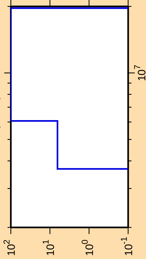
\Delta\sigma/\sigma vs. E for ^{196}\text{Tl}(n,n\alpha)
