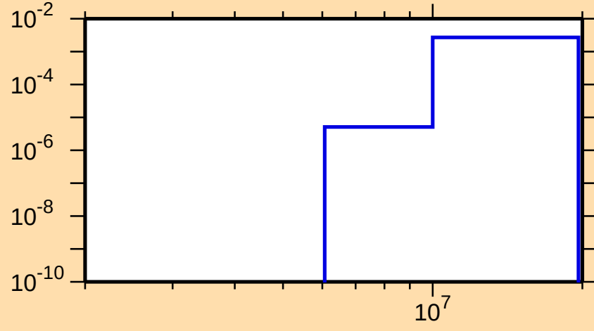
\sigma vs. E for ^{196}\text{Tl}(n,np)
