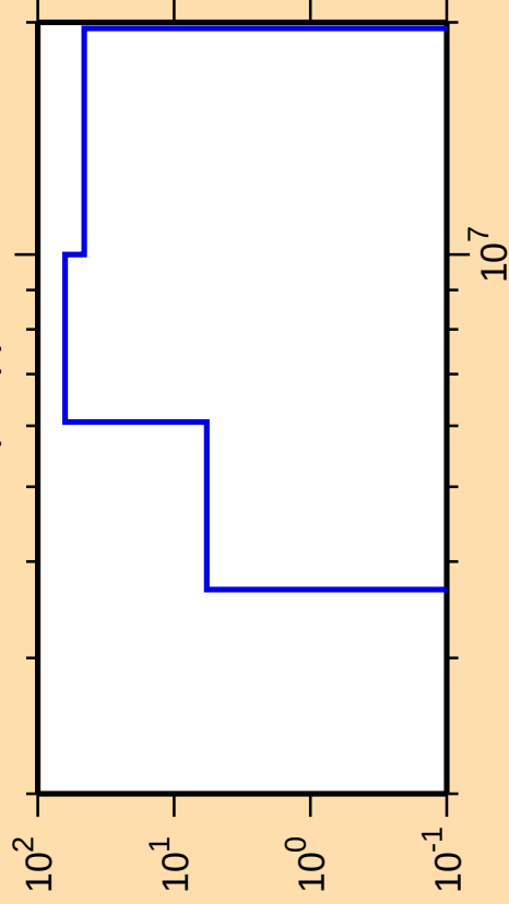
\Delta\sigma/\sigma vs. E for ^{196}\text{Tl}(n,np)
