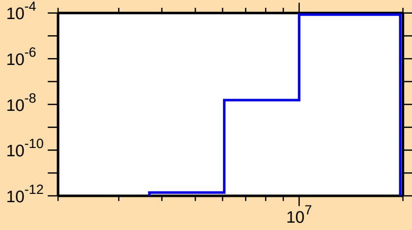
\sigma vs. E for ^{196}\text{Tl}(n,n\alpha)
