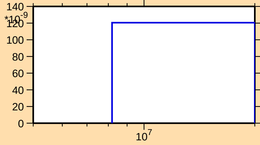
\sigma vs. E for ^{196}\text{Tl}(n,\text{nd})
