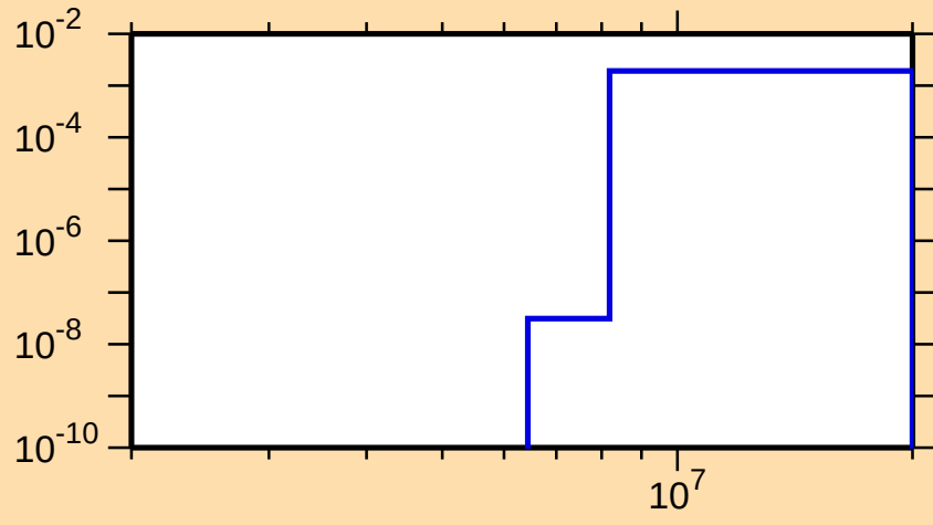
\sigma vs. E for ^{196}\text{Tl}(n,d)
