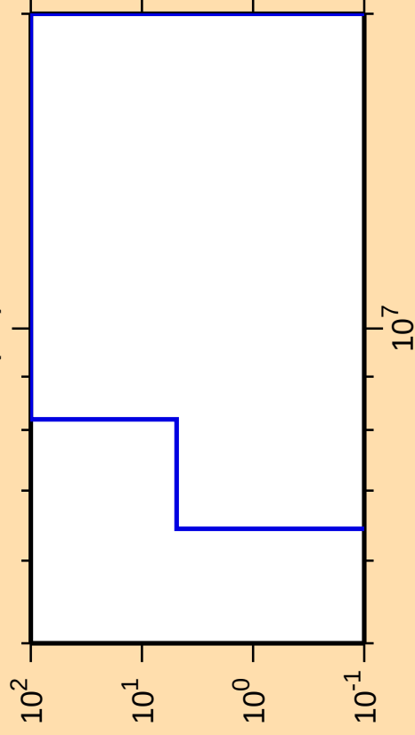
\Delta\sigma/\sigma vs. E for ^{196}\text{Tl}(n,t)
