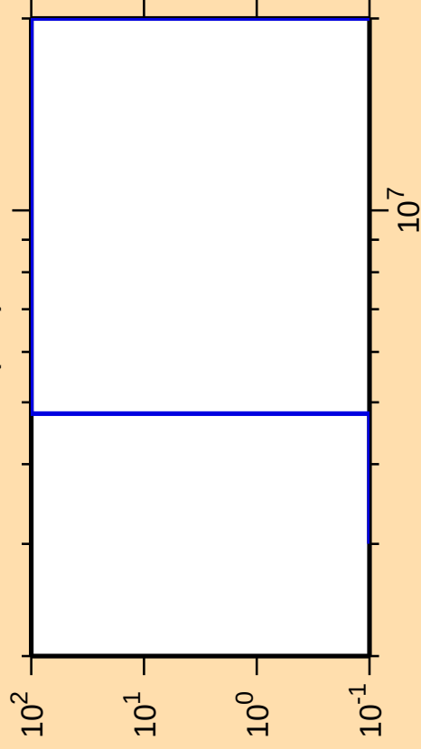
\Delta\sigma/\sigma vs. E for ^{196}\text{Tl}(n,d)
