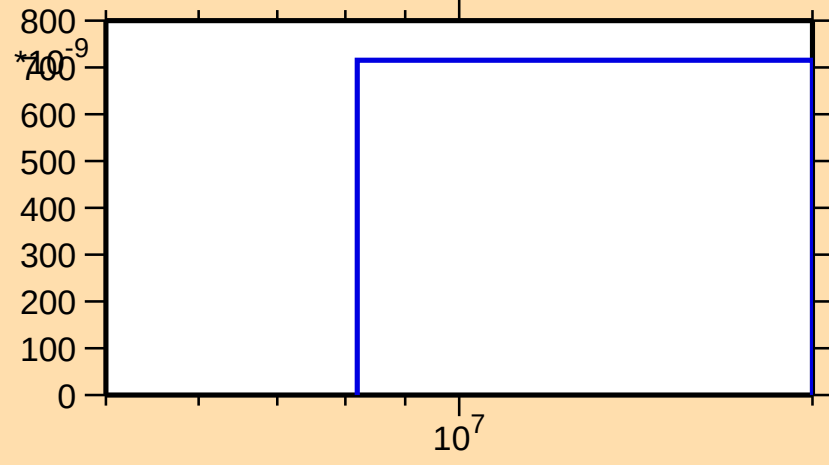
\sigma vs. E for ^{196}\text{Tl}(n,2np)
