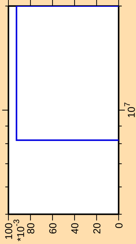
\Delta\sigma/\sigma vs. E for ^{196}\text{Tl}(\text{mt } 45)
