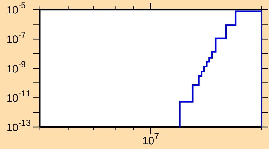
\sigma vs. E for ^{198}\text{Tl}(n,\text{nd})
