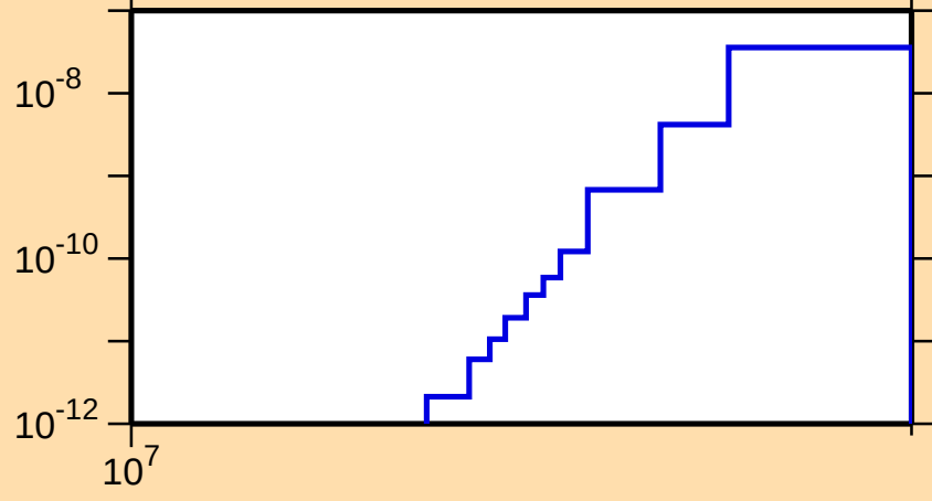
\sigma vs. E for ^{198}\text{Tl}(n,\text{He3})
