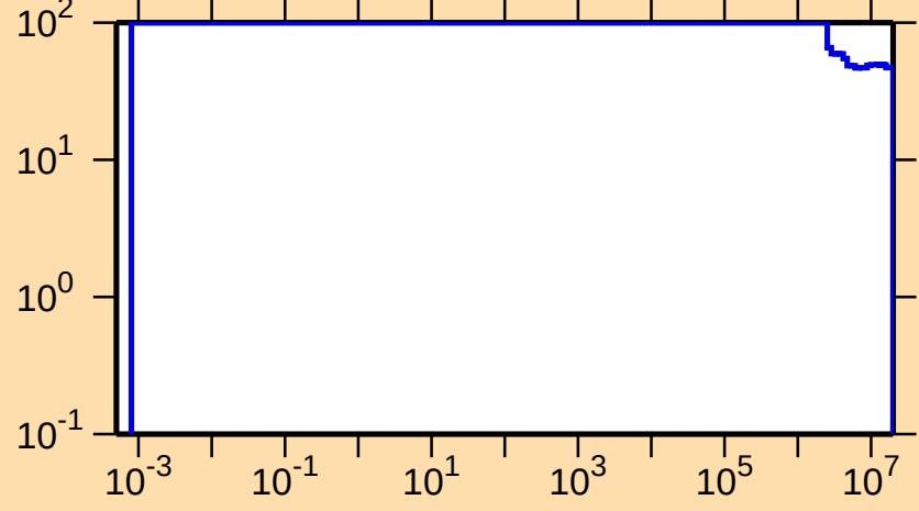
\Delta\sigma/\sigma vs. E for ^{198}\text{Tl}(n,p)
