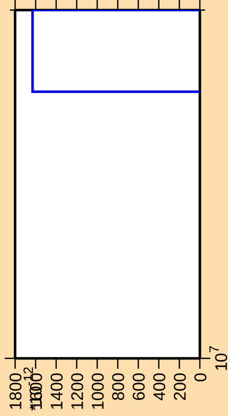
\Delta\sigma/\sigma vs. E for ^{198}\text{Tl} (mt 42)
