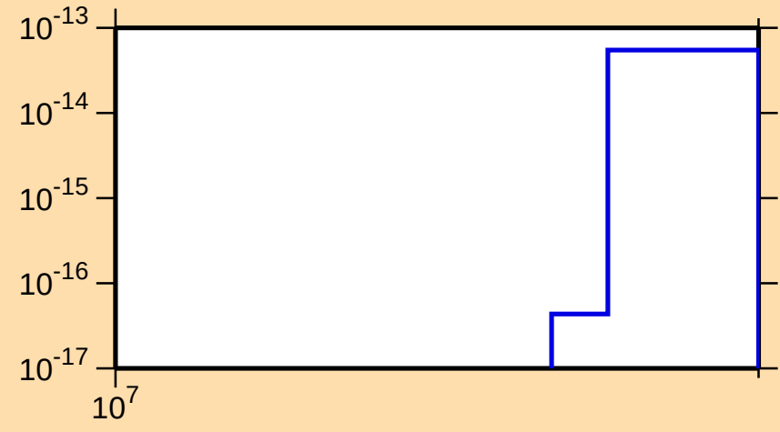
\sigma vs. E for ^{198}\text{Tl}(\text{mt } 34)
