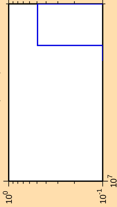
\Delta\sigma/\sigma vs. E for ^{198}\text{Tl}(\text{mt } 34)
