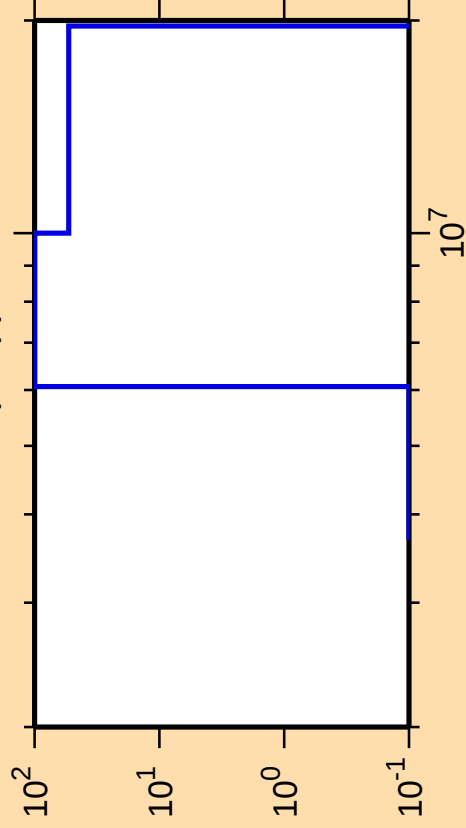
\Delta\sigma/\sigma vs. E for ^{198}\text{Tl}(n,np)
