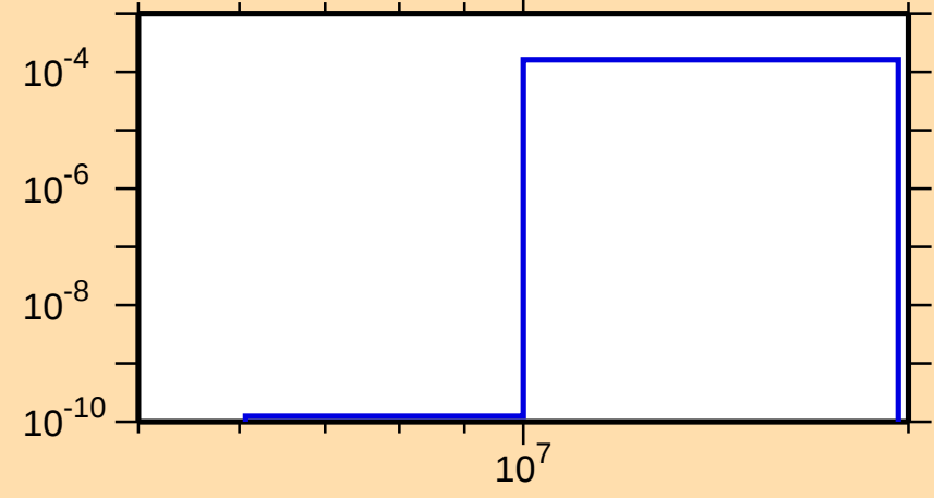
\sigma vs. E for ^{198}\text{Tl}(n,t)
