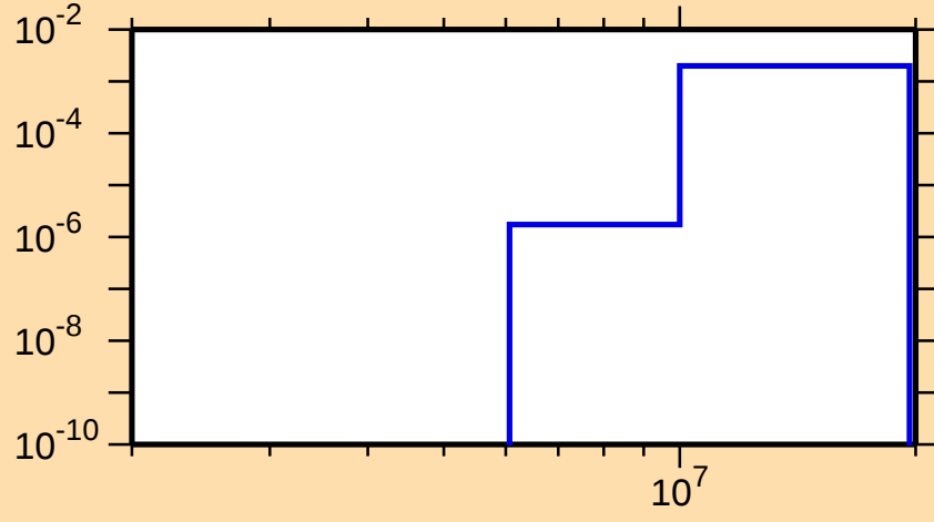
\sigma vs. E for ^{198}\text{Tl}(n,np)
