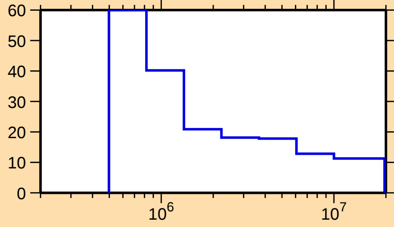
\Delta\sigma/\sigma vs. E for ^{198}\text{Tl}(n,n\text{nonel.})
