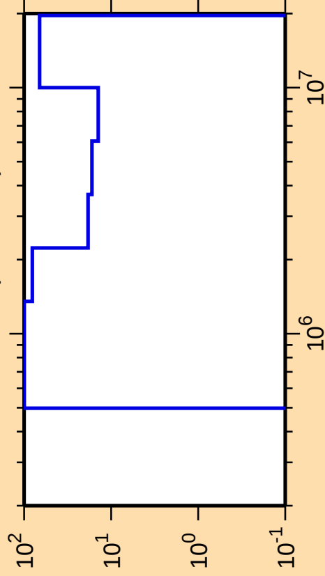
\Delta\sigma/\sigma vs. E for ^{198}\text{Tl}(n,n\text{cont.})
