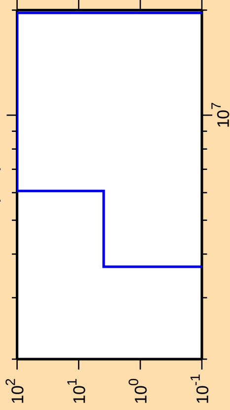
\Delta\sigma/\sigma vs. E for ^{198}\text{Tl}(n,d)
