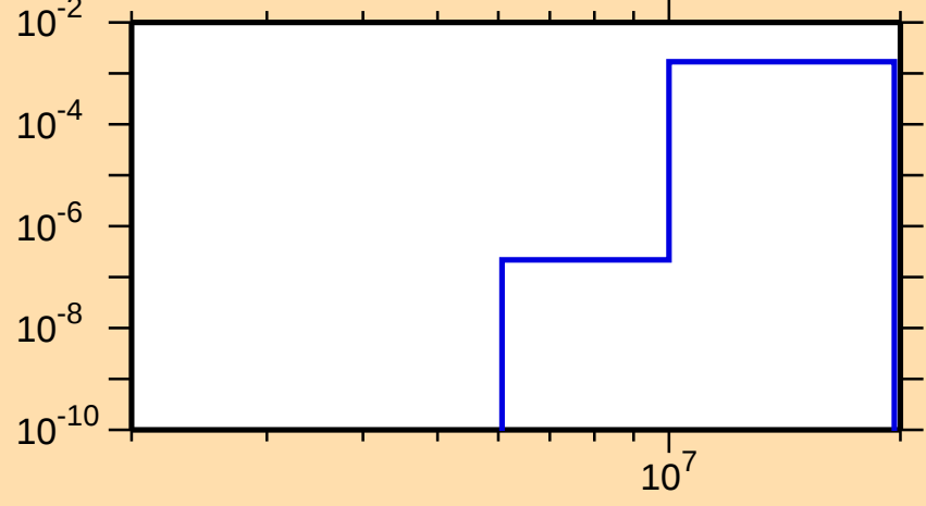
\sigma vs. E for ^{198}\text{Tl}(n,d)
