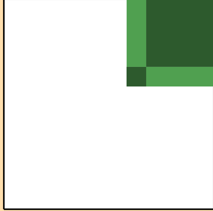
\sigma vs. E for ^{200}\text{Tl}(n,3n)
