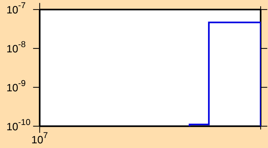
\sigma vs. E for ^{200}\text{Tl}(n,\text{nt})
