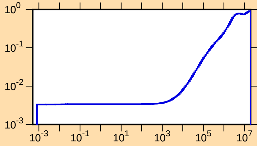
\mu vs. E for ^{203}\text{Tl}(\text{mt251})
