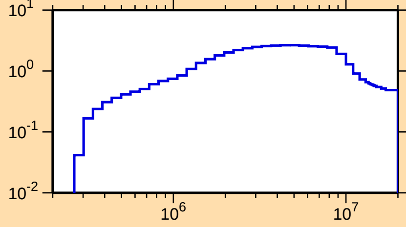
\sigma vs. E for ^{203}\text{Tl}(n,\text{inel.})
