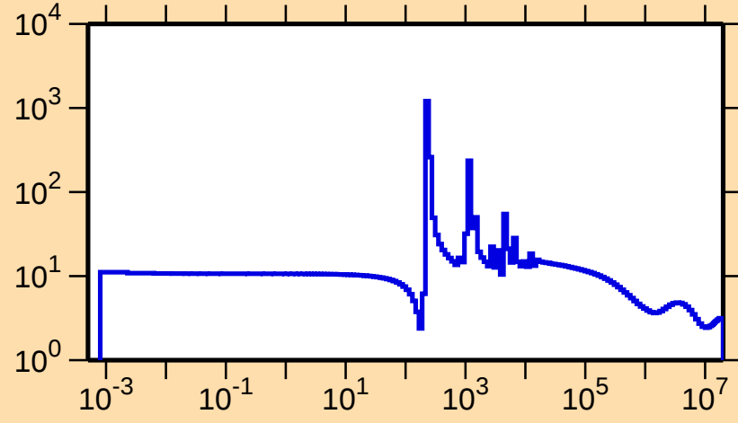
\sigma vs. E for ^{203}\text{Tl}(n,\text{el.})
