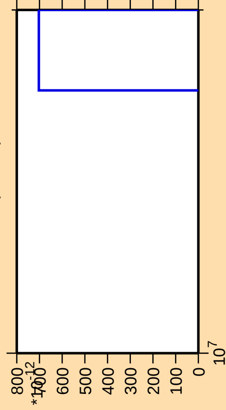
\Delta\sigma/\sigma vs. E for ^{203}\text{Tl}(\text{mt } 42)
