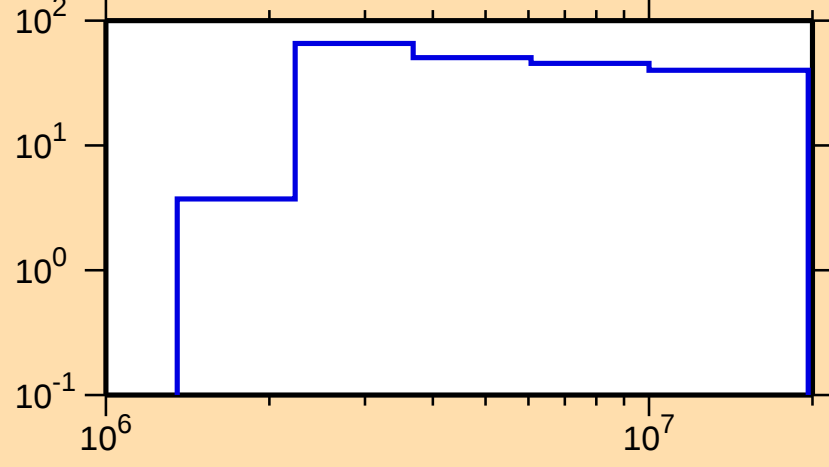
\Delta\sigma/\sigma vs. E for ^{203}\text{Tl}(n,p)
