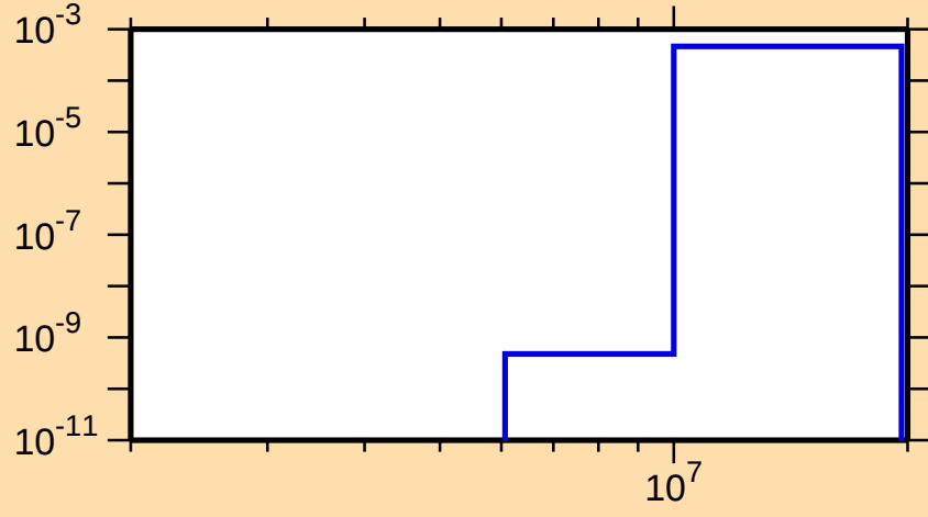
\sigma vs. E for ^{203}\text{Tl}(n,np)
