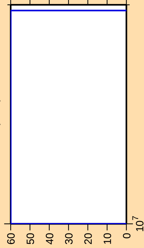
\Delta\sigma/\sigma vs. E for ^{203}\text{Tl}(n,\text{nt})
