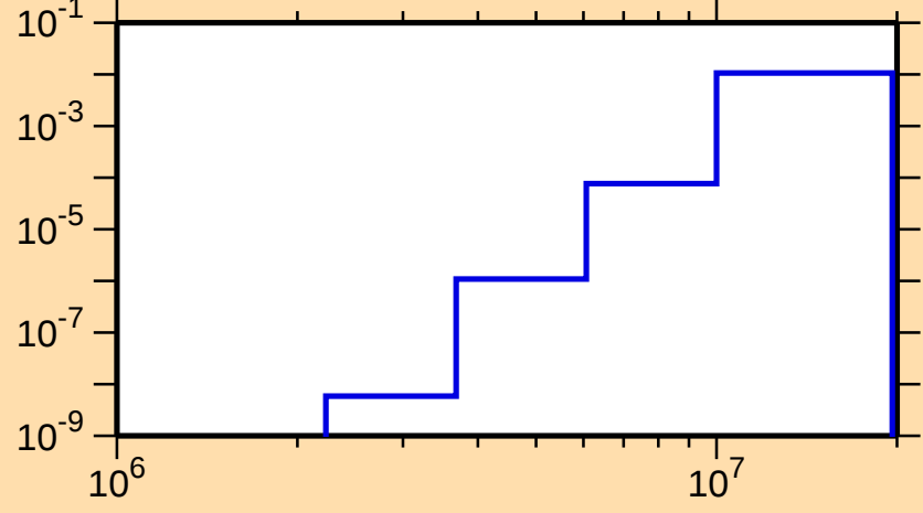
\sigma vs. E for ^{203}\text{Tl}(n,p)
