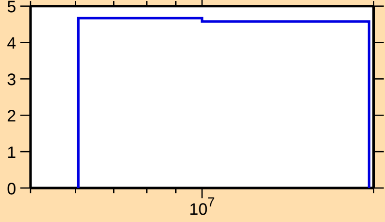
\Delta\sigma/\sigma vs. E for ^{203}\text{Tl}(n,2n)
