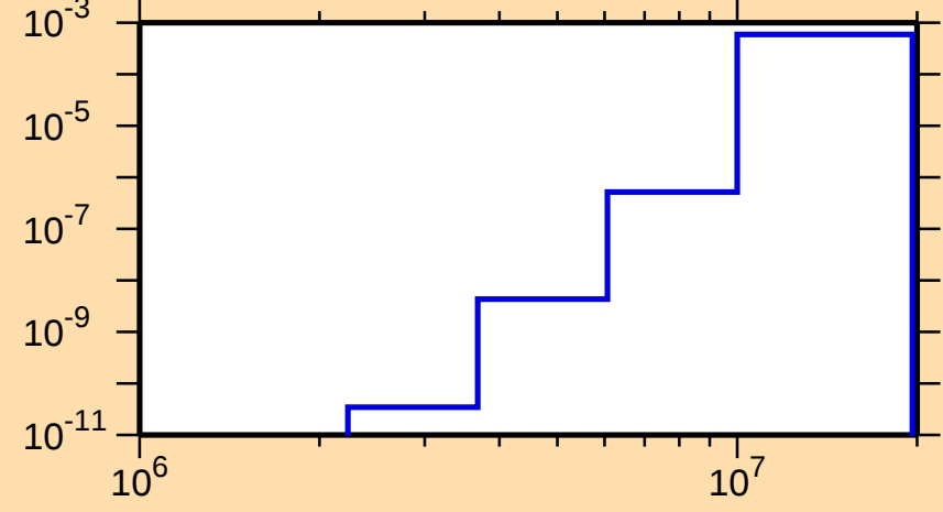
\sigma vs. E for ^{203}\text{Tl}(n,\alpha)
