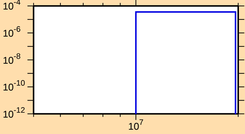
\sigma vs. E for ^{203}\text{Tl}(n,t)
