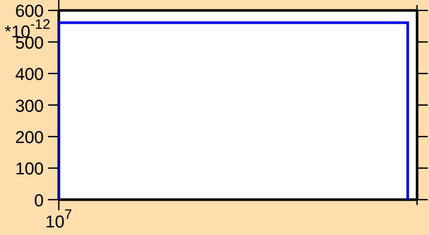
\sigma vs. E for ^{203}\text{Tl}(n,\text{nt})
