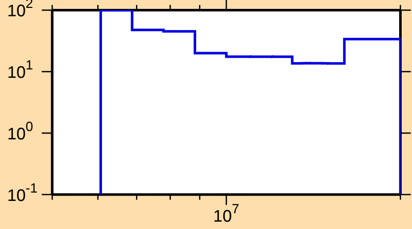
\Delta\sigma/\sigma vs. E for ^{204}\text{Tl}(n,2n)
