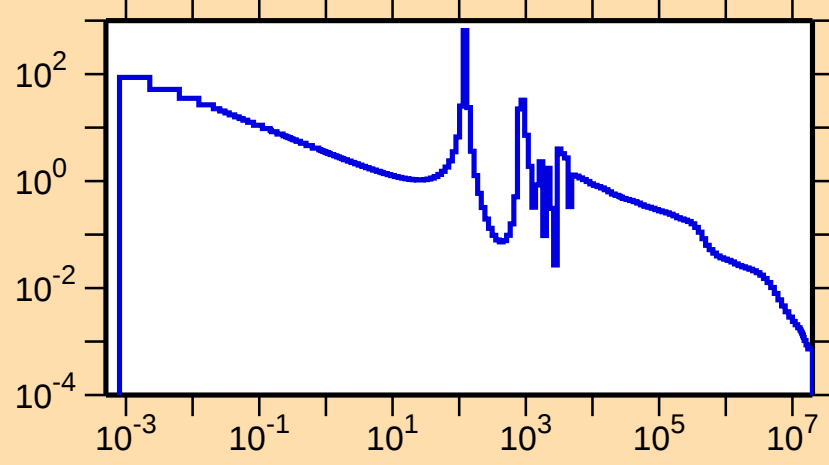
\sigma vs. E for ^{204}\text{Tl}(n,\gamma)
