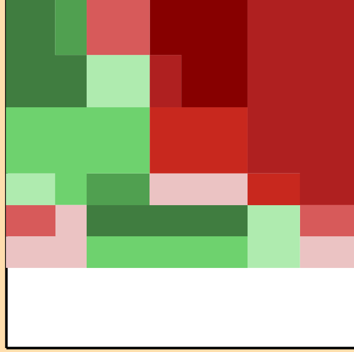
\Delta\sigma/\sigma vs. E for ^{204}\text{Tl}(n,\text{el.})
