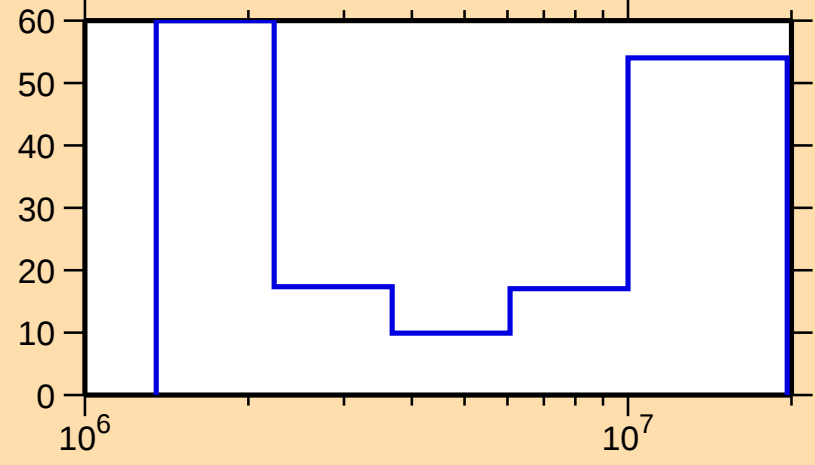
\Delta\sigma/\sigma vs. E for ^{204}\text{Tl}(n,n\text{cont.})
