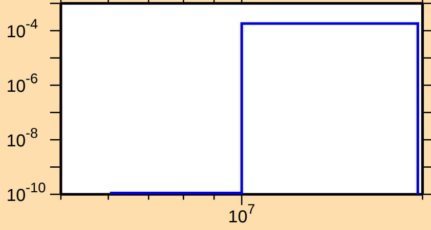
\sigma vs. E for ^{204}\text{Tl}(n,d)
