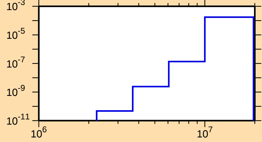
\sigma vs. E for ^{204}\text{Tl}(n,\alpha)
