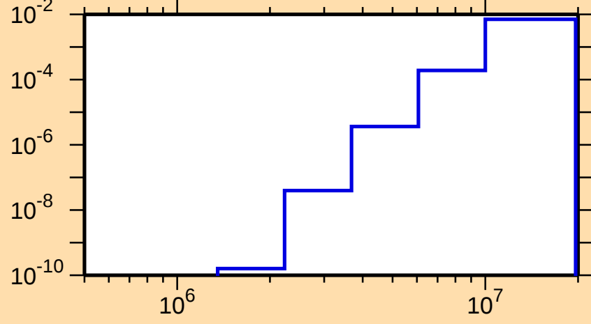
\sigma vs. E for ^{204}\text{Tl}(n,p)
