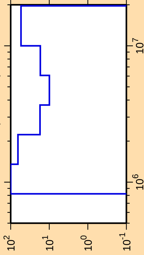
\Delta\sigma/\sigma vs. E for ^{204}\text{Tl}(n,\text{ncont.})
