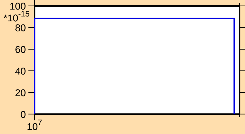
\sigma vs. E for ^{204}\text{Tl}(n,\text{He3})
