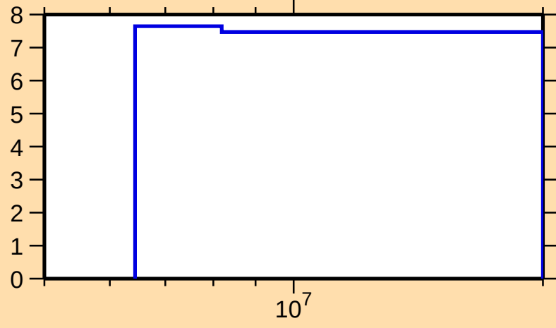
\Delta\sigma/\sigma vs. E for ^{204}\text{Tl}(n,\text{nonel.})
