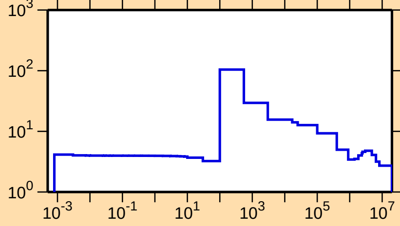
\sigma vs. E for ^{204}\text{Tl}(n,\text{el.})
