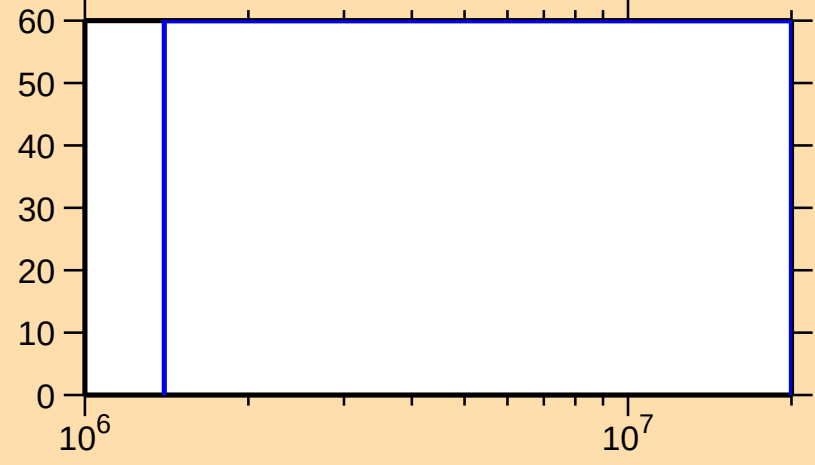
\Delta\sigma/\sigma vs. E for ^{204}\text{Tl}(n,\gamma)
