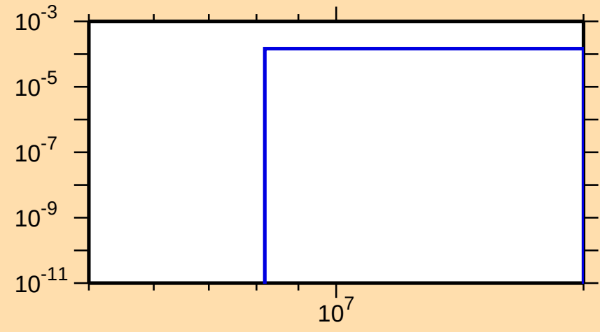
\sigma vs. E for ^{204}\text{Tl}(n,d)
