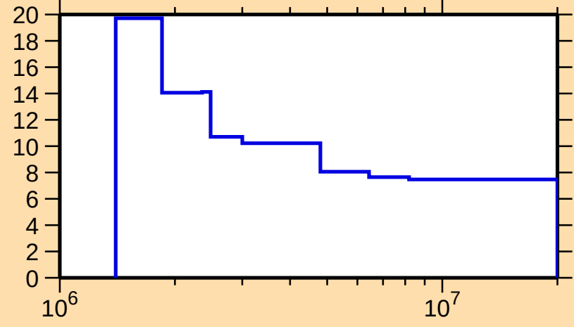
\Delta\sigma/\sigma vs. E for ^{204}\text{Tl}(n,\text{nonel.})
