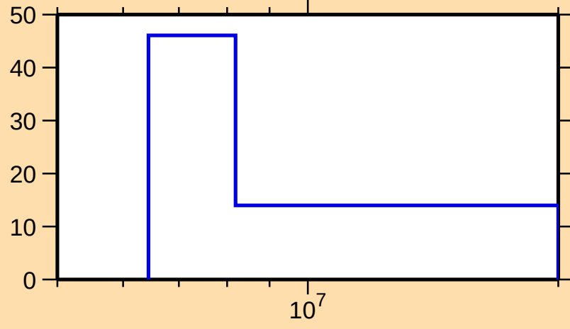
\Delta\sigma/\sigma vs. E for ^{204}\text{Tl}(n,2n)
