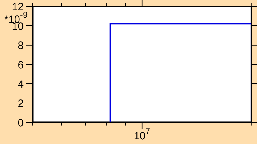
\sigma vs. E for ^{204}\text{Tl}(n,\text{nd})
