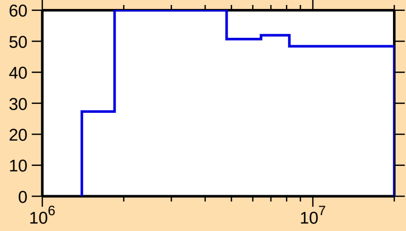
\Delta\sigma/\sigma vs. E for ^{204}\text{Tl}(n,p)
