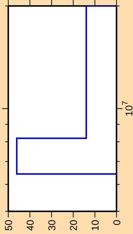
\Delta\sigma/\sigma vs. E for ^{204}\text{Tl}(n,2n)
