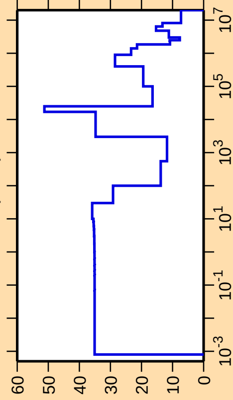
\Delta\sigma/\sigma vs. E for ^{204}\text{Tl}(n,\text{el.})
