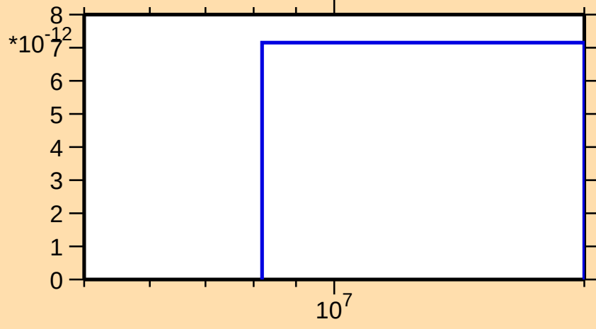
\sigma vs. E for ^{204}\text{Tl}(n,2n\alpha)
