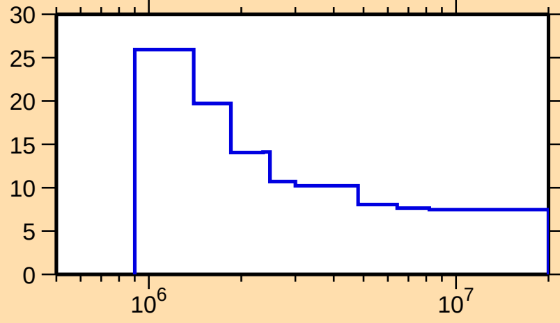
\Delta\sigma/\sigma vs. E for ^{204}\text{Tl}(n,n\text{nonel.})
