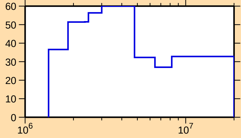
\Delta\sigma/\sigma vs. E for ^{204}\text{Tl}(n,n_1)
