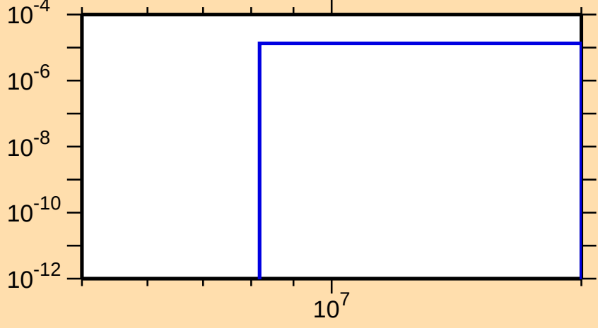
\sigma vs. E for ^{204}\text{Tl}(n,t)
