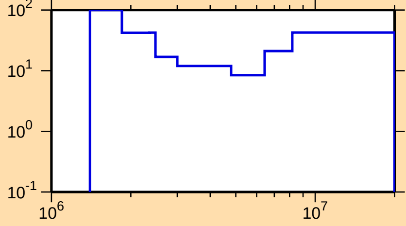
\Delta\sigma/\sigma vs. E for ^{204}\text{Tl}(n,n\text{cont.})
