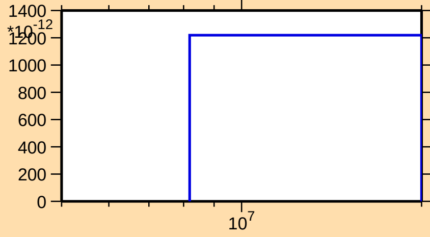
\sigma vs. E for ^{204}\text{Tl}(n,2np)
