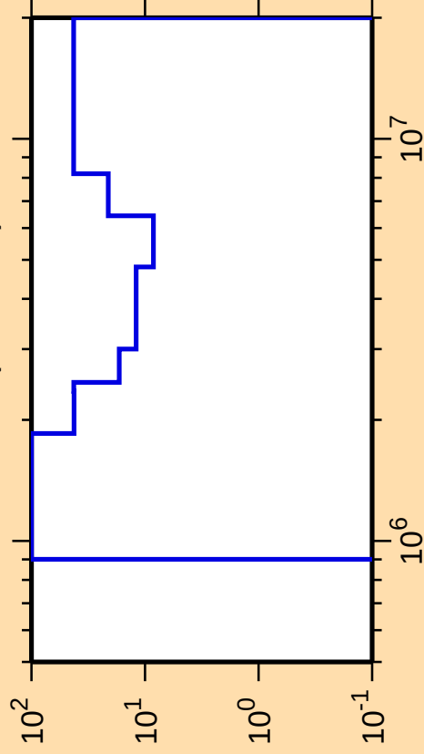
\Delta\sigma/\sigma vs. E for ^{204}\text{Tl}(n,n\text{cont.})
