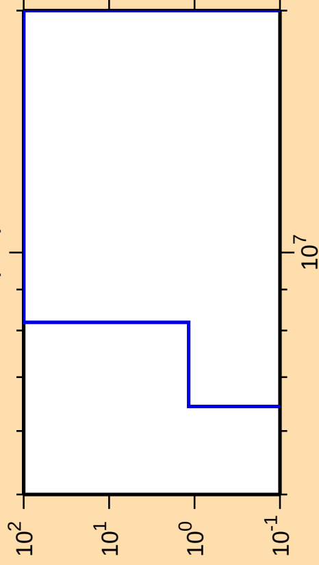
\Delta\sigma/\sigma vs. E for ^{204}\text{Tl}(n,d)
