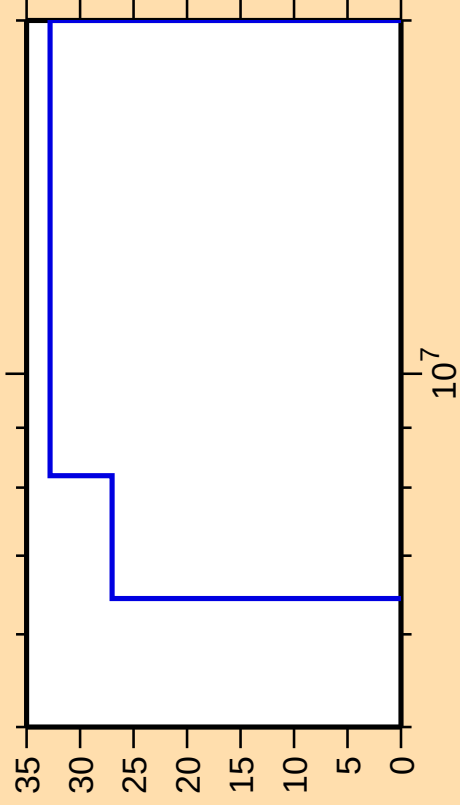
\Delta\sigma/\sigma vs. E for ^{204}\text{Tl}(n,n_1)
