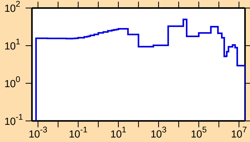
\Delta\sigma/\sigma vs. E for ^{204}\text{Tl}(n,\text{tot.})
