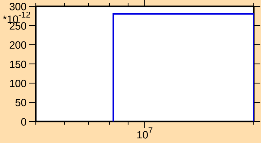
\sigma vs. E for ^{204}\text{Tl}(n,\text{nt})
