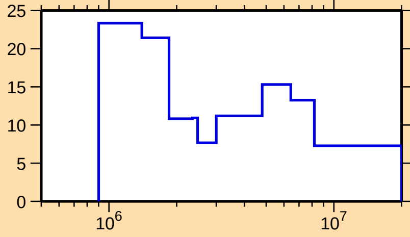
\Delta\sigma/\sigma vs. E for ^{204}\text{Tl}(n,\text{el.})
