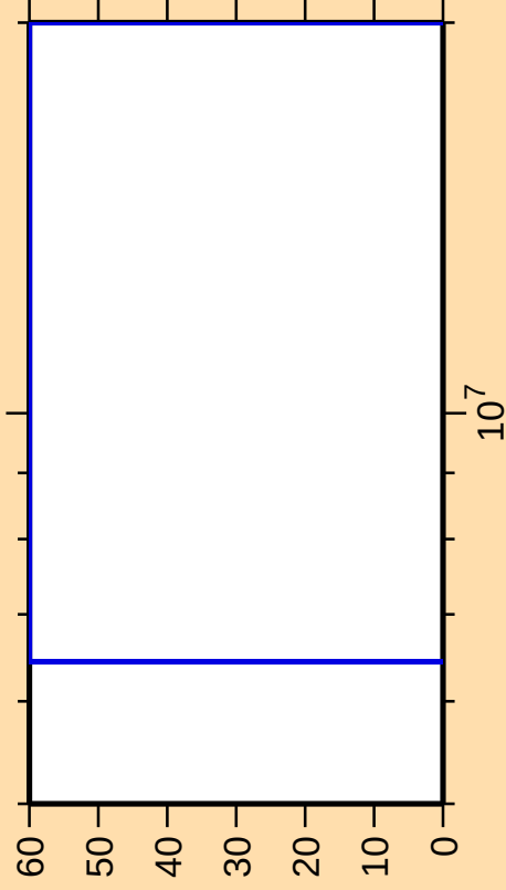
\Delta\sigma/\sigma vs. E for ^{204}\text{Tl}(n,\gamma)
