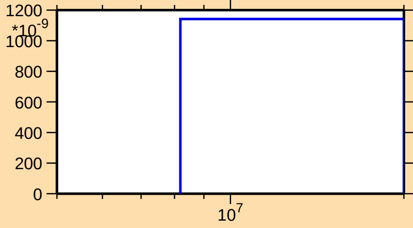
\sigma vs. E for ^{204}\text{Tl}(n,n\alpha)
