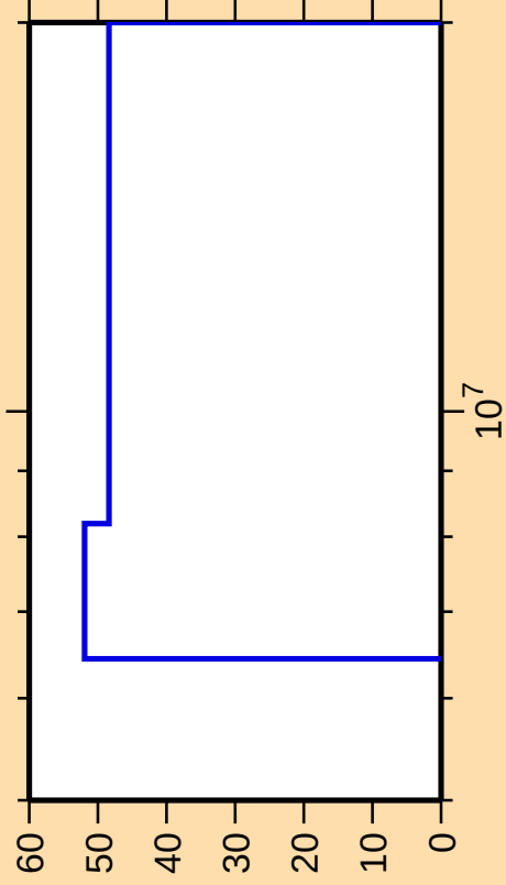
\Delta\sigma/\sigma vs. E for ^{204}\text{Tl}(n,p)
