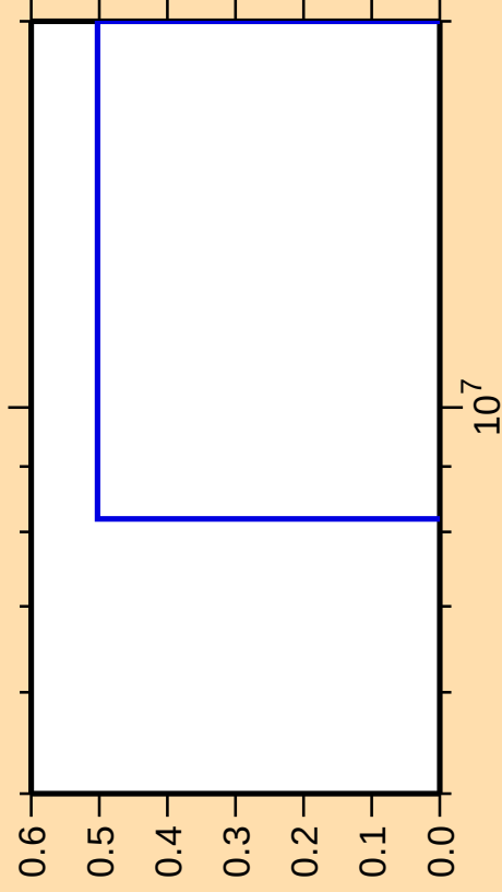
\Delta\sigma/\sigma vs. E for ^{204}\text{Tl}(n,\text{He}3)
