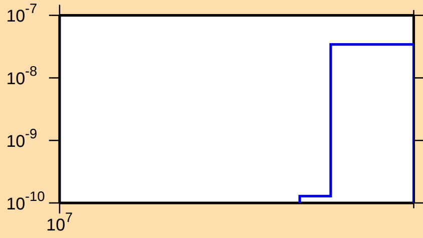
\sigma vs. E for ^{207}\text{Tl}(n,\text{nd})
