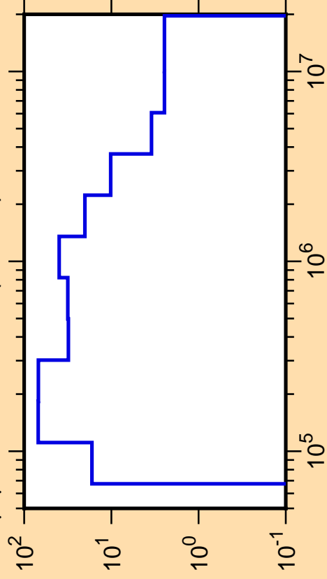
\Delta\mu/\mu vs. E for ^{207}\text{Tl}(\text{mt251})
