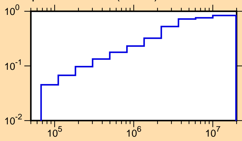
\mu vs. E for ^{207}\text{Tl}(\text{mt251})
