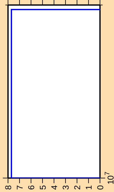
\Delta\sigma/\sigma vs. E for ^{207}\text{Tl}(n,2np)
