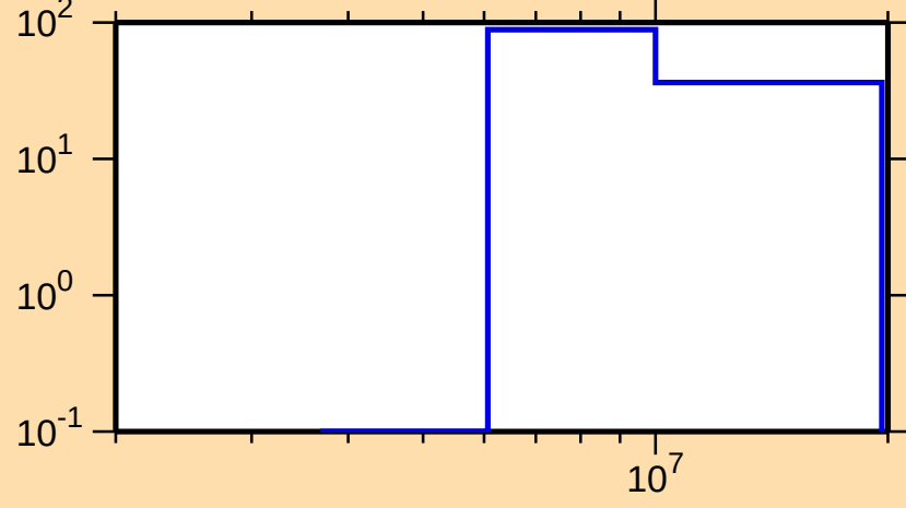
\Delta\sigma/\sigma vs. E for ^{207}\text{Tl}(n,p)
