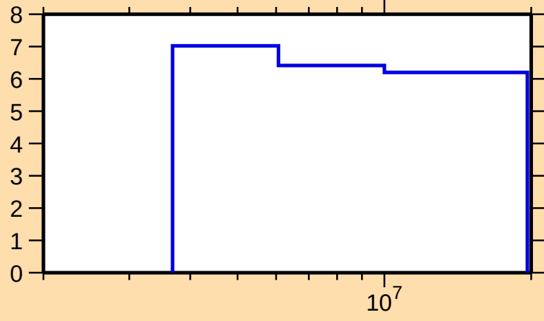
\Delta\sigma/\sigma vs. E for ^{207}\text{Tl}(n,n\text{nonel.})
