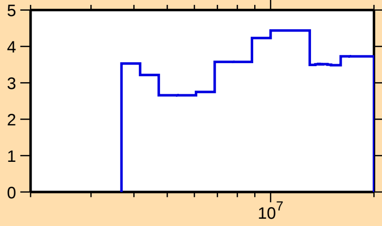
\Delta\sigma/\sigma vs. E for ^{208}\text{Tl}(n,\text{nonel.})
