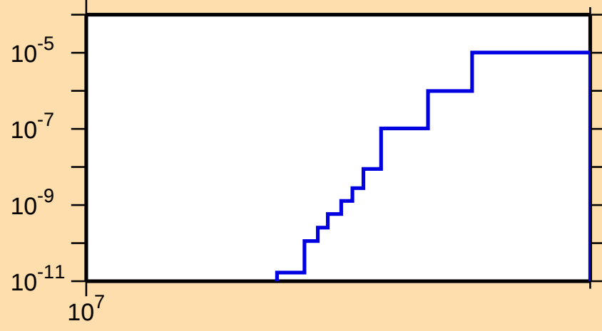
\sigma vs. E for ^{208}\text{Tl}(n,\text{nd})
