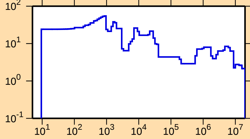
\Delta\sigma/\sigma vs. E for ^{208}\text{Tl}(n,\text{el.})
