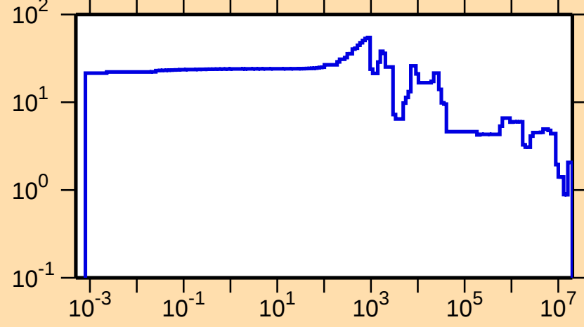
\Delta\sigma/\sigma vs. E for ^{208}\text{Tl}(n,\text{tot.})
