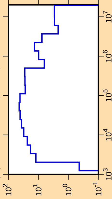
\Delta\mu/\mu vs. E for ^{208}\text{Tl}(\text{mt251})
