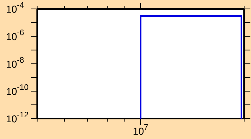
\sigma vs. E for ^{208}\text{Tl}(n,np)
