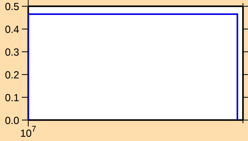
\sigma vs. E for ^{208}\text{Tl}(n,3n)
