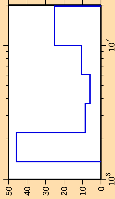
\Delta\sigma/\sigma vs. E for ^{208}\text{Tl}(n,\text{ncont.})
