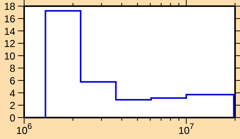
\Delta\sigma/\sigma vs. E for ^{208}\text{Tl}(n,n\text{nonel.})
