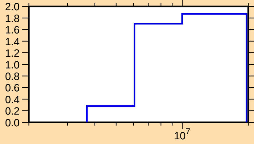
\sigma vs. E for ^{208}\text{Tl}(n,2n)
