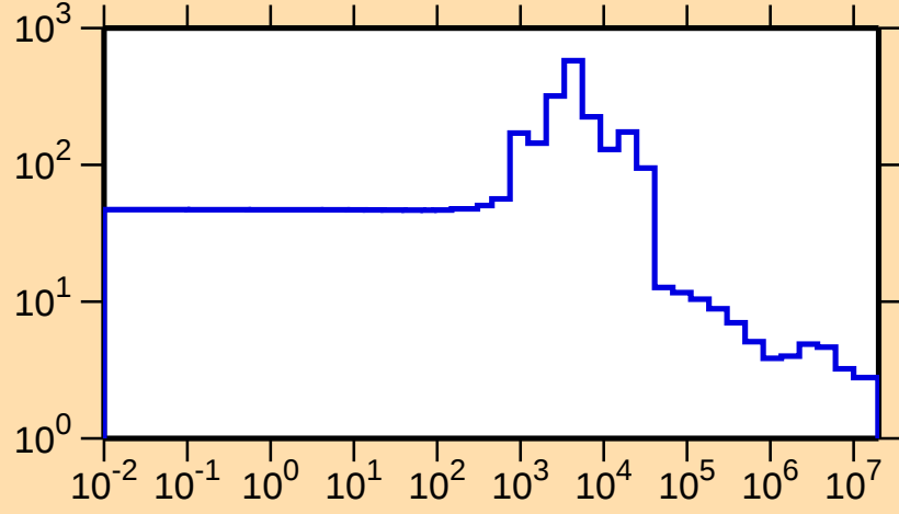
\sigma vs. E for ^{208}\text{Tl}(n,\text{el.})
