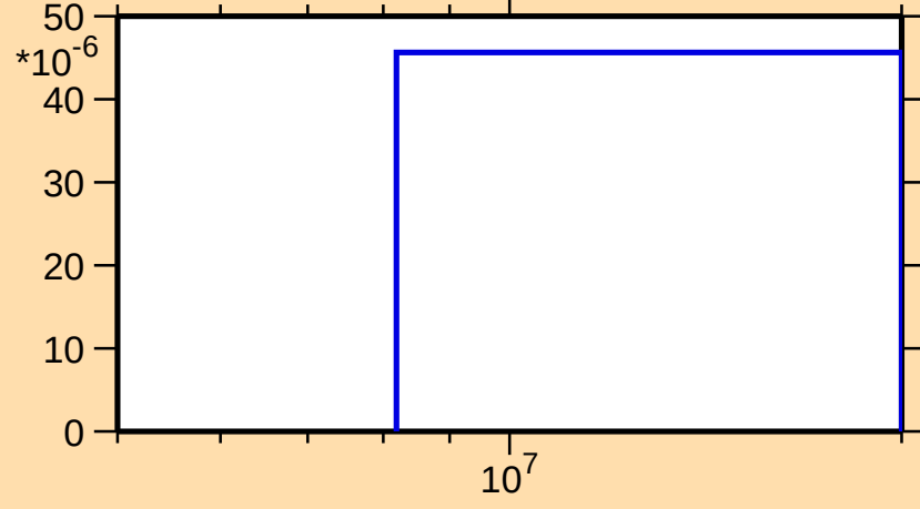
\sigma vs. E for ^{208}\text{Tl}(n,d)
