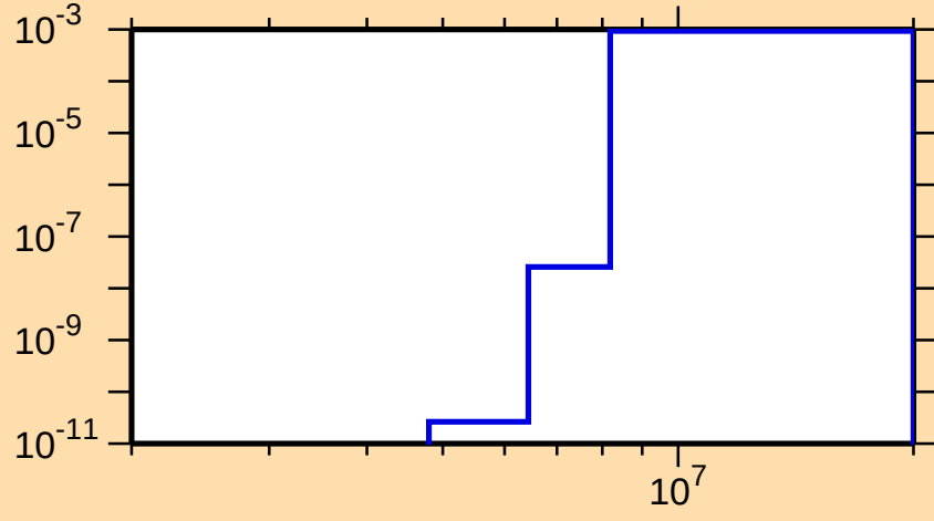
\sigma vs. E for ^{208}\text{Tl}(n,p)
