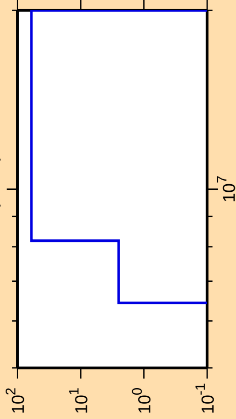
\Delta\sigma/\sigma vs. E for ^{208}\text{Tl}(n,n\alpha)
