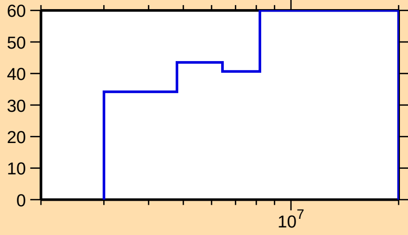
\Delta\sigma/\sigma vs. E for ^{208}\text{Tl}(n,\gamma)
