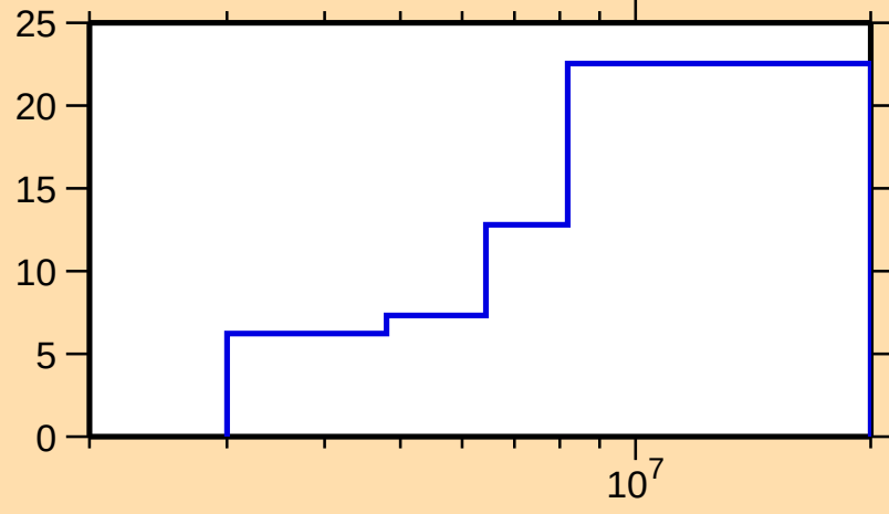
\Delta\sigma/\sigma vs. E for ^{208}\text{Tl}(n,n\text{cont.})
