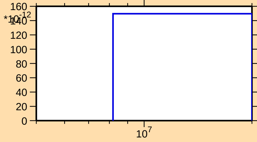
\sigma vs. E for ^{208}\text{Tl}(n,2n\alpha)
