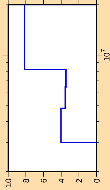
\Delta\sigma/\sigma vs. E for ^{208}\text{Tl}(n,2n)
