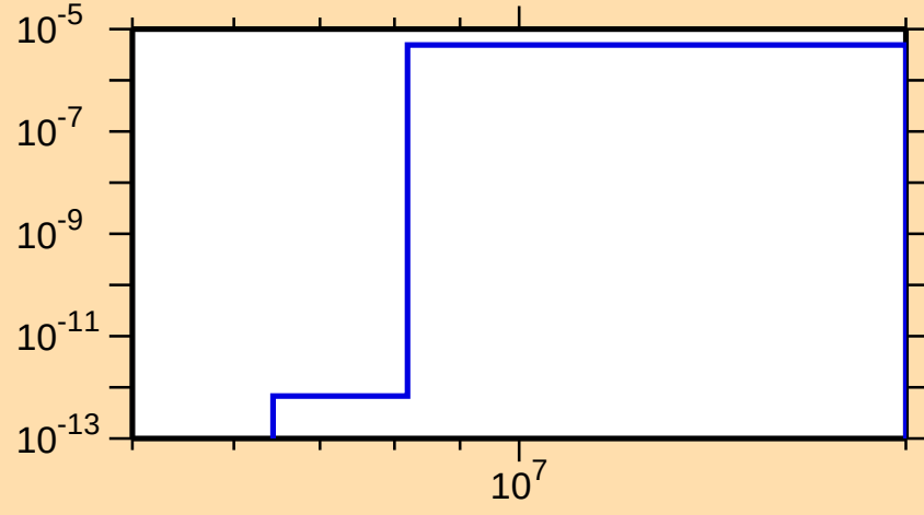
\sigma vs. E for ^{208}\text{Tl}(n,n\alpha)
