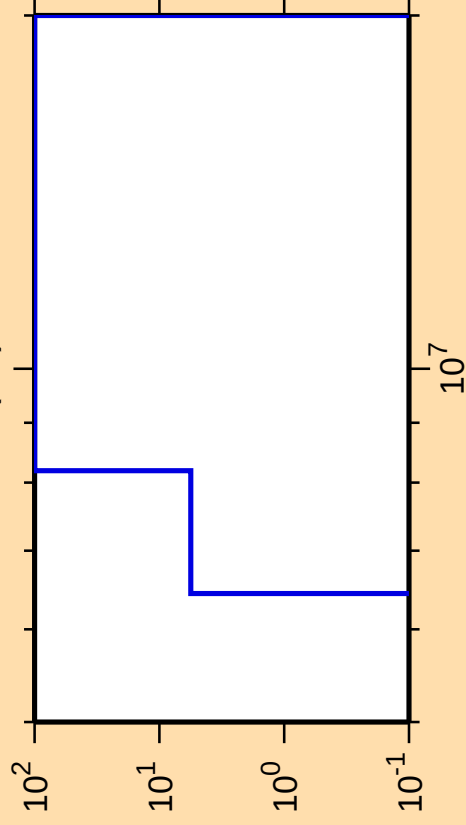
\Delta\sigma/\sigma vs. E for ^{208}\text{Tl}(n,t)
