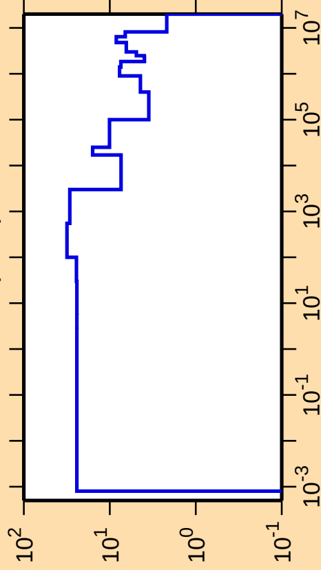
\Delta\sigma/\sigma vs. E for ^{208}\text{Tl}(n,\text{el.})
