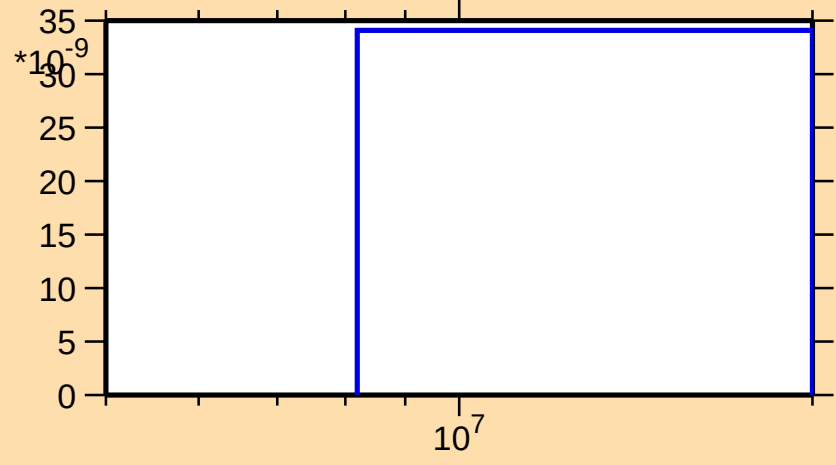
\sigma vs. E for ^{208}\text{Tl}(n,\text{nt})
