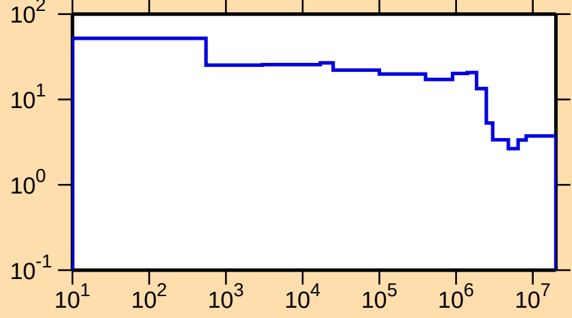
\Delta\sigma/\sigma vs. E for ^{208}\text{Tl}(n,\text{nonel.})
