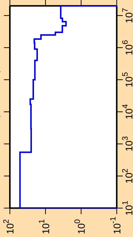
\Delta\sigma/\sigma vs. E for ^{208}\text{Tl}(n,\text{nonel.})
