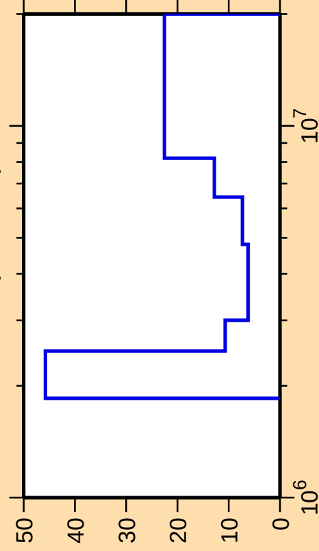
\Delta\sigma/\sigma vs. E for ^{208}\text{Tl}(n,n\text{cont.})
