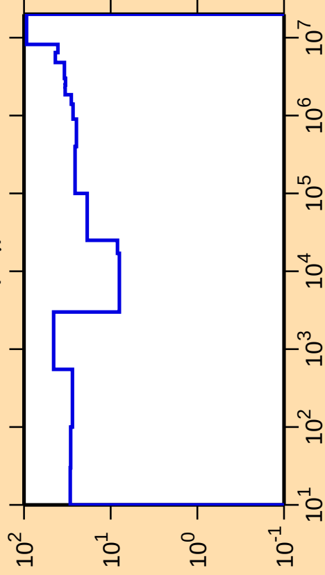
\Delta\sigma/\sigma vs. E for ^{208}\text{Tl}(n,\gamma)
