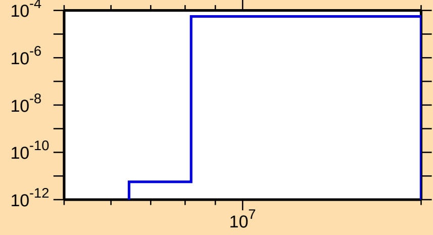
\sigma vs. E for ^{208}\text{Tl}(n,t)
