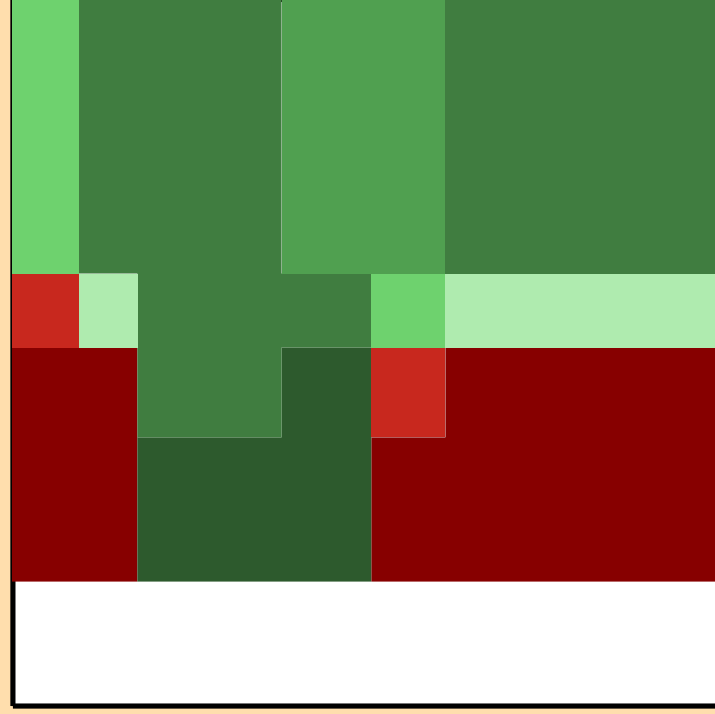
\Delta\sigma/\sigma vs. E for ^{208}\text{Tl}(n,\text{nonel.})
