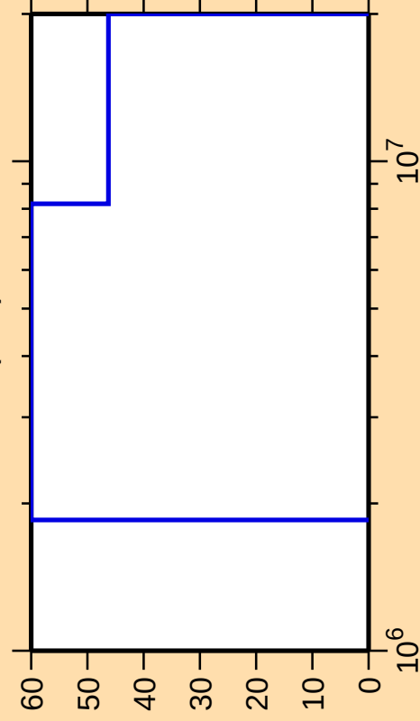
\Delta\sigma/\sigma vs. E for ^{208}\text{Tl}(n,\alpha)
