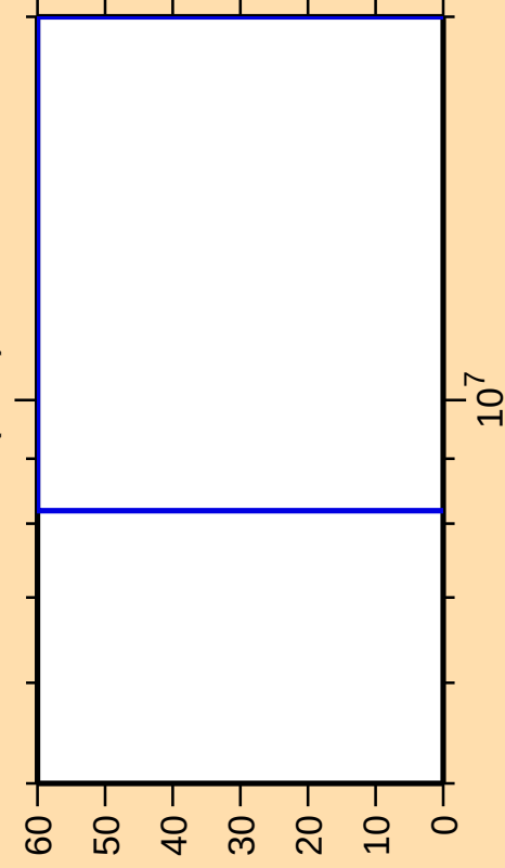
\Delta\sigma/\sigma vs. E for ^{208}\text{Tl}(n,\text{nt})
