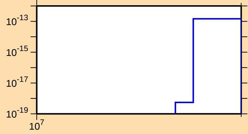
\sigma vs. E for ^{209}\text{Tl}(\text{mt 42})
