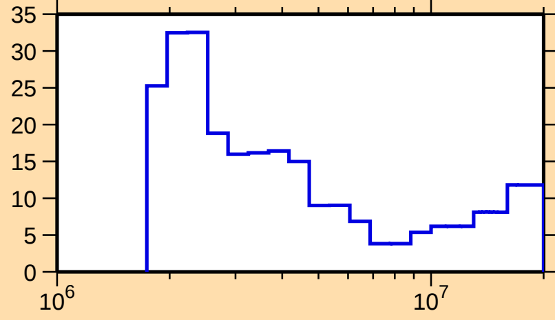
\Delta\sigma/\sigma vs. E for ^{209}\text{Tl}(n,n_1)
