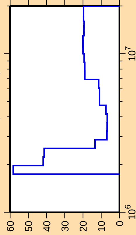
\Delta\sigma/\sigma vs. E for ^{209}\text{Tl}(n,\text{ncont.})
