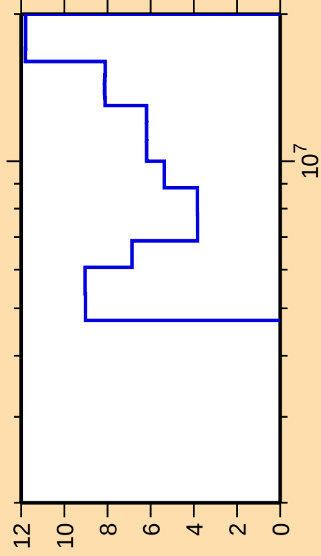
\Delta\sigma/\sigma vs. E for ^{209}\text{Tl}(n,n_1)
