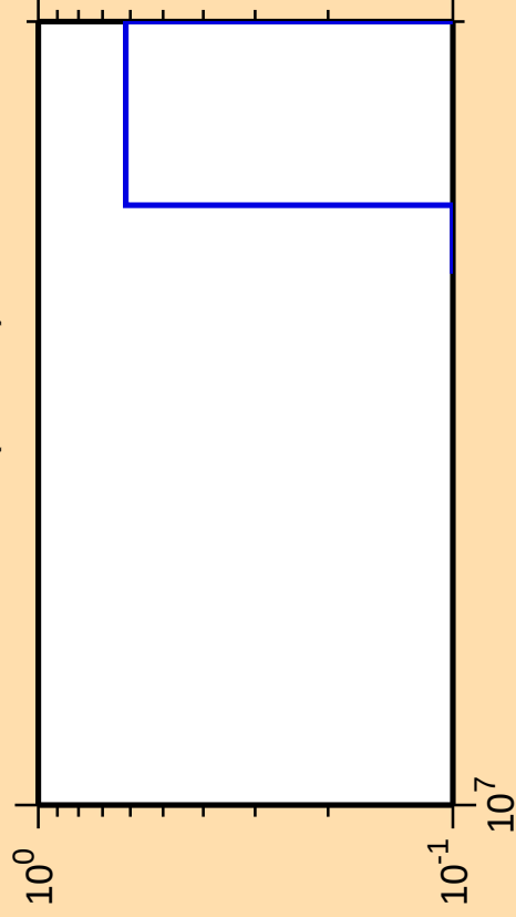
\Delta\sigma/\sigma vs. E for ^{209}\text{Tl}(n,3n\alpha)
