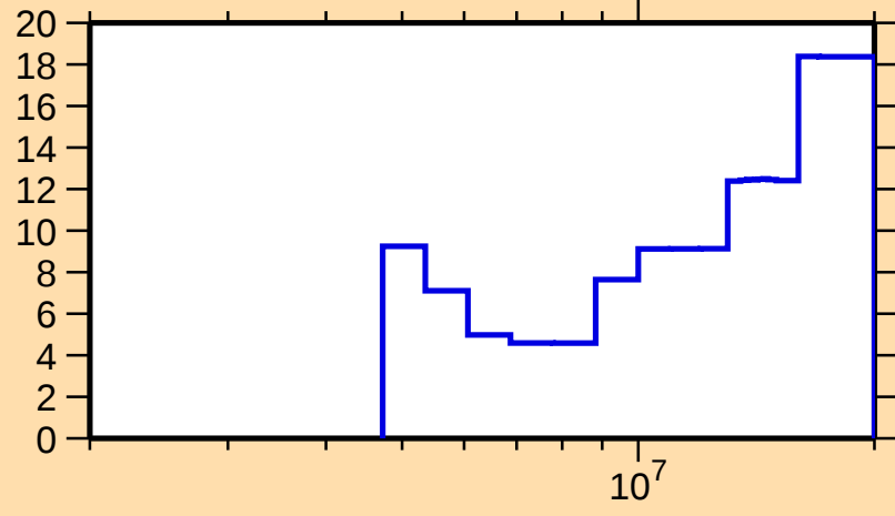
\Delta\sigma/\sigma vs. E for ^{209}\text{Tl}(n,2n)
