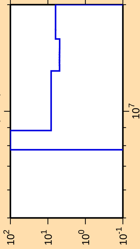
\Delta\sigma/\sigma vs. E for ^{209}\text{Tl}(n,3n)
