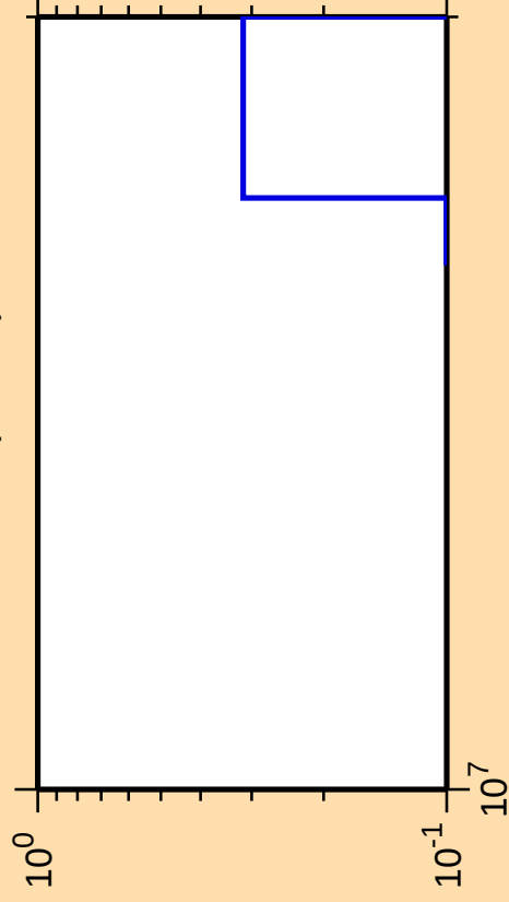
\Delta\sigma/\sigma vs. E for ^{209}\text{Tl}(\text{mt 42})
