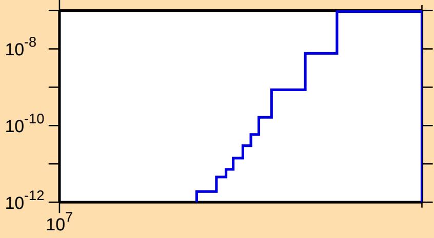
\sigma vs. E for ^{209}\text{Tl}(n,2n\alpha)
