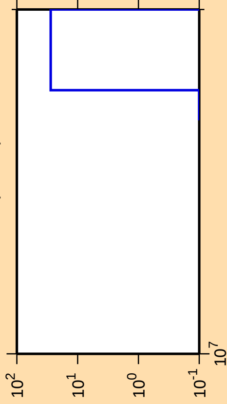
\Delta\sigma/\sigma vs. E for ^{209}\text{Tl}(\text{mt 11})
