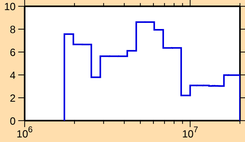
\Delta\sigma/\sigma vs. E for ^{209}\text{Tl}(n,\text{el.})
