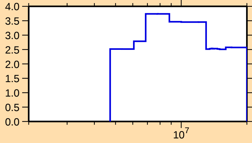
\Delta\sigma/\sigma vs. E for ^{209}\text{Tl}(n,\text{nonel.})
