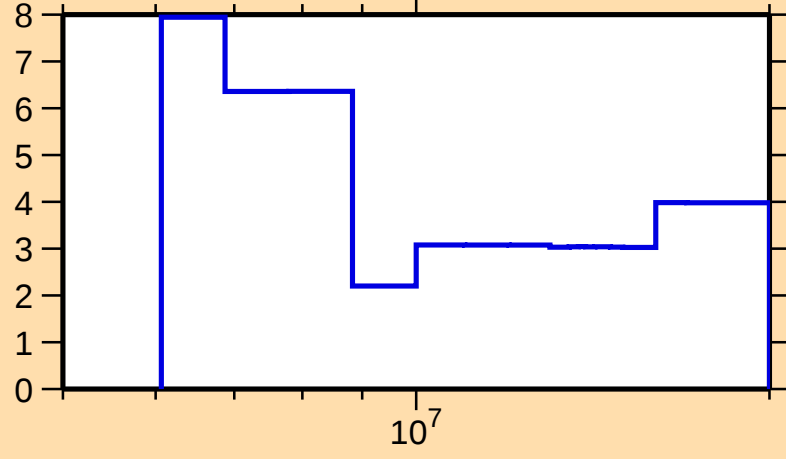
\Delta\sigma/\sigma vs. E for ^{209}\text{Tl}(n,\text{el.})
