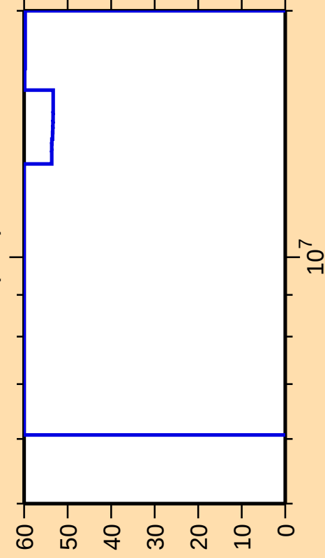
\Delta\sigma/\sigma vs. E for ^{209}\text{Tl}(n,\alpha)
