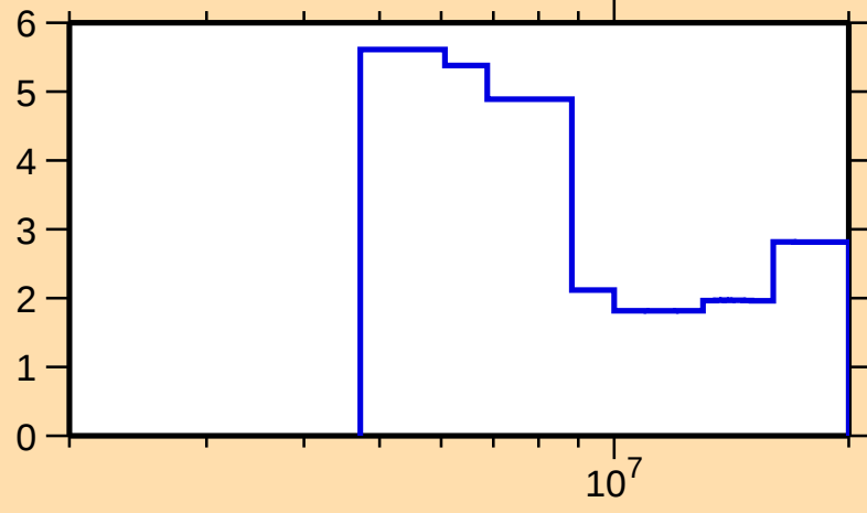
\Delta\sigma/\sigma vs. E for ^{209}\text{Tl}(n,\text{tot.})
