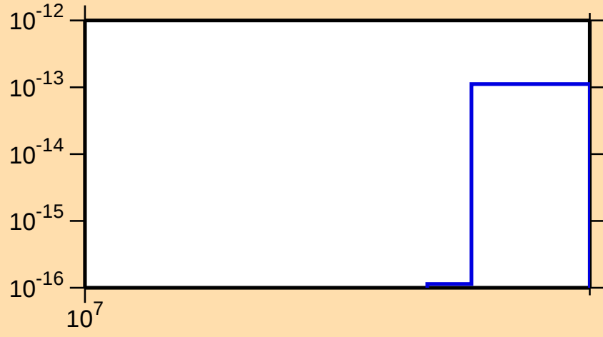
\sigma vs. E for ^{209}\text{Tl}(n,3n\alpha)
