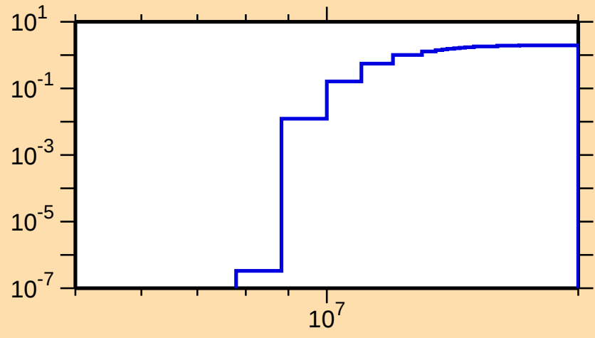
\sigma vs. E for ^{209}\text{Tl}(n,3n)
