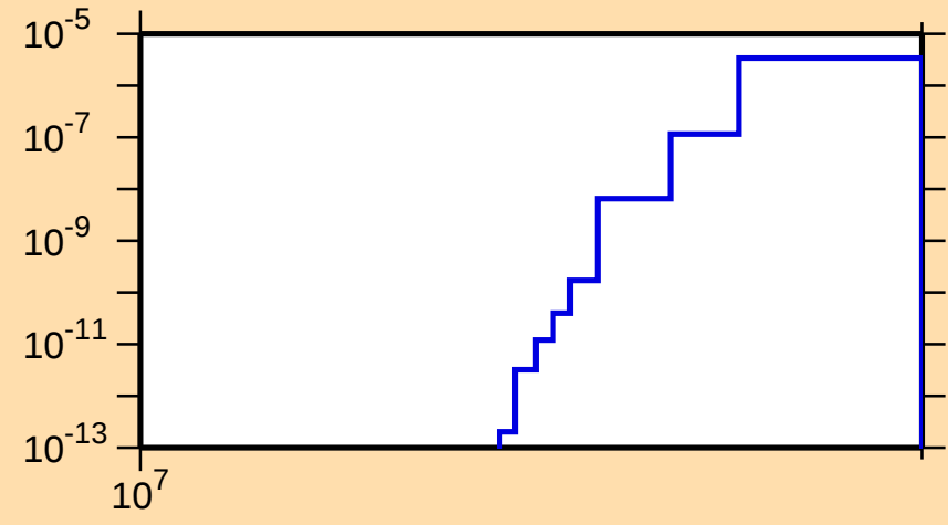
\sigma vs. E for ^{209}\text{Tl}(n,\text{nd})
