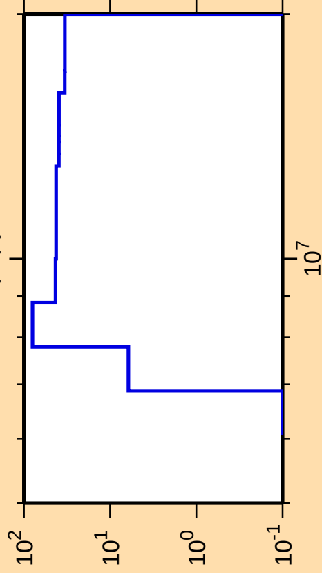
\Delta\sigma/\sigma vs. E for ^{209}\text{Tl}(n,p)
