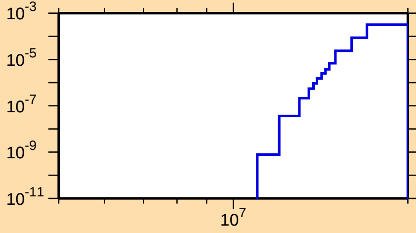
\sigma vs. E for ^{209}\text{Tl}(n,np)
