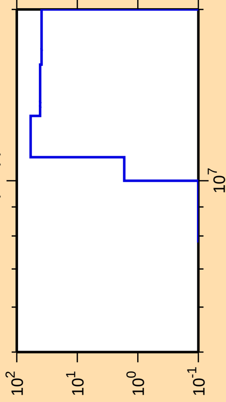
\Delta\sigma/\sigma vs. E for ^{209}\text{Tl}(n,np)
