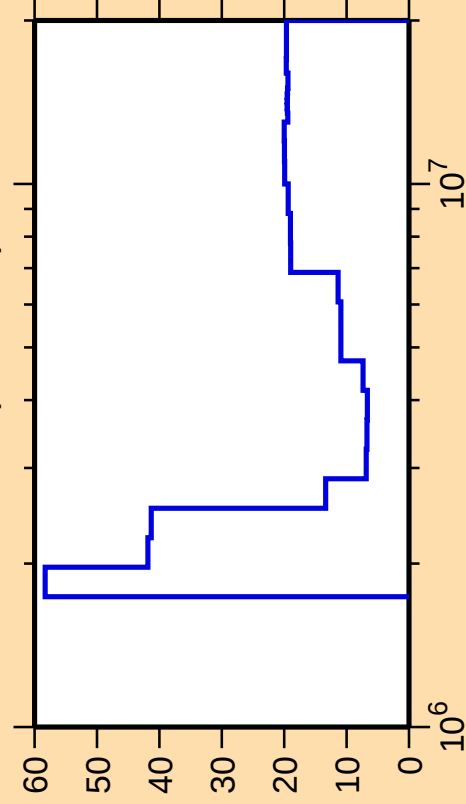
\Delta\sigma/\sigma vs. E for ^{209}\text{Tl}(n,n\text{cont.})
