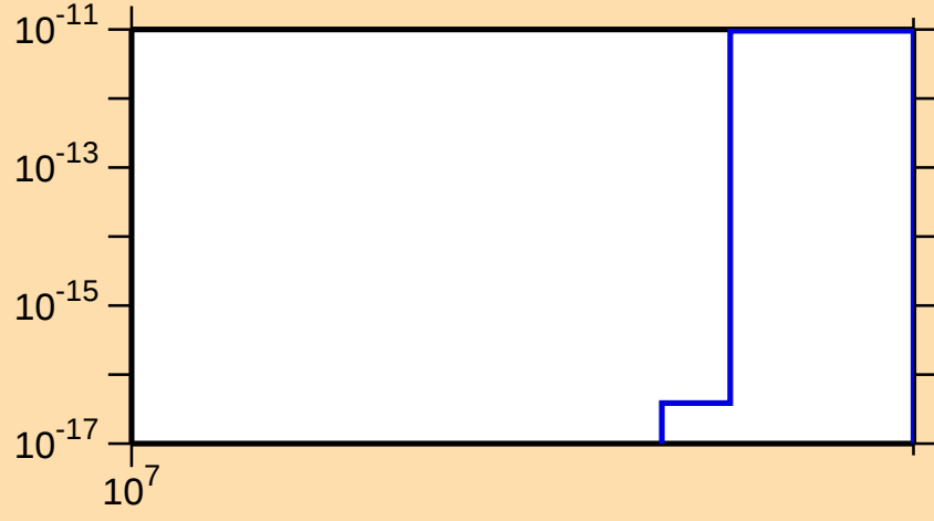
\sigma vs. E for ^{209}\text{Tl}(\text{mt 11})
