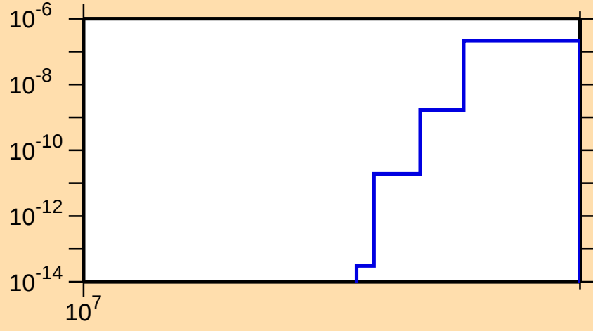
\sigma vs. E for ^{209}\text{Tl}(n,2np)
