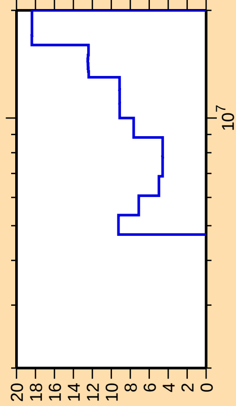
\Delta\sigma/\sigma vs. E for ^{209}\text{Tl}(n,2n)
