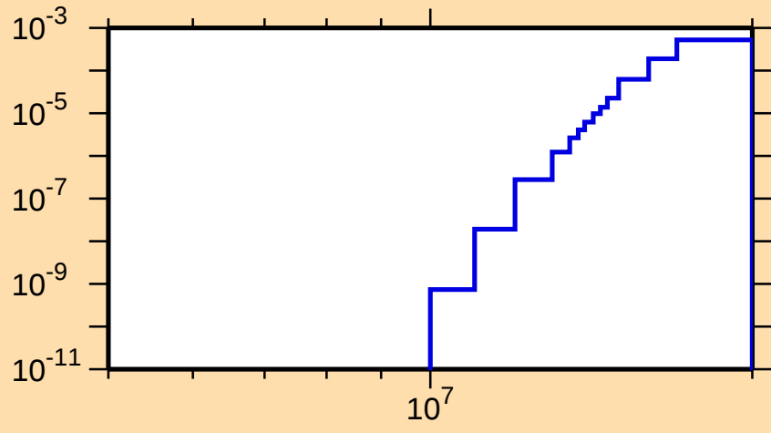
\sigma vs. E for ^{209}\text{Tl}(n,d)
