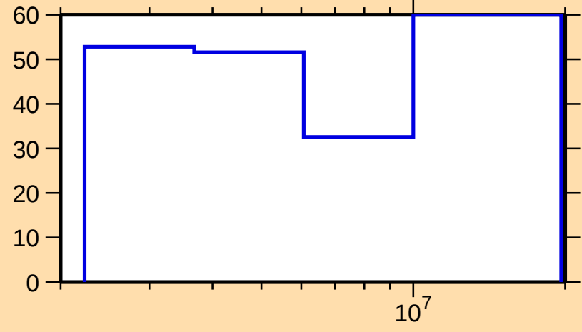
\Delta\sigma/\sigma vs. E for ^{209}\text{Tl}(n,\gamma)
