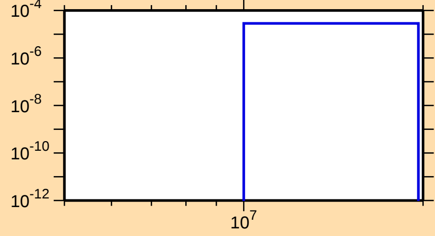
\sigma vs. E for ^{209}\text{Tl}(n,d)
