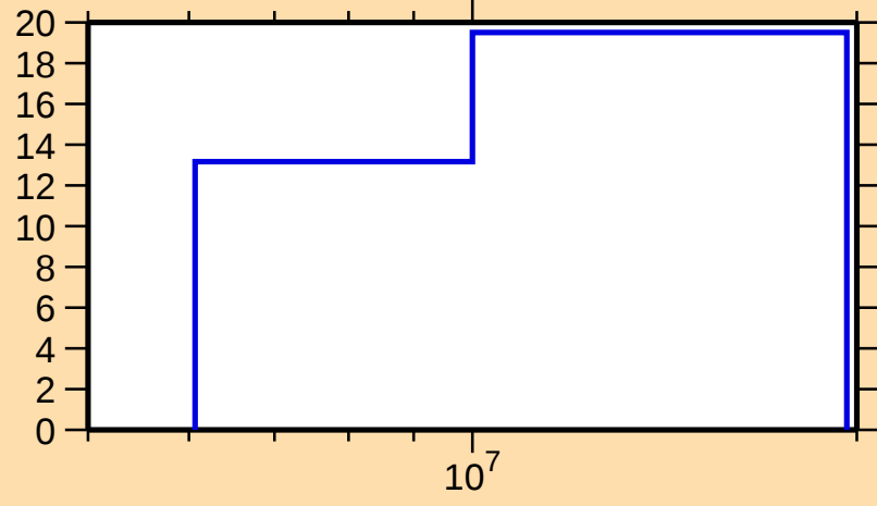
\Delta\sigma/\sigma vs. E for ^{209}\text{Tl}(n,n\text{cont.})
