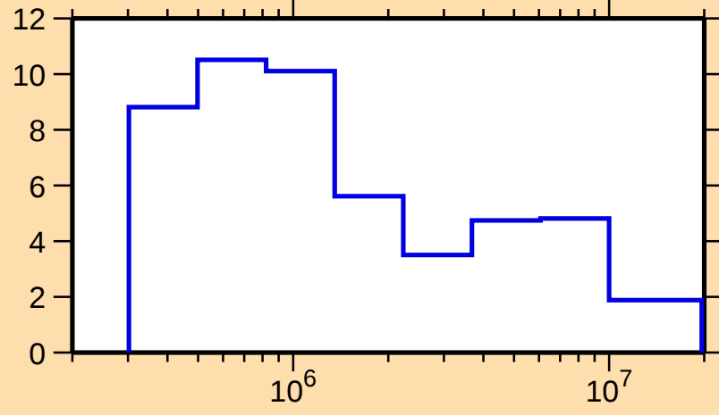
\Delta\sigma/\sigma vs. E for ^{209}\text{Tl}(n,\text{tot.})
