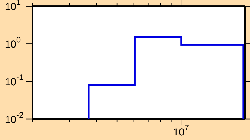
\sigma vs. E for ^{209}\text{Tl}(n,2n)
