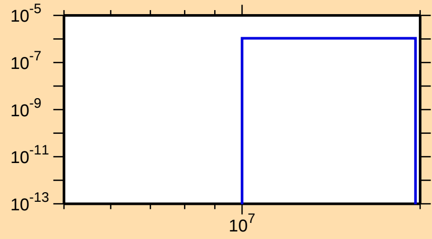
\sigma vs. E for ^{209}\text{Tl}(n,\text{nt})
