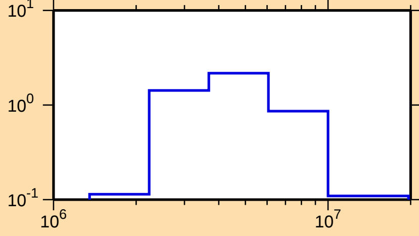
\sigma vs. E for ^{209}\text{Tl}(n,n\text{cont.})
