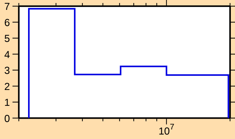
\Delta\sigma/\sigma vs. E for ^{209}\text{Tl}(n,\text{nonel.})
