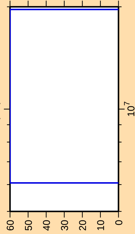
\Delta\sigma/\sigma vs. E for ^{209}\text{Tl}(n,t)
