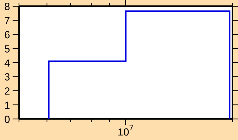
\Delta\sigma/\sigma vs. E for ^{209}\text{Tl}(n,n_1)
