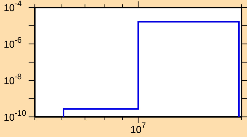
\sigma vs. E for ^{209}\text{Tl}(n,n\alpha)
