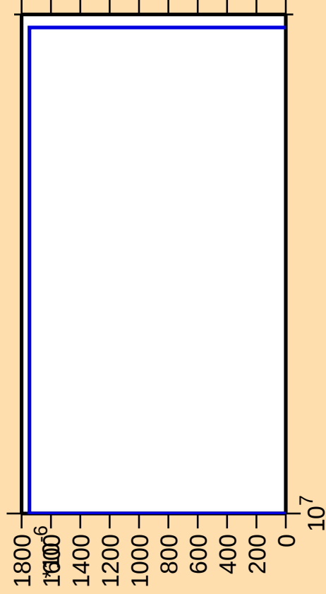
\Delta\sigma/\sigma vs. E for ^{209}\text{Tl}(\text{mt } 42)
