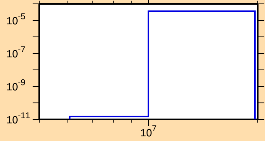
\sigma vs. E for ^{209}\text{Tl}(n,t)
