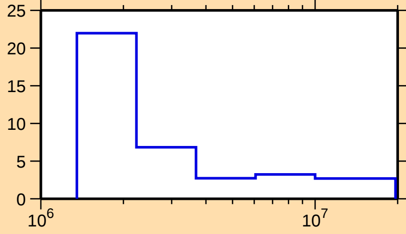
\Delta\sigma/\sigma vs. E for ^{209}\text{Tl}(n,n\text{nonel.})
