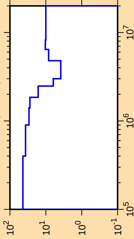
\Delta\sigma/\sigma vs. E for ^{209}\text{Tl}(n,\text{inel.})
