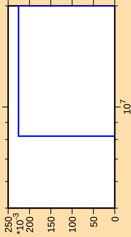
\Delta\sigma/\sigma vs. E for ^{209}\text{Tl}(\text{mt 11})
