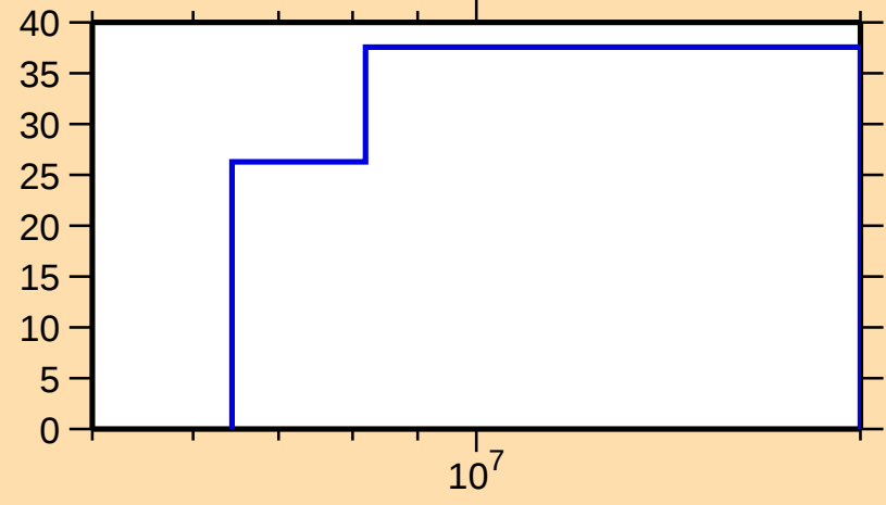
\Delta\sigma/\sigma vs. E for ^{209}\text{Tl}(n,p)
