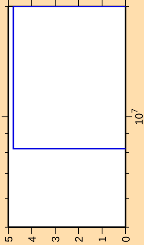
\Delta\sigma/\sigma vs. E for ^{209}\text{Tl}(n,3n)
