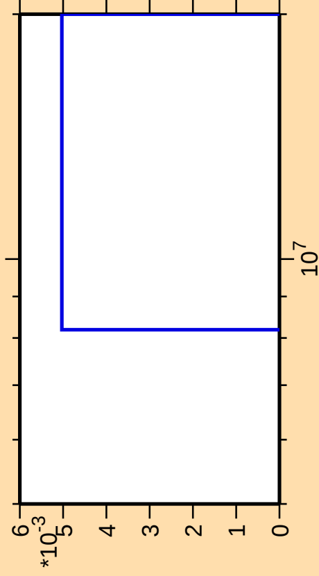
\Delta\sigma/\sigma vs. E for ^{209}\text{Tl}(n,3n\alpha)
