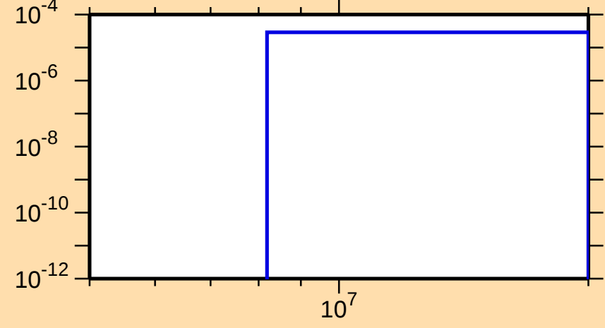
\sigma vs. E for ^{209}\text{Tl}(n,t)
