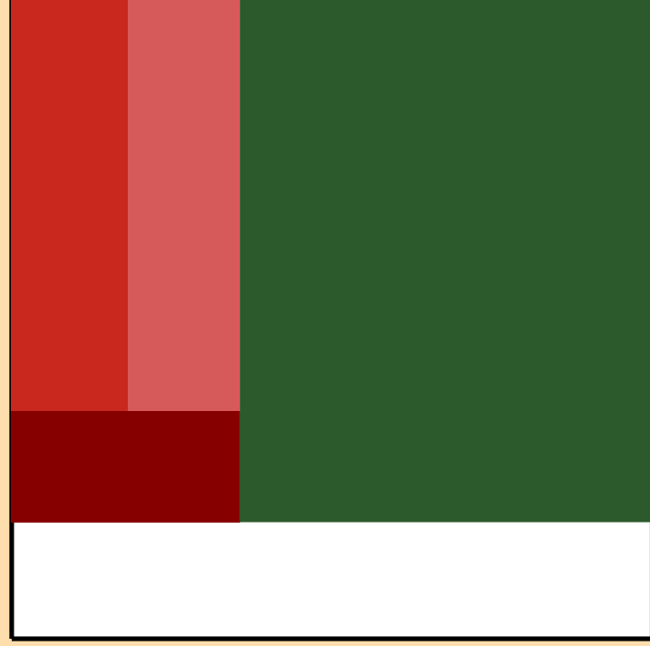
\Delta\sigma/\sigma vs. E for ^{209}\text{Tl}(n,\gamma)
