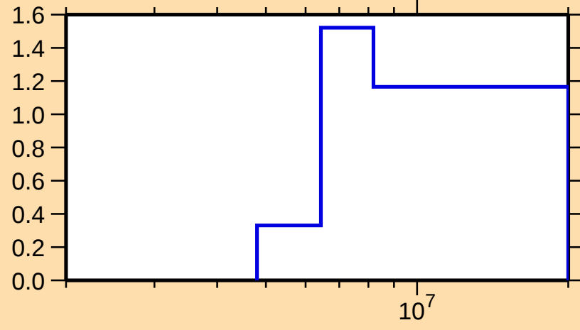
\sigma vs. E for ^{209}\text{Tl}(n,2n)
