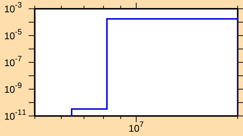
\sigma vs. E for ^{209}\text{Tl}(n,p)
