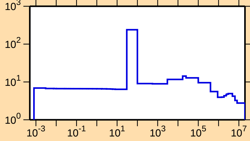
\sigma vs. E for ^{209}\text{Tl}(n,\text{el.})
