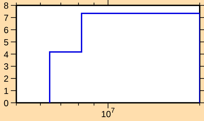
\Delta\sigma/\sigma vs. E for ^{209}\text{Tl}(n,2n)
