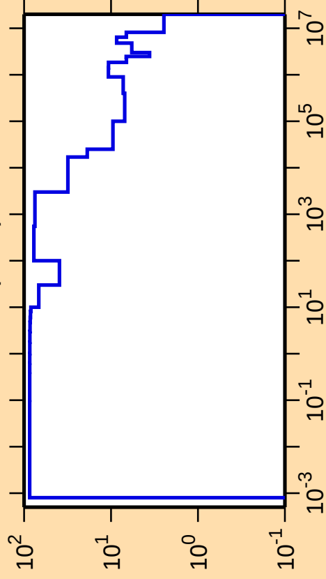
\Delta\sigma/\sigma vs. E for ^{209}\text{Tl}(n,\text{el.})
