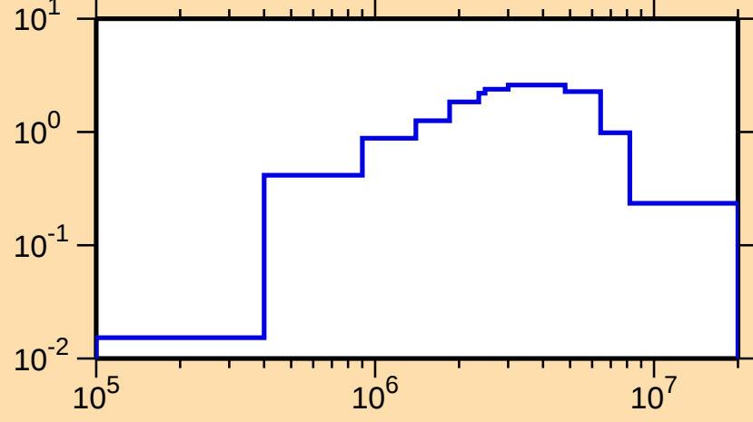
\sigma vs. E for ^{209}\text{Tl}(n,\text{inel.})
