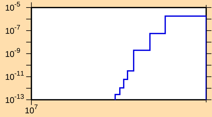
\sigma vs. E for ^{211}\text{Tl}(n,\text{nd})
