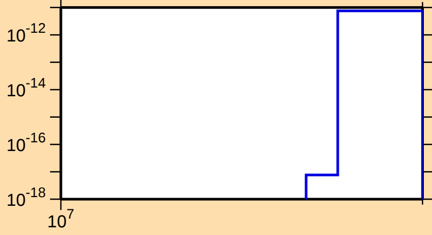
\sigma vs. E for ^{211}\text{Tl}(\text{mt } 11)
