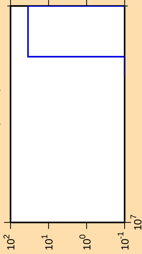
\Delta\sigma/\sigma vs. E for ^{211}\text{Tl}(\text{mt } 11)
