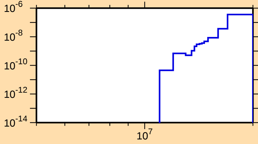
\sigma vs. E for ^{211}\text{Tl}(n,2n\alpha)
