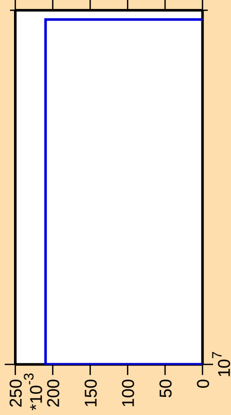
\Delta\sigma/\sigma vs. E for ^{211}\text{Tl} (mt 11)
