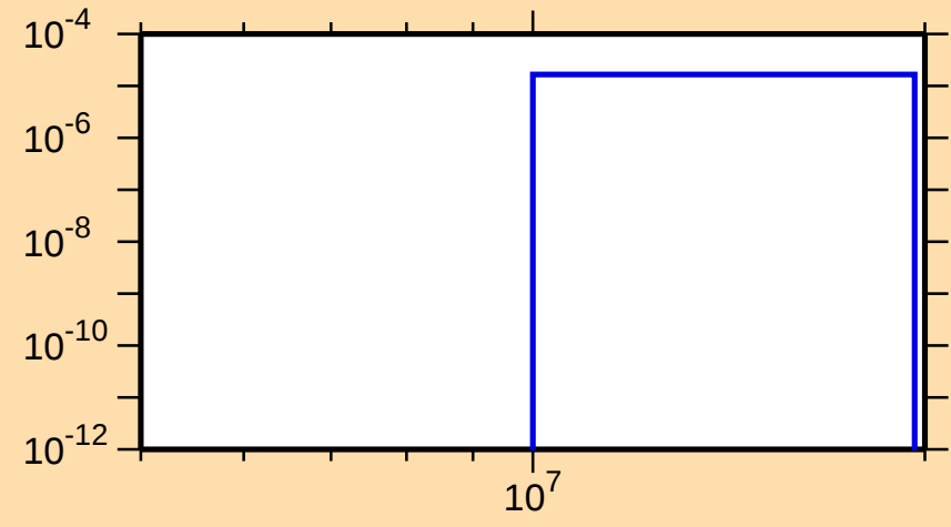
\sigma vs. E for ^{211}\text{Tl}(n,d)
