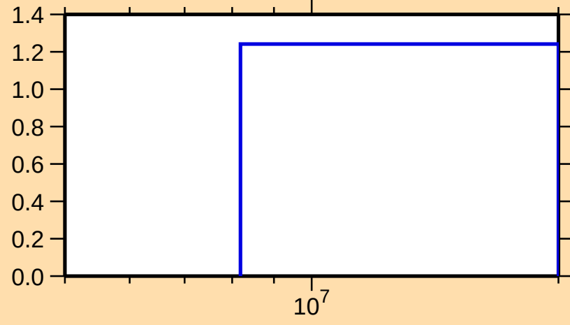
\sigma vs. E for ^{211}\text{Tl}(n,3n)
