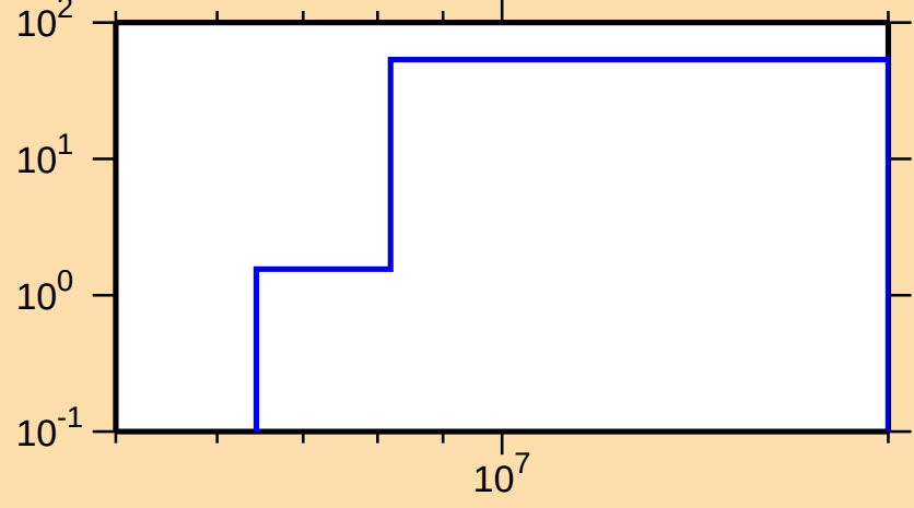
\Delta\sigma/\sigma vs. E for ^{211}\text{Tl}(n,p)
