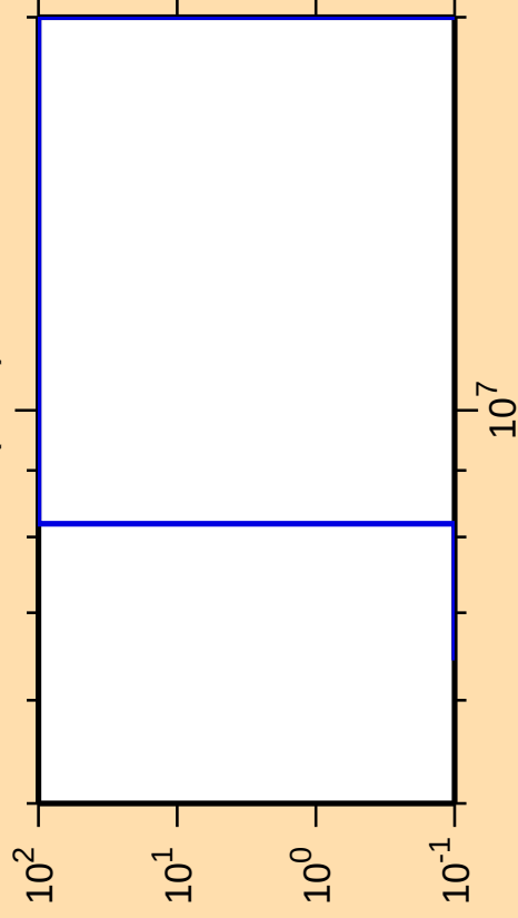
\Delta\sigma/\sigma vs. E for ^{211}\text{Tl}(n,\text{nt})
