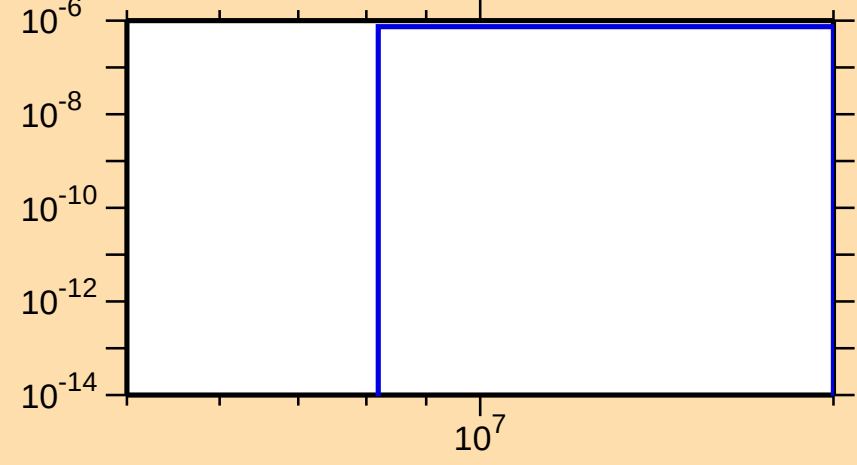
\sigma vs. E for ^{211}\text{Tl}(n,\text{nt})
