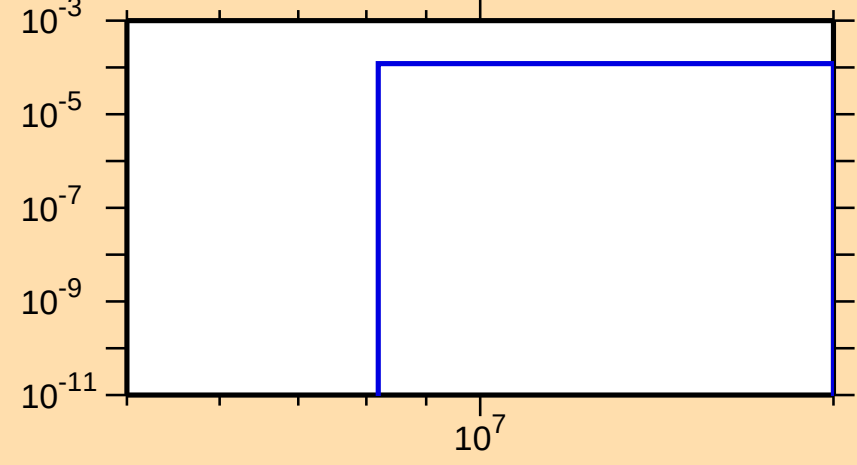
\sigma vs. E for ^{211}\text{Tl}(n,p)
