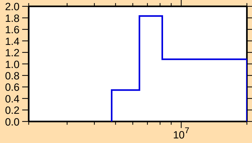
\sigma vs. E for ^{211}\text{Tl}(n,2n)
