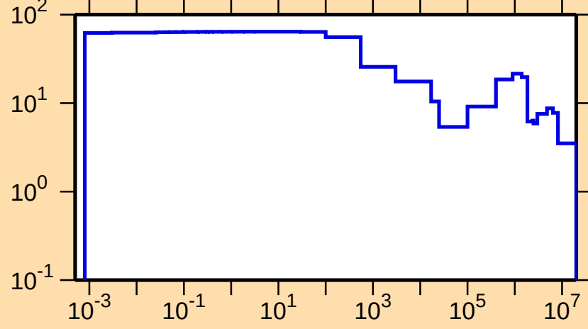
\Delta\sigma/\sigma vs. E for ^{211}\text{Tl}(n,\text{tot.})
