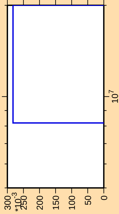
\Delta\sigma/\sigma vs. E for ^{211}\text{Tl}(\text{mt } 11)
