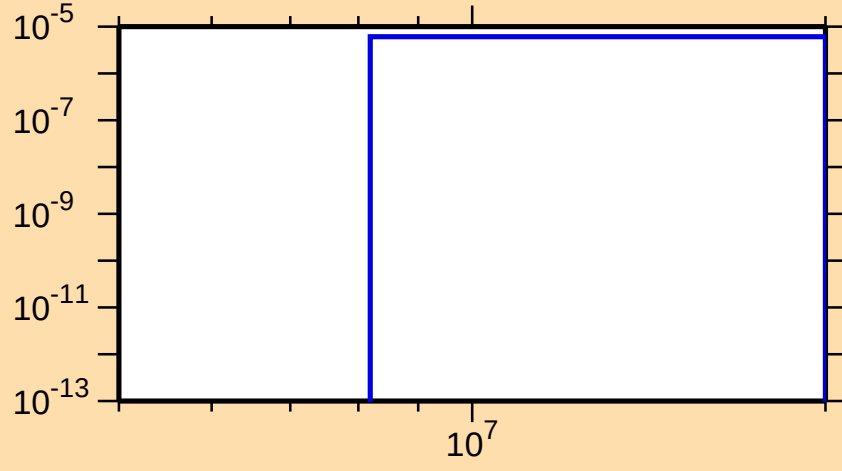
\sigma vs. E for ^{211}\text{Tl}(n,np)
