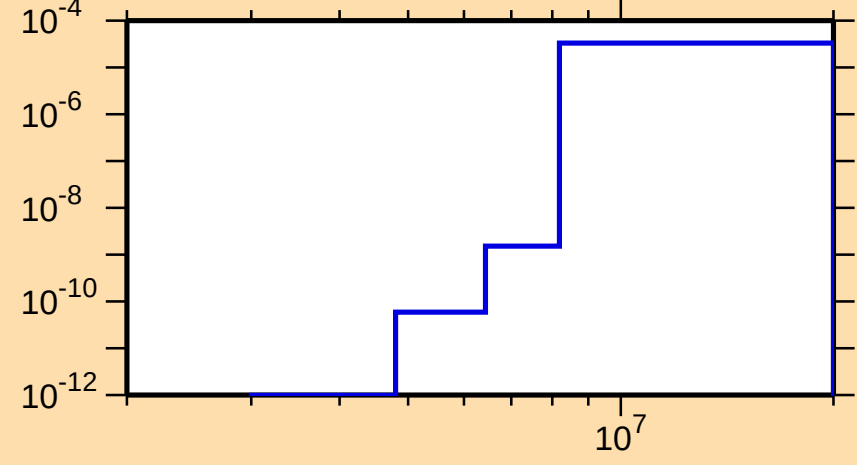
\sigma vs. E for ^{211}\text{Tl}(n,\alpha)
