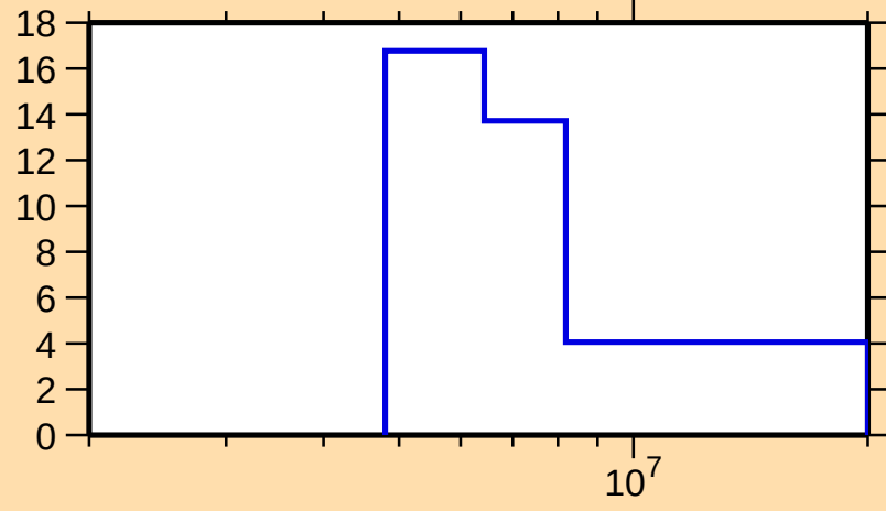
\Delta\sigma/\sigma vs. E for ^{211}\text{Tl}(n,\text{el.})
