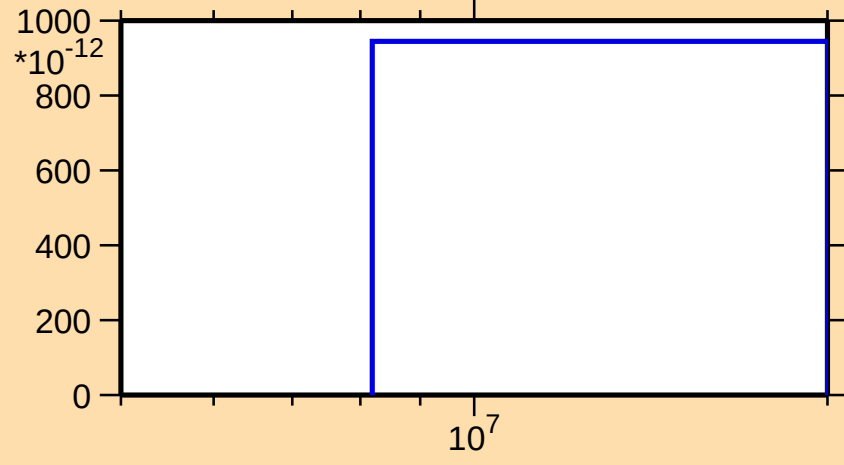
\sigma vs. E for ^{211}\text{Tl}(n,2np)
