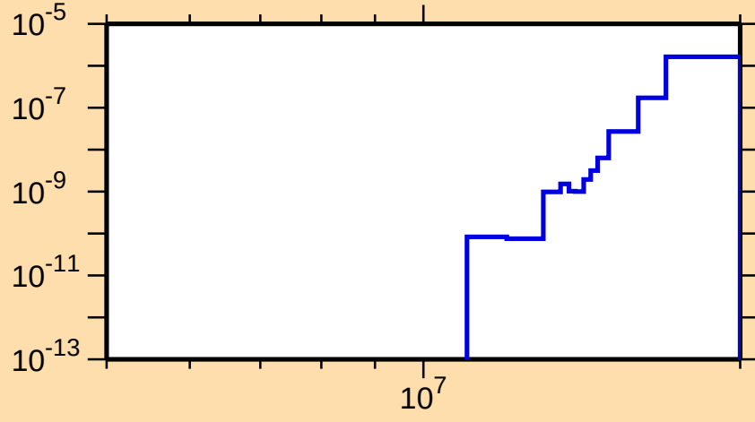
\sigma vs. E for ^{212}\text{Tl}(n,2n\alpha)
