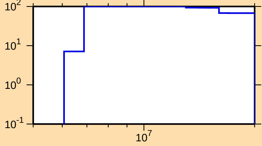
\Delta\sigma/\sigma vs. E for ^{212}\text{Tl}(n,p)
