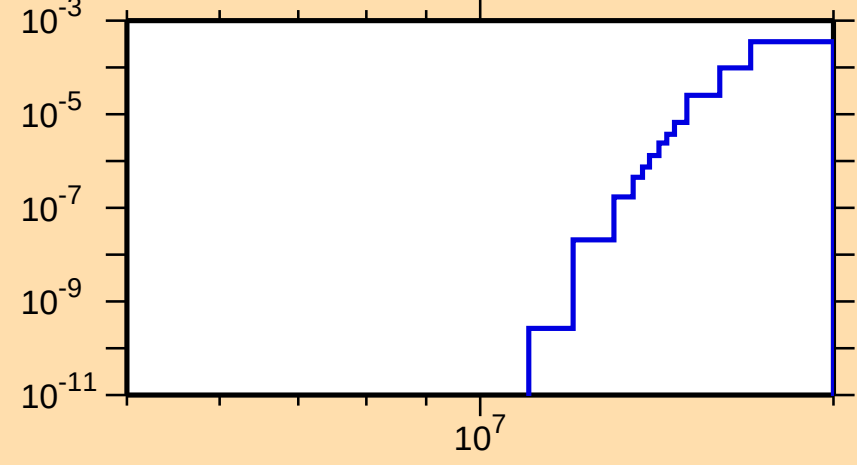
\sigma vs. E for ^{212}\text{Tl}(n,np)
