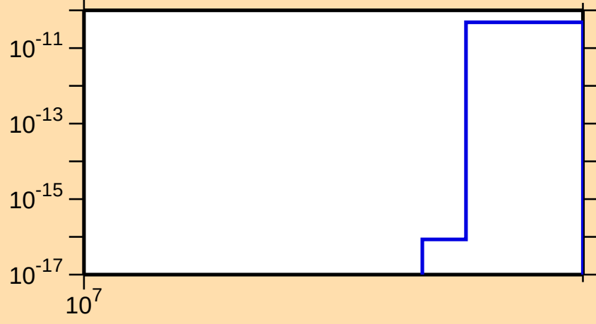
\sigma vs. E for ^{212}\text{Tl}(\text{mt } 11)
