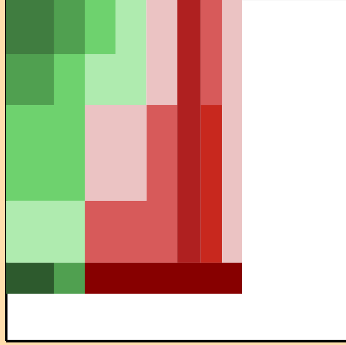
\Delta\sigma/\sigma vs. E for ^{212}\text{Tl}(n,n_1)
