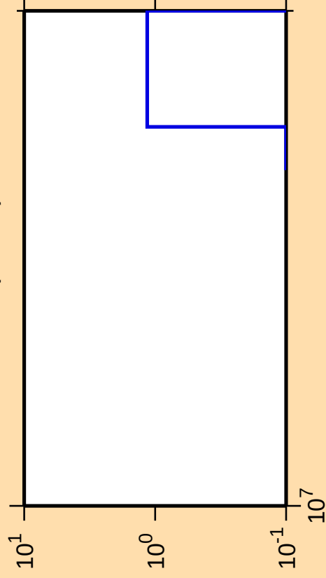
\Delta\sigma/\sigma vs. E for ^{212}\text{Tl}(\text{mt } 42)
