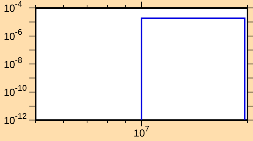
\sigma vs. E for ^{212}\text{Tl}(n,d)
