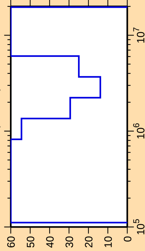
\Delta\sigma/\sigma vs. E for ^{212}\text{Tl}(n,\text{inel.})
