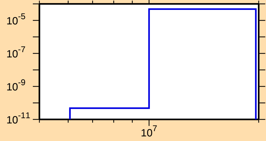
\sigma vs. E for ^{212}\text{Tl}(n,t)
