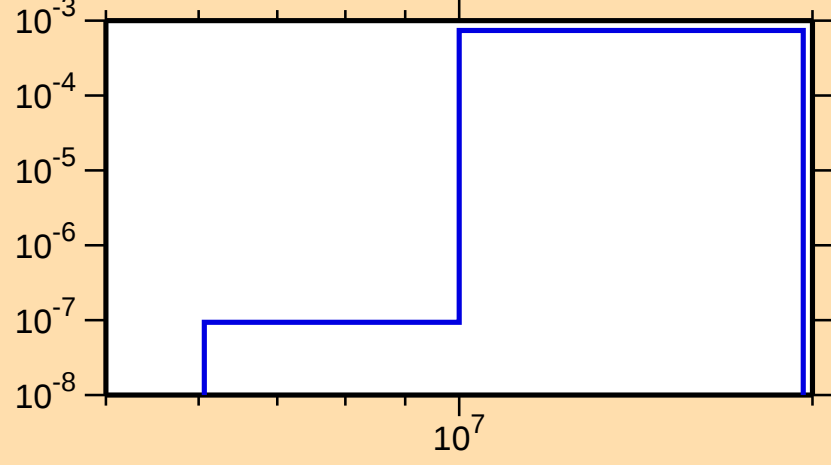
\sigma vs. E for ^{212}\text{Tl}(n,p)
