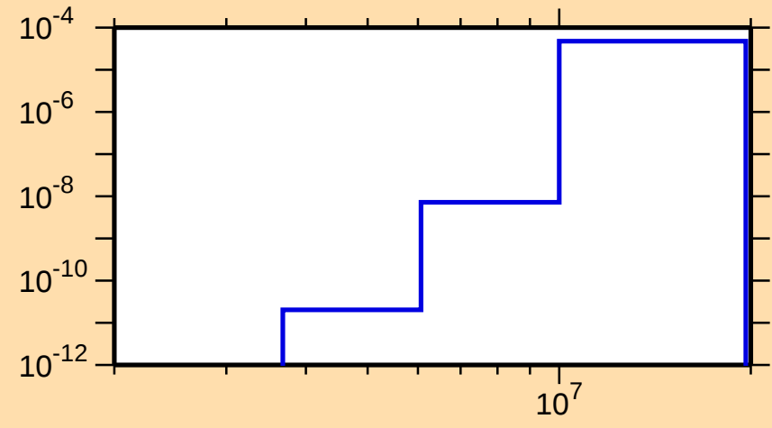
\sigma vs. E for ^{212}\text{Tl}(n,\alpha)
