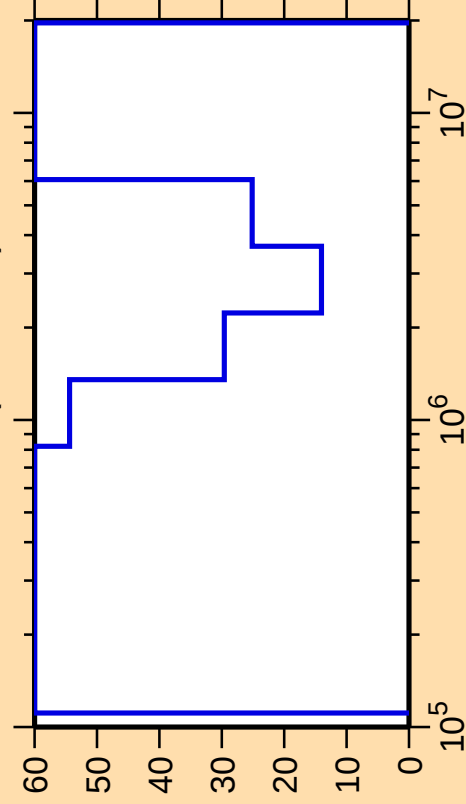
\Delta\sigma/\sigma vs. E for ^{212}\text{Tl}(n,n_{\text{cont}})
