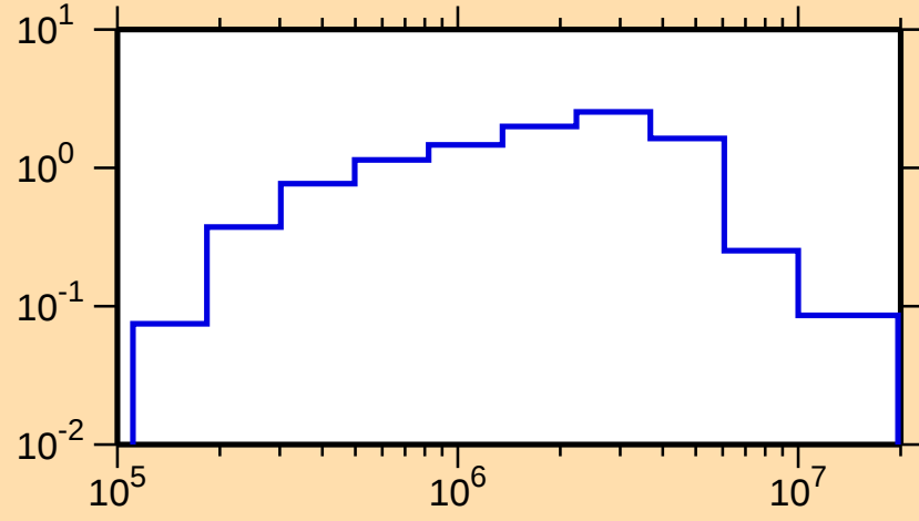
\sigma vs. E for ^{212}\text{Tl}(n,\text{inel.})
