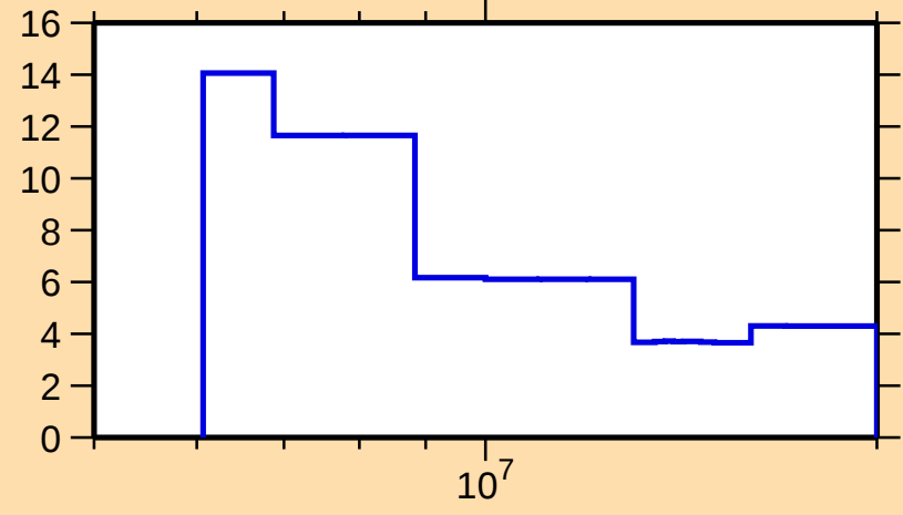
\Delta\sigma/\sigma vs. E for ^{214}\text{Tl}(n,\text{tot.})
