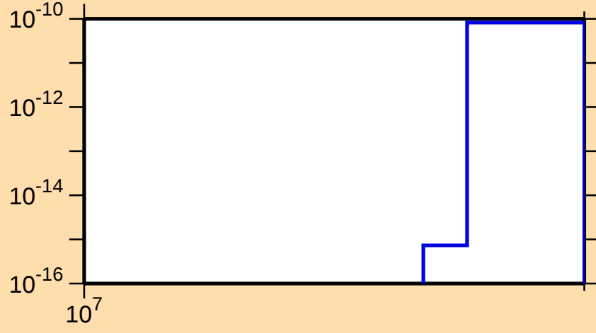
\sigma vs. E for ^{214}\text{Tl}(\text{mt 11})
