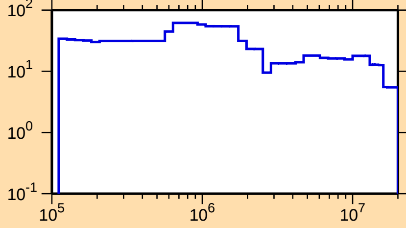
\Delta\sigma/\sigma vs. E for ^{214}\text{Tl}(n,\text{el.})
