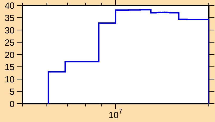
\Delta\sigma/\sigma vs. E for ^{214}\text{Tl}(n,2n)
