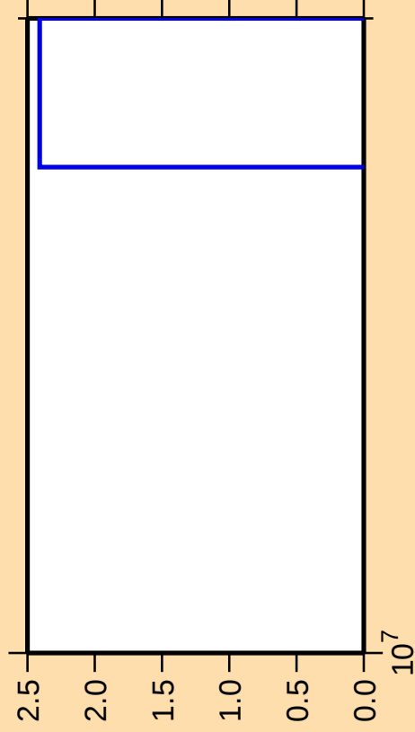
\Delta\sigma/\sigma vs. E for ^{214}\text{Tl}(\text{mt } 42)
