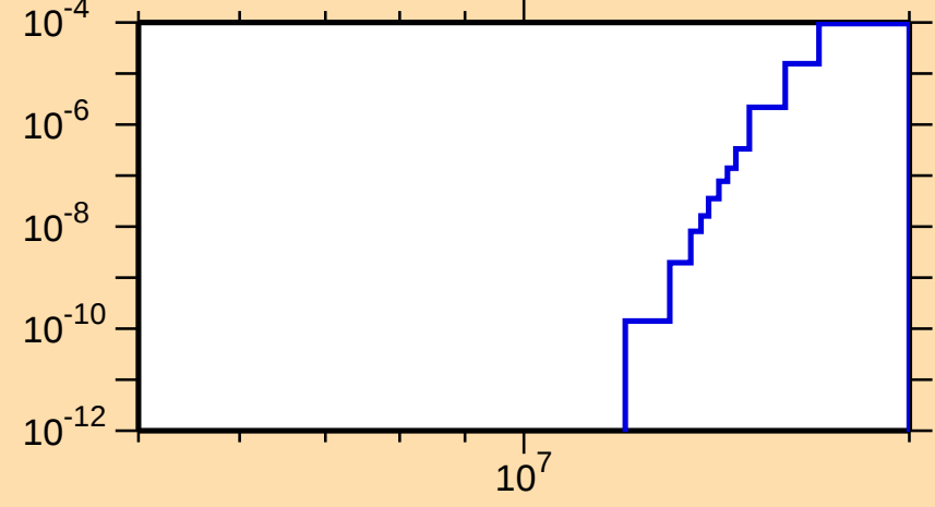
\sigma vs. E for ^{214}\text{Tl}(n,\text{nt})
