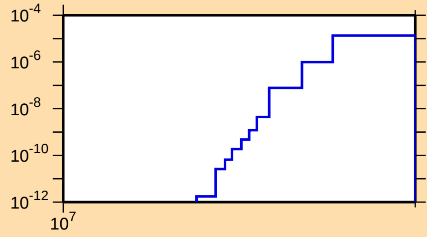
\sigma vs. E for ^{214}\text{Tl}(n,\text{nd})
