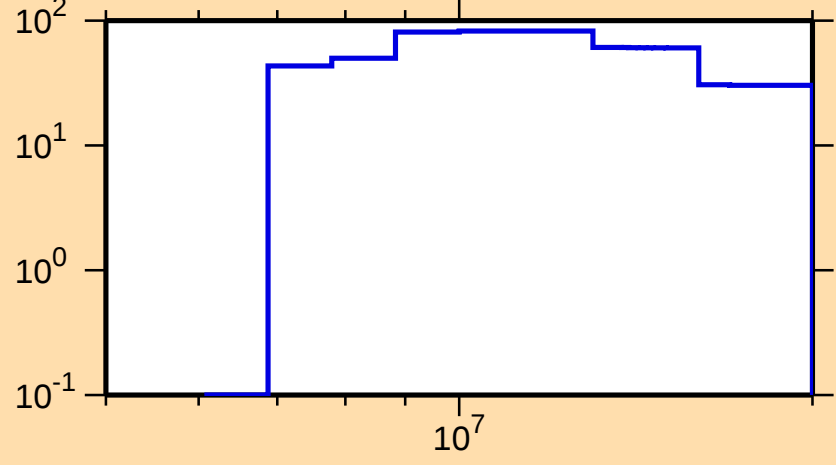
\Delta\sigma/\sigma vs. E for ^{214}\text{Tl}(n,p)
