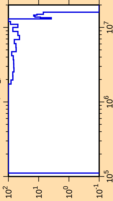
\Delta\sigma/\sigma vs. E for ^{214}\text{Tl}(n,n_1)
