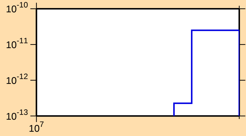
\sigma vs. E for ^{214}\text{Tl}(n,3n\alpha)
