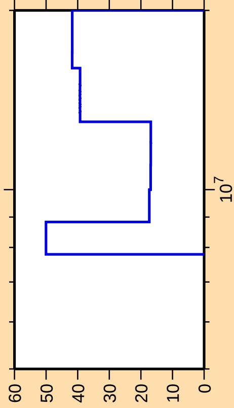
\Delta\sigma/\sigma vs. E for ^{214}\text{Tl}(n,3n)
