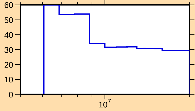
\Delta\sigma/\sigma vs. E for ^{214}\text{Tl}(n,n\text{cont.})
