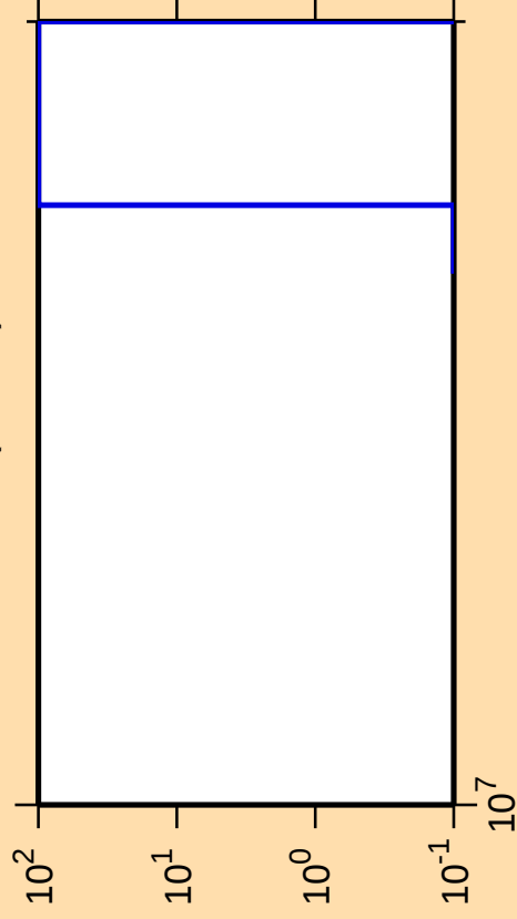
\Delta\sigma/\sigma vs. E for ^{214}\text{Tl}(\text{mt 11})
