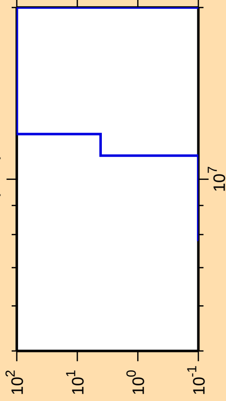
\Delta\sigma/\sigma vs. E for ^{214}\text{Tl}(n,\text{nt})
