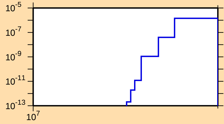
\sigma vs. E for ^{214}\text{Tl}(n,2np)
