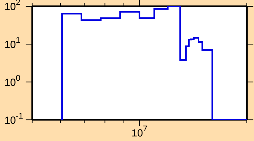
\Delta\sigma/\sigma vs. E for ^{214}\text{Tl}(n,n_1)
