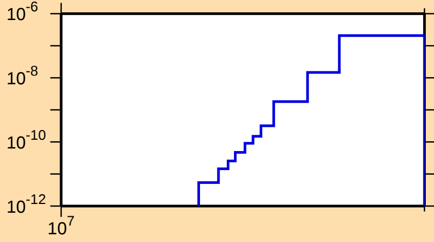
\sigma vs. E for ^{214}\text{Tl}(n,2n\alpha)
