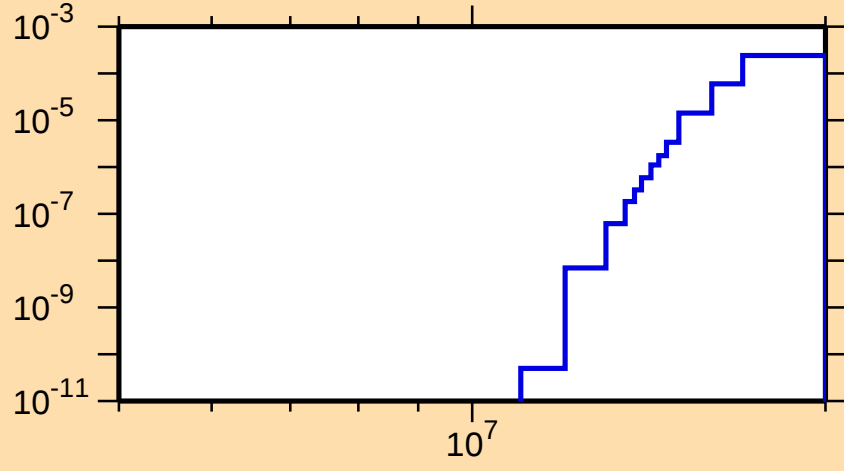
\sigma vs. E for ^{214}\text{Tl}(n,np)
