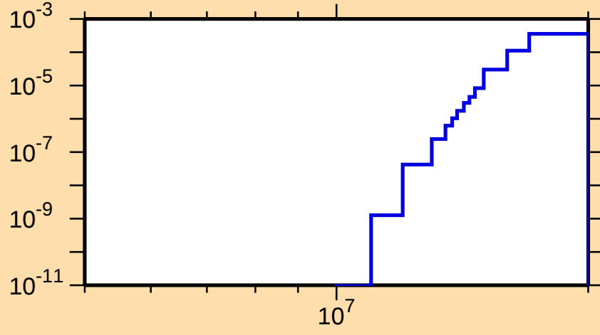
\sigma vs. E for ^{214}\text{Tl}(n,d)
