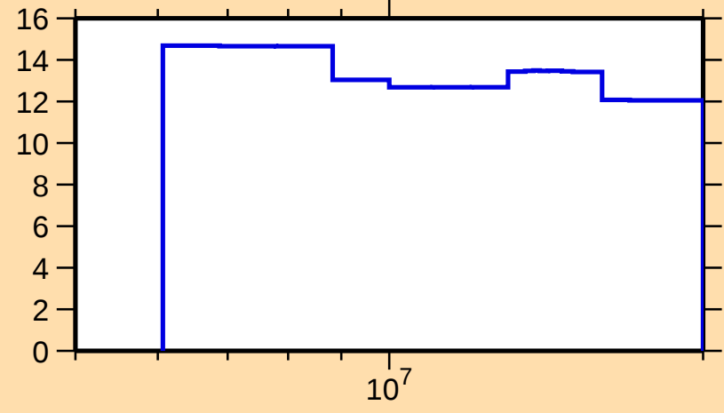
\Delta\sigma/\sigma vs. E for ^{214}\text{Tl}(n,\text{nonel.})
