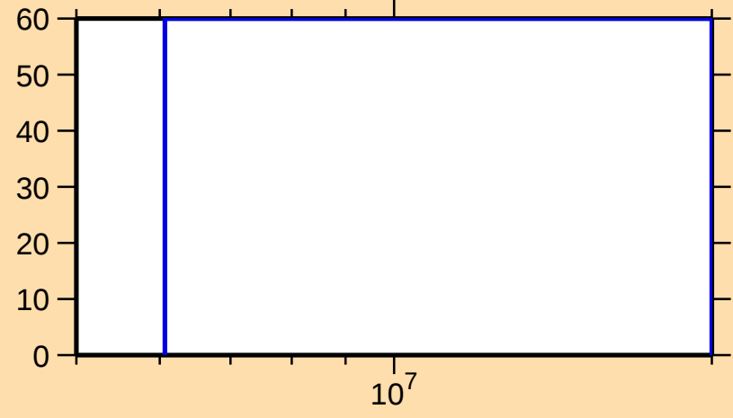
\Delta\sigma/\sigma vs. E for ^{214}\text{Tl}(n,\gamma)
