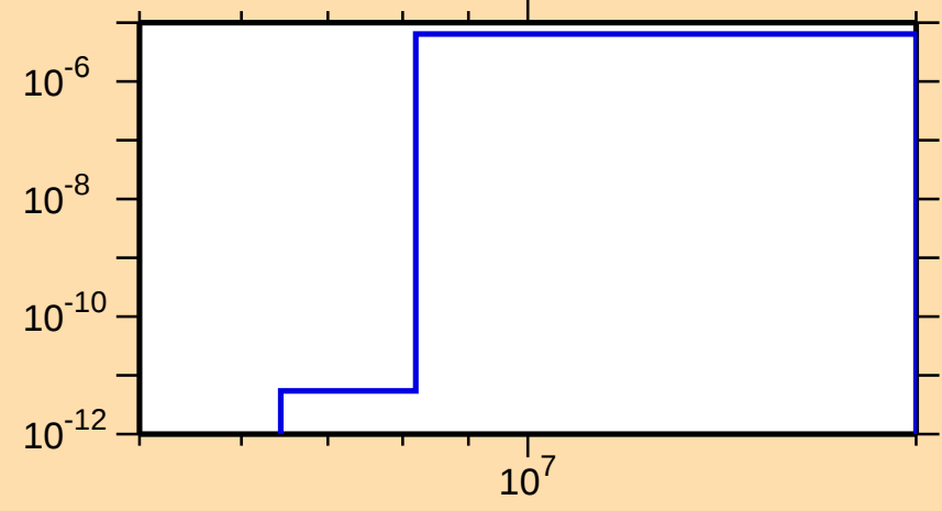
\sigma vs. E for ^{214}\text{Tl}(n,\alpha)
