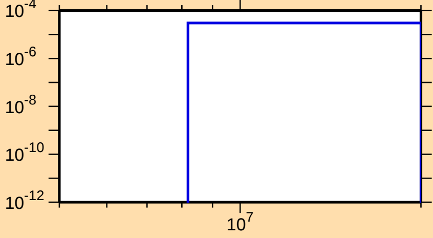
\sigma vs. E for ^{214}\text{Tl}(n,t)
