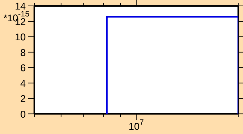
\sigma vs. E for ^{214}\text{Tl}(\text{mt } 42)
