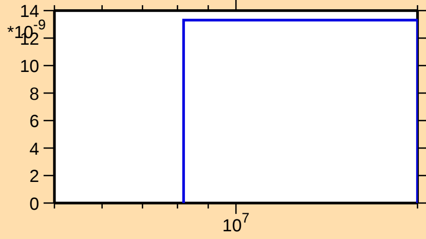
\sigma vs. E for ^{214}\text{Tl}(n,2np)
