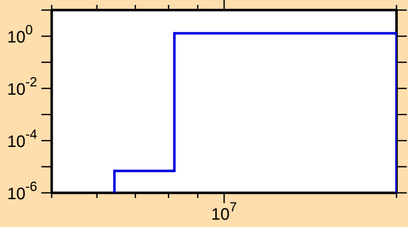
\sigma vs. E for ^{214}\text{Tl}(n,3n)
