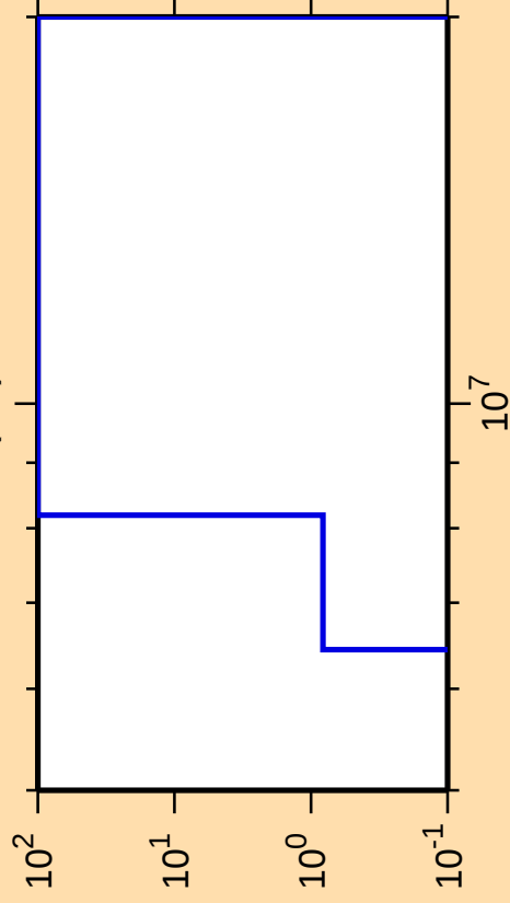
\Delta\sigma/\sigma vs. E for ^{214}\text{Tl}(n,t)
