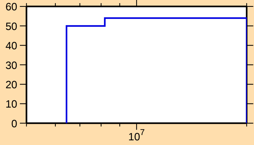
\Delta\sigma/\sigma vs. E for ^{214}\text{Tl}(n,p)
