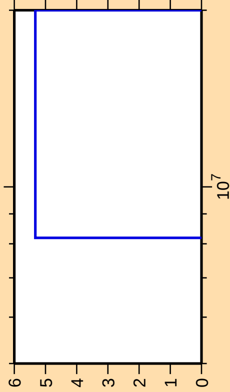
\Delta\sigma/\sigma vs. E for ^{214}\text{Tl}(\text{mt 11})
