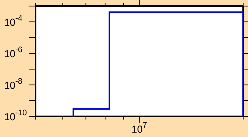
\sigma vs. E for ^{214}\text{Tl}(n,p)
