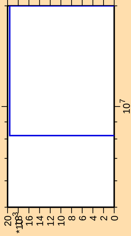
\Delta\sigma/\sigma vs. E for ^{214}\text{Tl}(\text{mt } 42)
