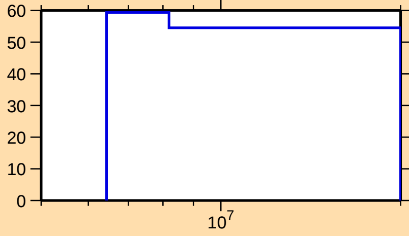
\Delta\sigma/\sigma vs. E for ^{214}\text{Tl}(n,n_1)
