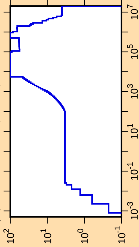
\Delta\mu/\mu vs. E for ^{215}\text{Tl}(\text{mt251})
