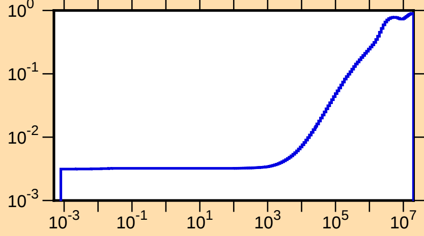
\mu vs. E for ^{215}\text{Tl}(\text{mt251})
