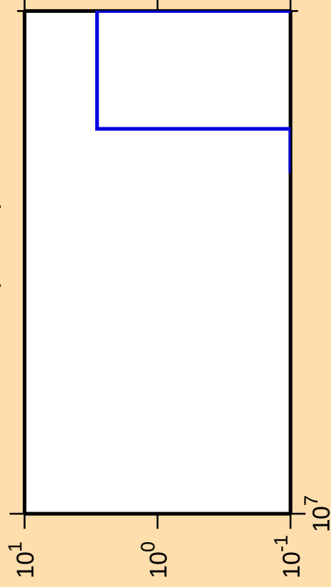
\Delta\sigma/\sigma vs. E for ^{215}\text{Tl}(\text{mt } 42)
