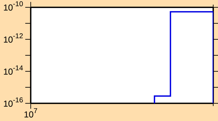
\sigma vs. E for ^{215}\text{Tl}(\text{mt 11})
