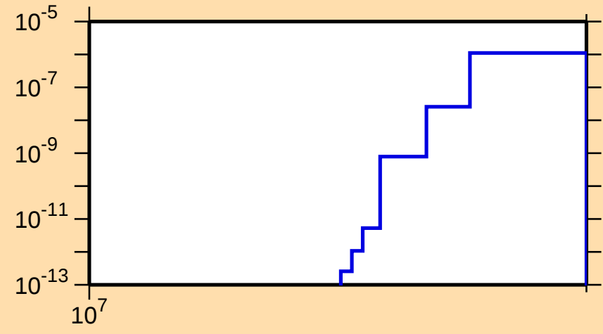
\sigma vs. E for ^{215}\text{Tl}(n,\text{nd})
