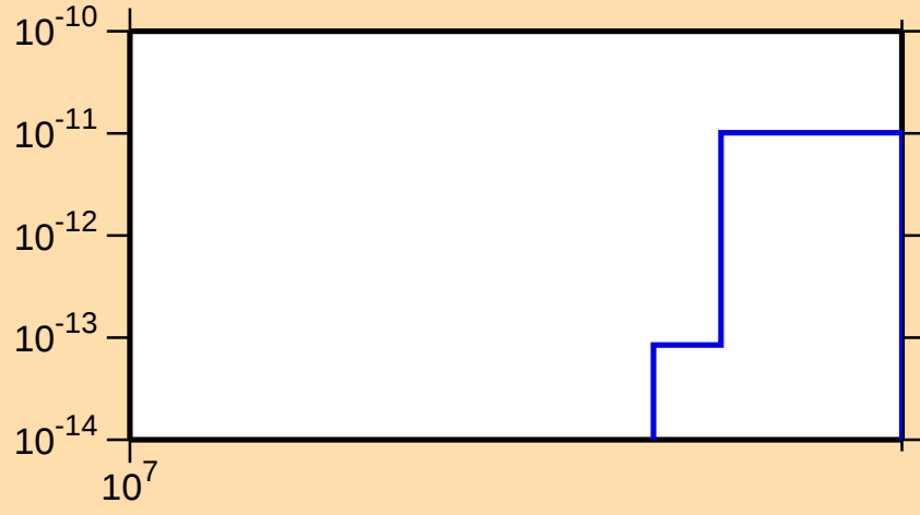
\sigma vs. E for ^{215}\text{Tl}(n,3n\alpha)
