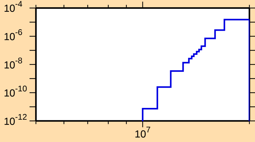
\sigma vs. E for ^{215}\text{Tl}(n,n\alpha)
