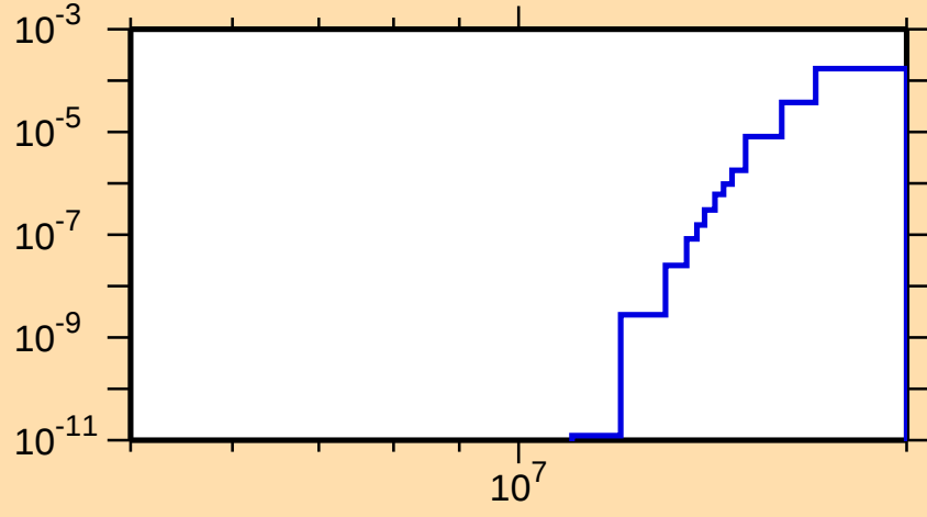
\sigma vs. E for ^{215}\text{Tl}(n,np)
