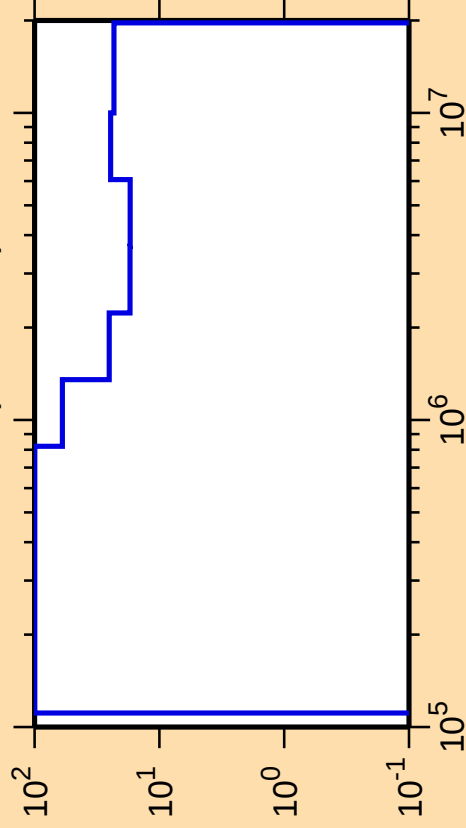
\Delta\sigma/\sigma vs. E for ^{215}\text{Tl}(n,\text{ncont.})
