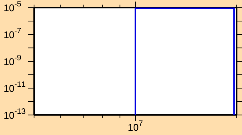
\sigma vs. E for ^{215}\text{Tl}(n,d)
