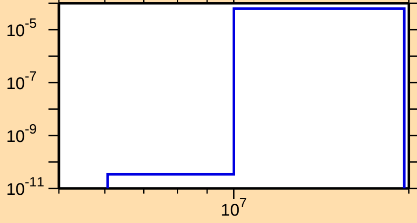
\sigma vs. E for ^{215}\text{Tl}(n,p)
