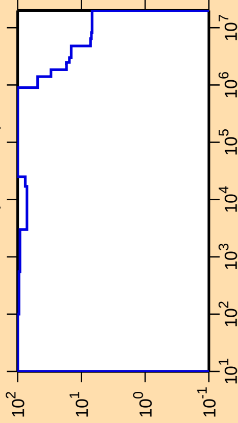
\Delta\sigma/\sigma vs. E for ^{215}\text{Tl}(n,\text{nonel.})
