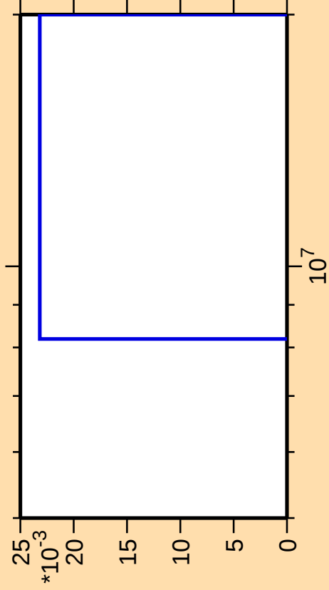
\Delta\sigma/\sigma vs. E for ^{215}\text{Tl}(\text{mt } 42)
