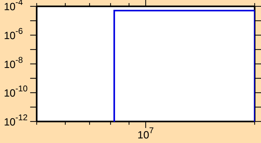
\sigma vs. E for ^{215}\text{Tl}(n,p)
