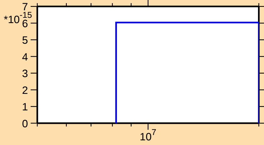
\sigma vs. E for ^{215}\text{Tl}(\text{mt } 42)
