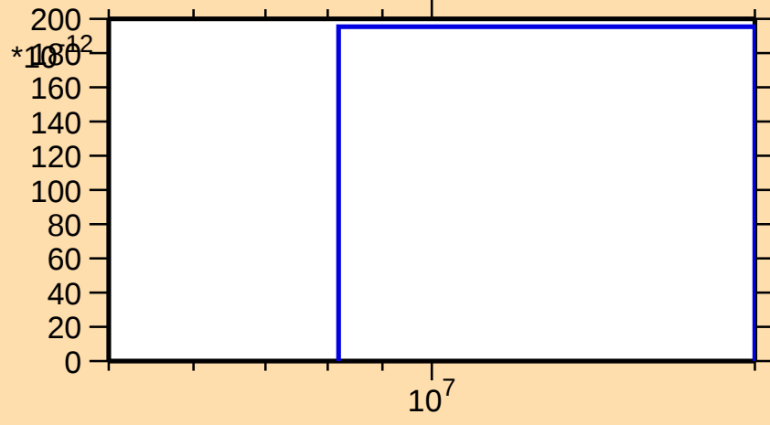
\sigma vs. E for ^{215}\text{Tl}(n,2n\alpha)
