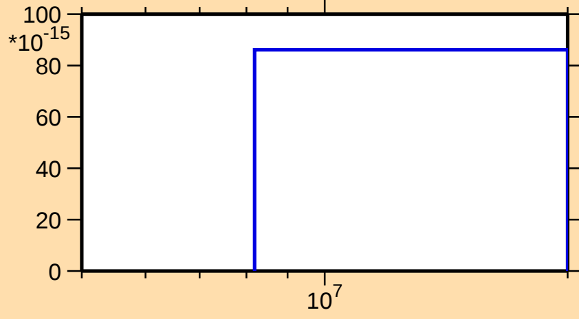
\sigma vs. E for ^{215}\text{Tl}(n,3n\alpha)
