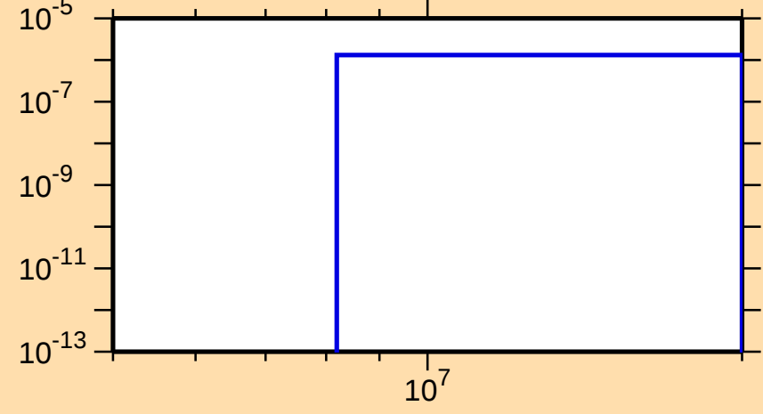
\sigma vs. E for ^{215}\text{Tl}(n,\text{nt})
