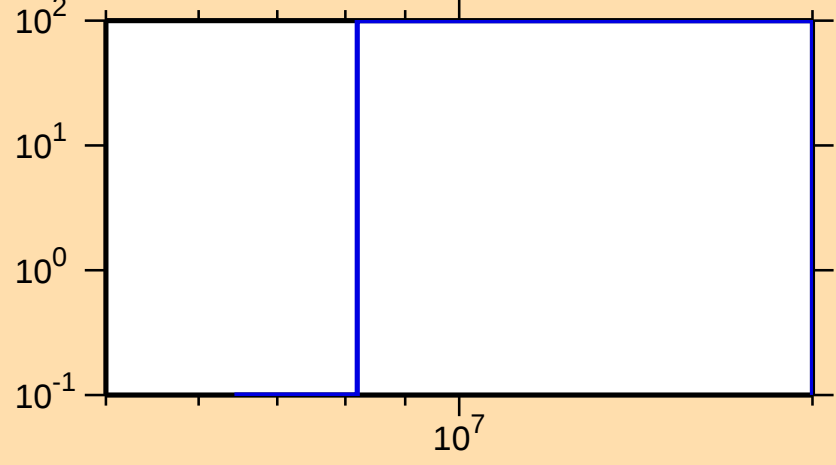
\Delta\sigma/\sigma vs. E for ^{215}\text{Tl}(n,p)
