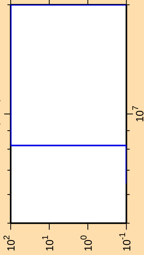
\Delta\sigma/\sigma vs. E for ^{215}\text{Tl}(n,\text{nt})
