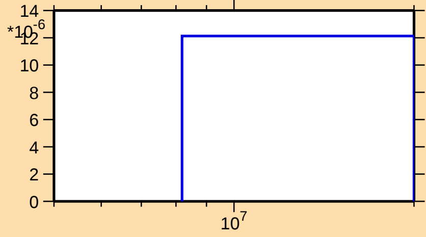
\sigma vs. E for ^{215}\text{Tl}(n,t)
