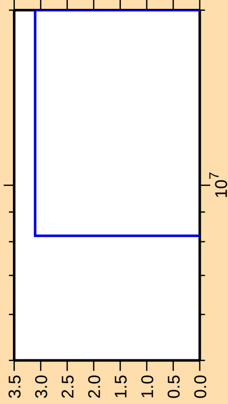
\Delta\sigma/\sigma vs. E for ^{215}\text{Tl}(\text{mt 11})
