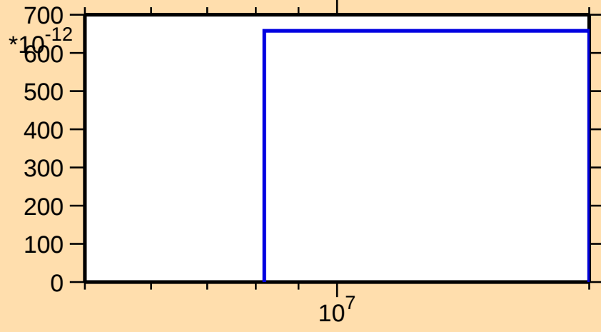
\sigma vs. E for ^{215}\text{Tl}(n,2np)
