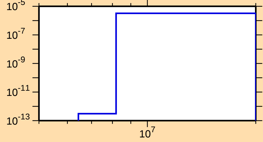
\sigma vs. E for ^{215}\text{Tl}(n,\alpha)
