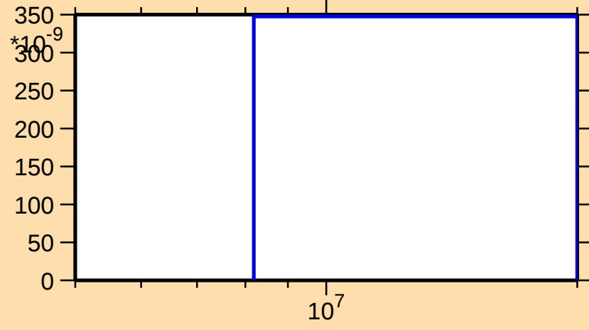
\sigma vs. E for ^{215}\text{Tl}(n,\alpha)
