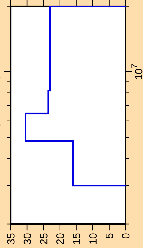
\Delta\sigma/\sigma vs. E for ^{215}\text{Tl}(n,n\text{cont.})
