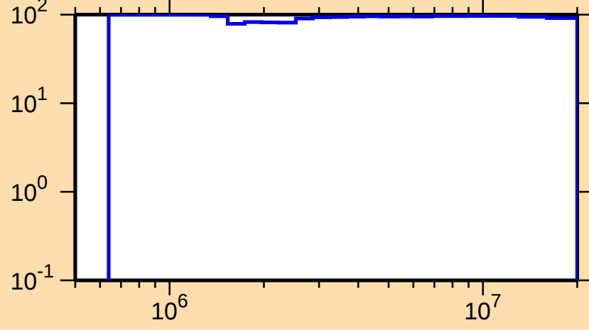
\Delta\sigma/\sigma vs. E for ^{166}\text{W}(n,ncont.)
