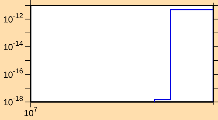
\sigma vs. E for ^{166}\text{W}(n,nt)
