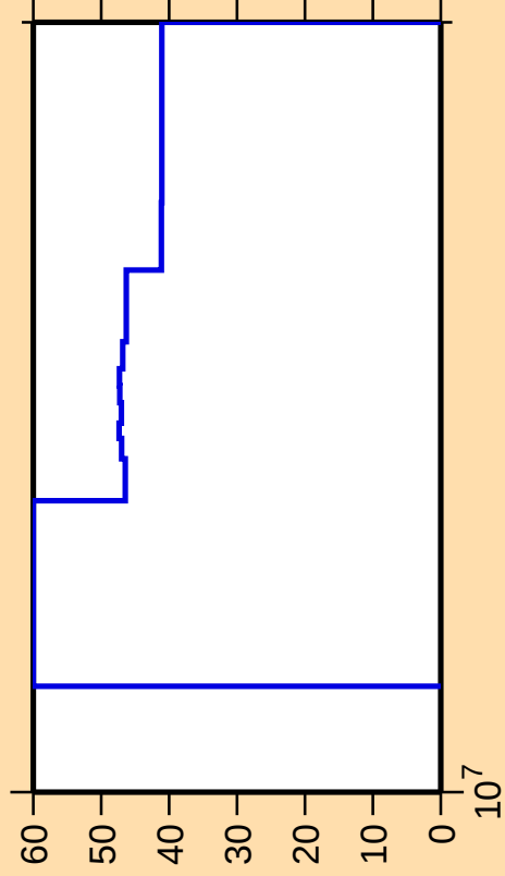
\Delta\sigma/\sigma vs. E for ^{166}\text{W}(n,n_1)
