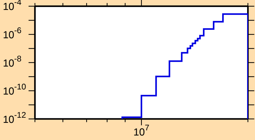
\sigma vs. E for ^{166}\text{W}(\text{mt } 45)
