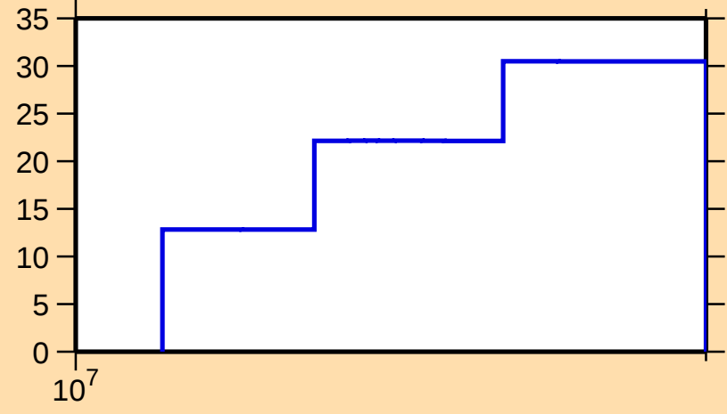
\Delta\sigma/\sigma vs. E for ^{166}\text{W}(n,\text{tot.})
