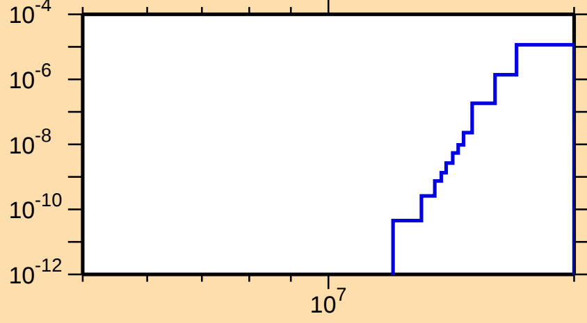
\sigma vs. E for ^{166}\text{W}(n,2n\alpha)
