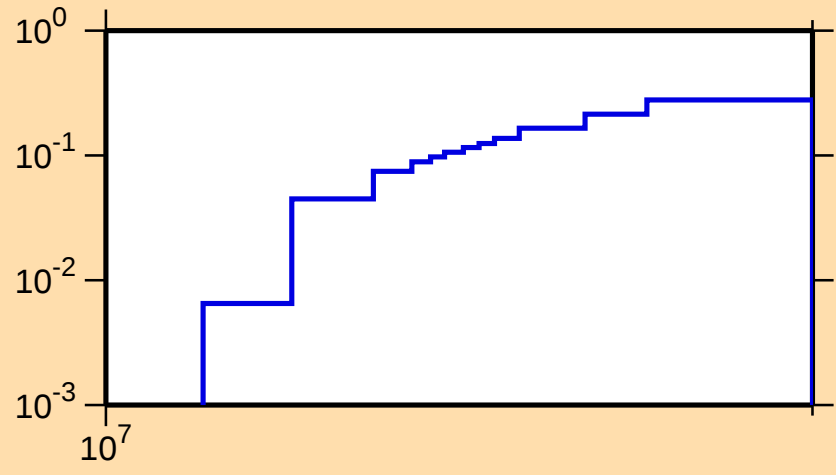
\sigma vs. E for ^{166}\text{W}(n,2n)
