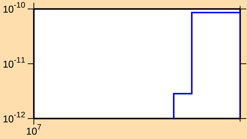
\sigma vs. E for ^{166}\text{W} (mt 34)
