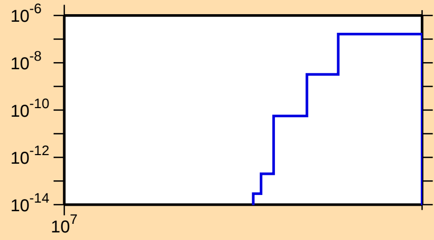
\sigma vs. E for ^{166}\text{W}(n,\text{nd})
