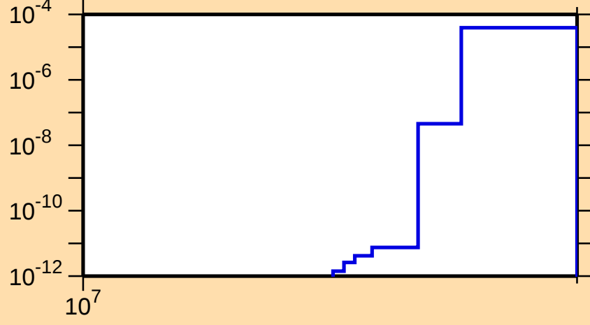
\sigma vs. E for ^{166}\text{W}(n,2np)
