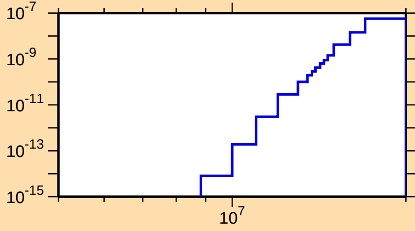
\sigma vs. E for ^{166}\text{W}(\text{mt117})
