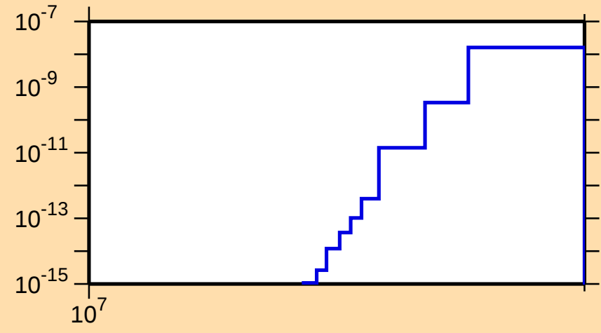
\sigma vs. E for ^{166}\text{W}(n,\text{pt})
