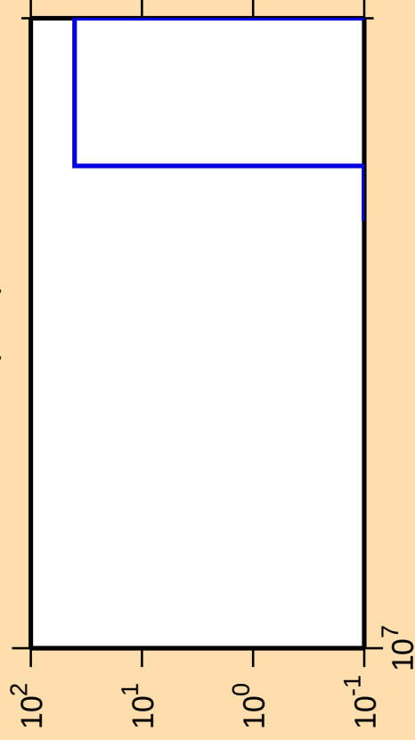
\Delta\sigma/\sigma vs. E for ^{166}\text{W}(n,nt)
