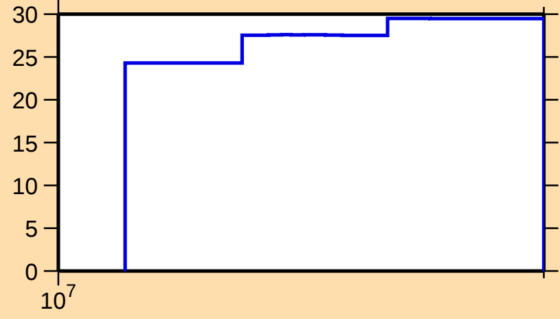
\Delta\sigma/\sigma vs. E for ^{166}\text{W}(n,\text{nonel.})
