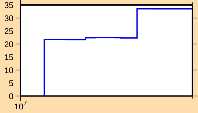
\Delta\sigma/\sigma vs. E for ^{166}\text{W}(n,\text{el.})
