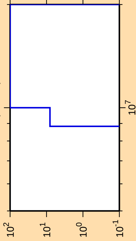
\Delta\sigma/\sigma vs. E for ^{166}\text{W}(\text{mt } 45)
