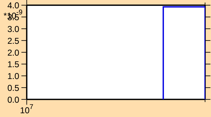
\sigma vs. E for ^{166}\text{W}(n,3n)
