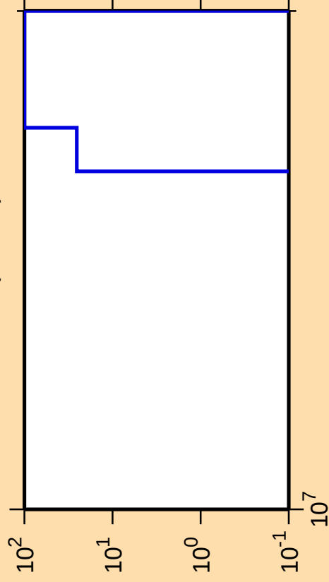
\Delta\sigma/\sigma vs. E for ^{166}\text{W} (mt 34)
